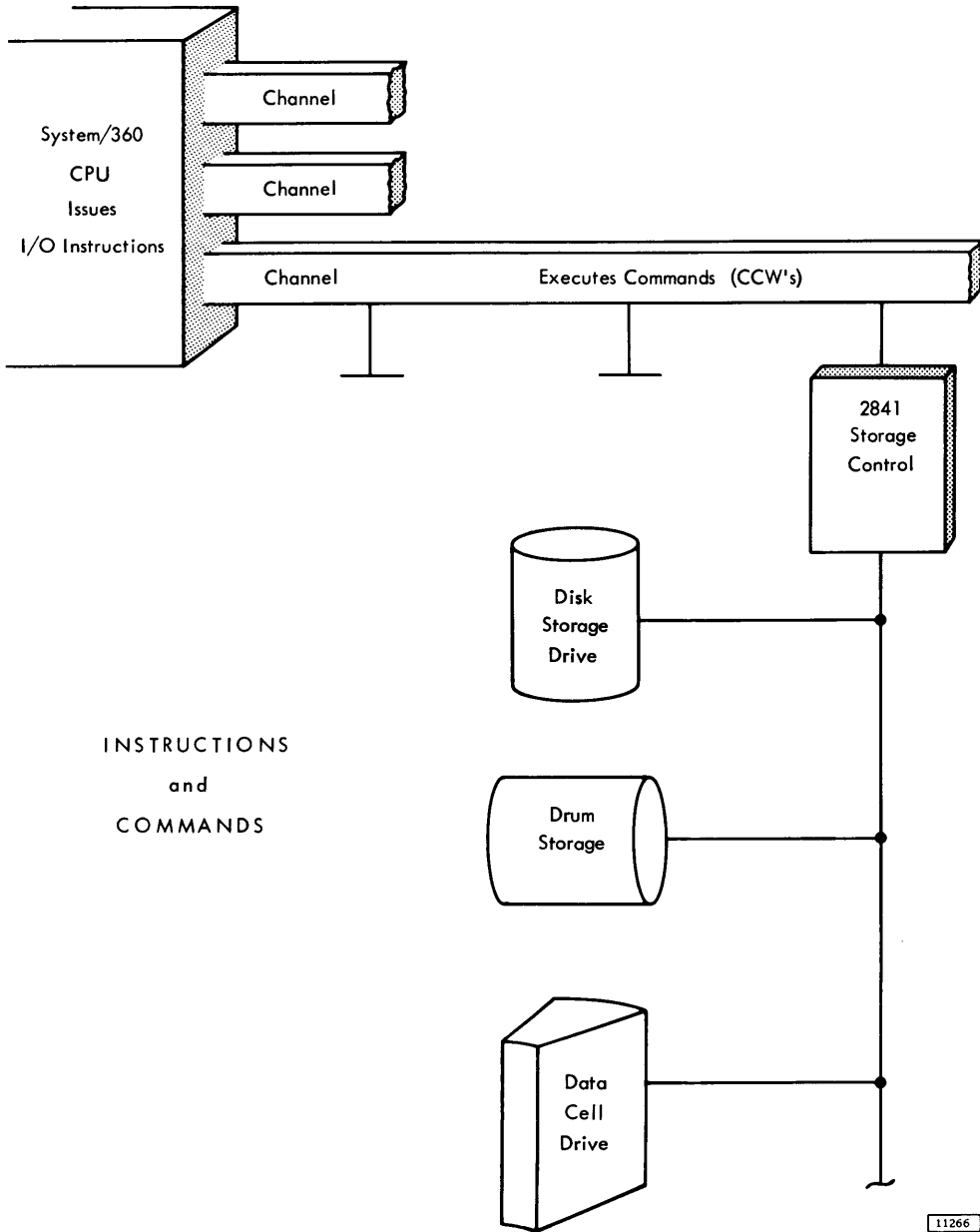
Figure 3. Instructions, Commands and Orders
