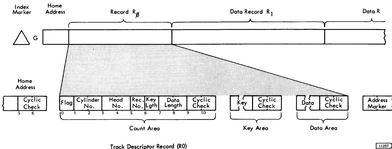
Figure 1. Track Descriptor Record
