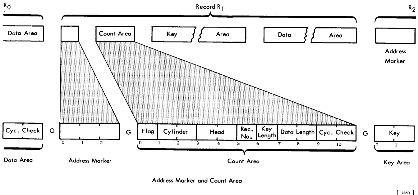
Figure 2. Address Marker and Count Area
