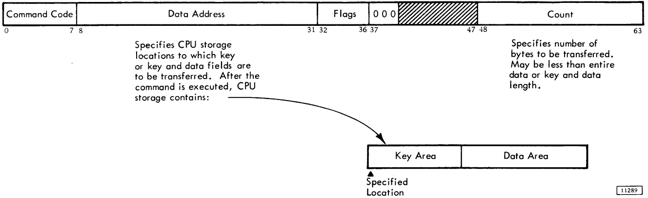
Figure 7. Read Data and Key and Data
