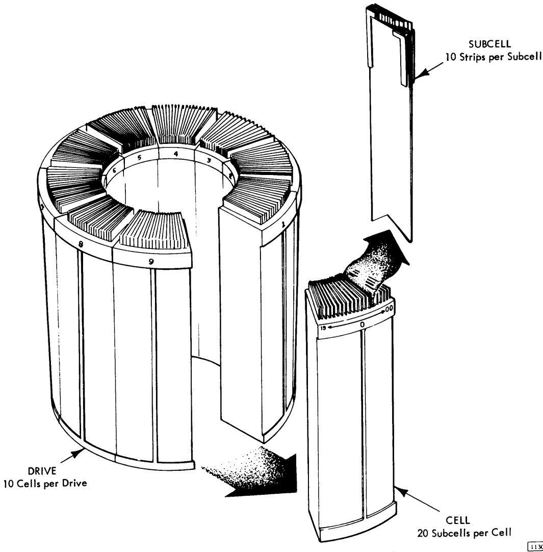
Figure 18. 2321 Drive, Cell, Subcell
