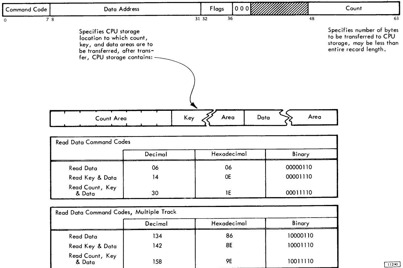
Figure 8. Read Count, Key, and Data
