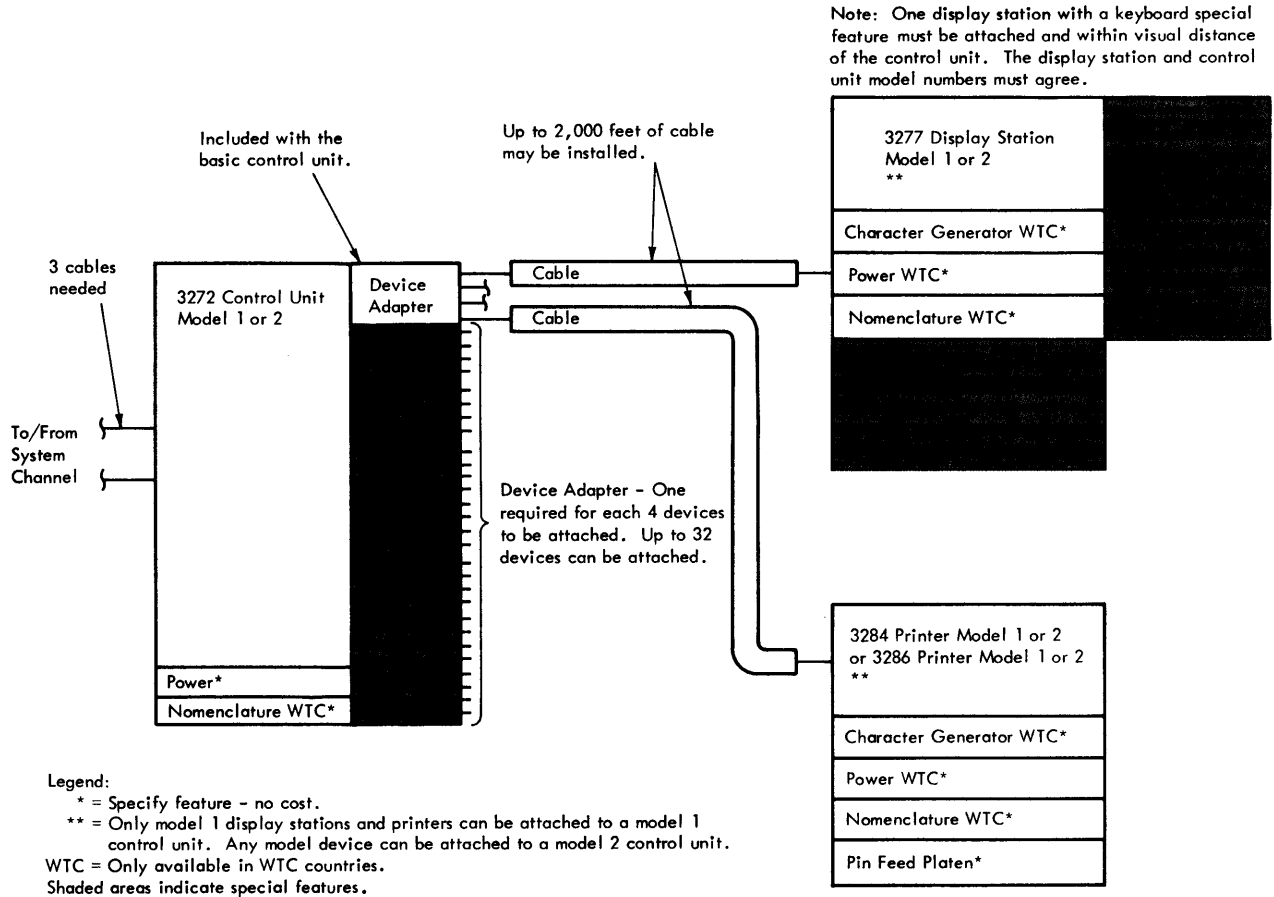
Figure A-1. 3270 Display System - Local
