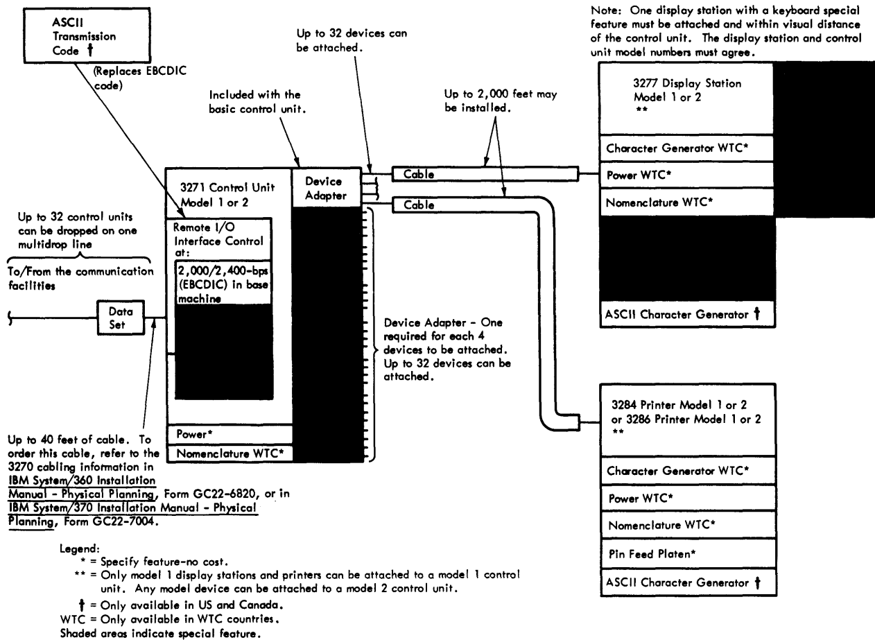
Figure A-2. 3270 Display System - Remote
