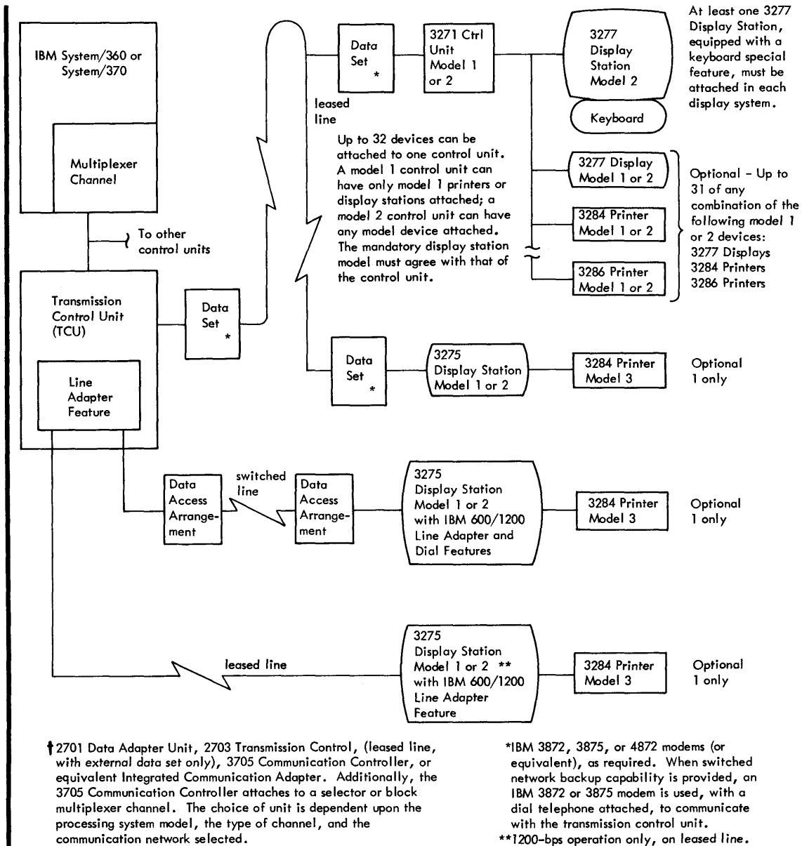
Figure 2-2. Remotely Attached 3270 Display System
