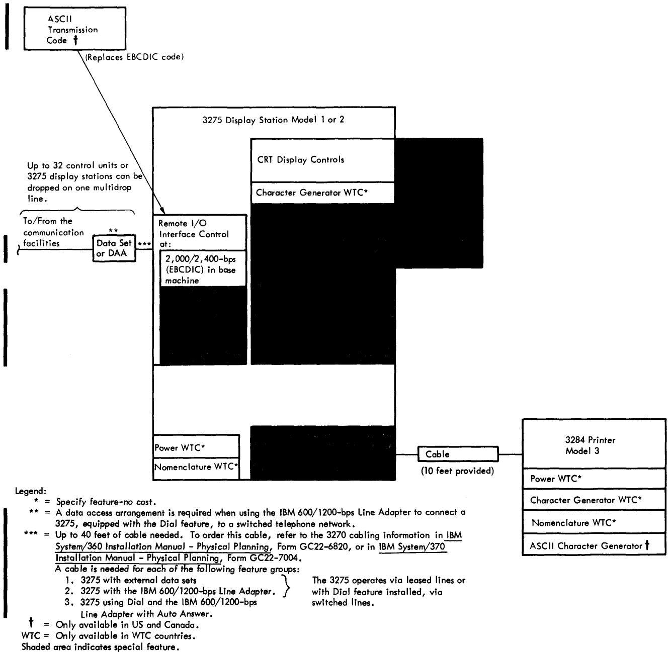
Figure A-3. 3275 Display Station
