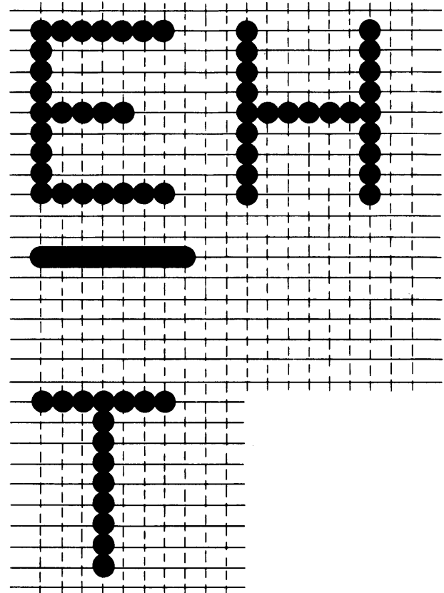
Figure 7-1. Examples of Monospace Characters Formed with 7 x 9 Dot Pattern
