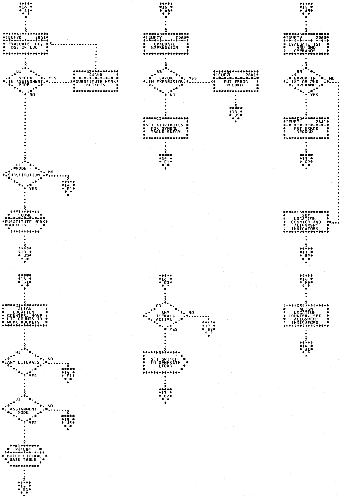
Chart 16. IEUF7C - Phase F7 Main Line Control (4 of 6)
