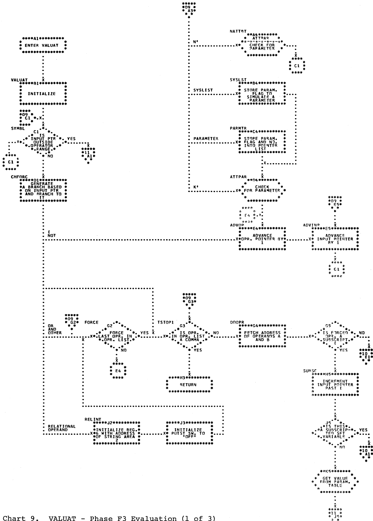
Chart 9. VALUAT - Phase F3 Evaluation (1 of 3)
