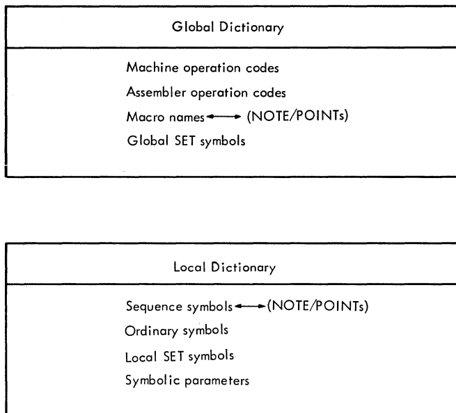
Figure 4. Dictionary Structure
