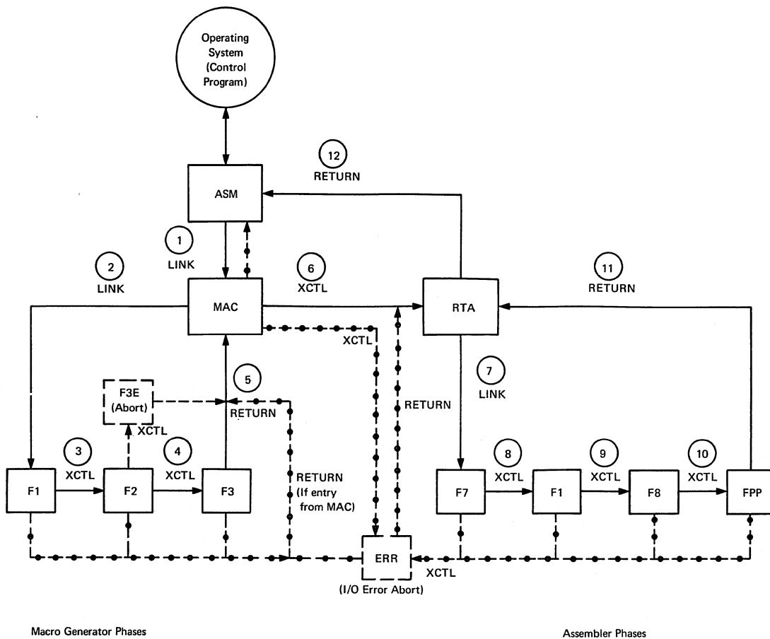
Figure 3. Program Flow
