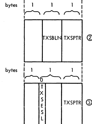
Figure 10. Types 1 and 2 Work Buckets
