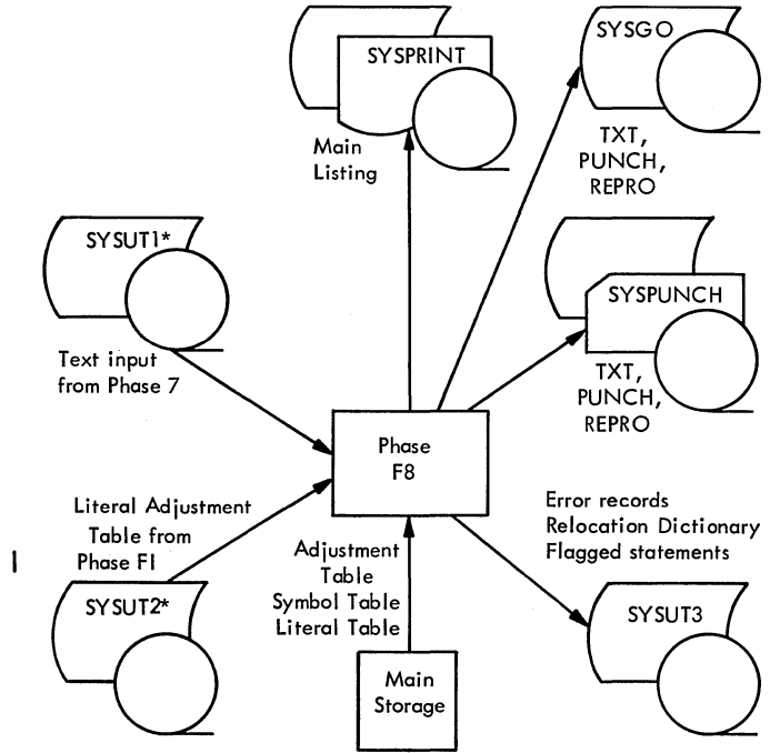
Figure 13. I/O Flow for Phase F8
