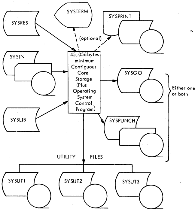
Figure 2. Data Sets Used by the Assembler
