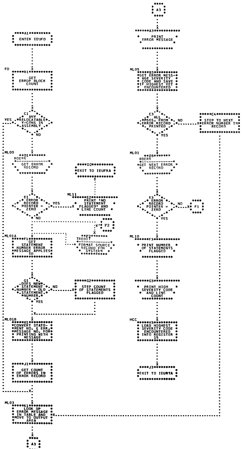
• Chart 38. IEUFD - Phase FPP Diagnostic
