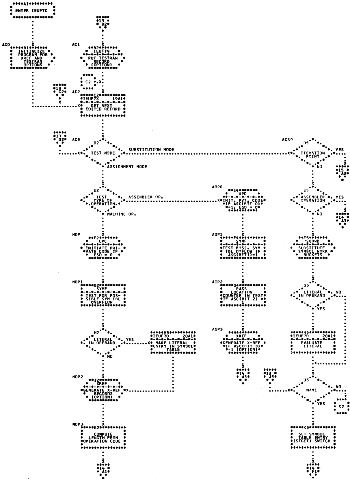
Chart 13. IEUF7C - Phase F7 Main Line Control (1 of 6)
