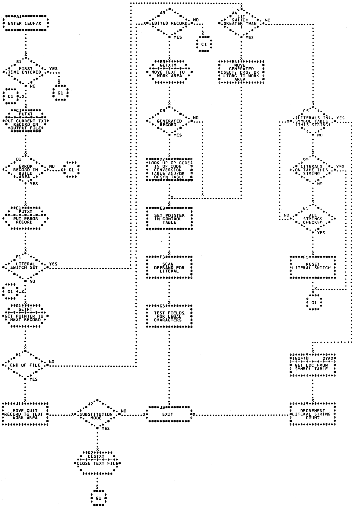
Chart 19. IEUF7X - Phase F7 Get Statement
