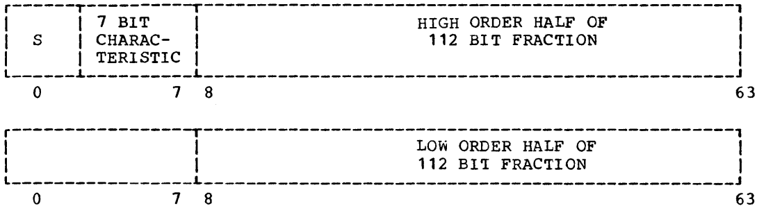
Figure 12. Floating-Point External Formats
