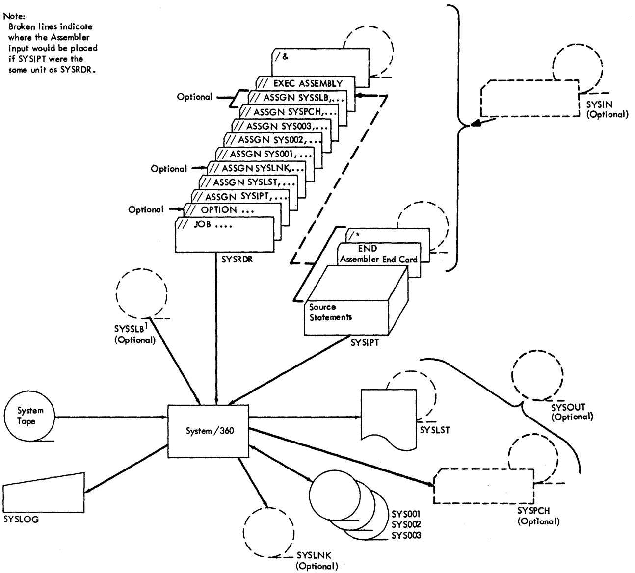
Figure 26. I/O Units Used by the Tape Assembler
