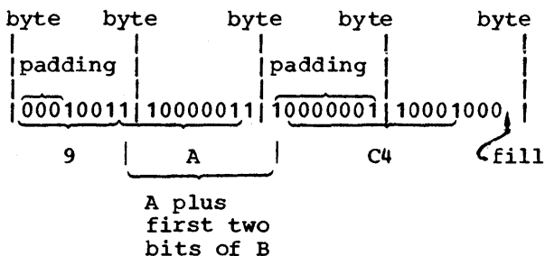
Figure 11. Bit-Length Specification (Multiple Operands)
