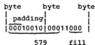
Figure 9. Bit-Length Specification (Single Constant)
