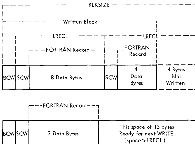
Figure 41. Variable-Length Blocked Records Written Under FORMAT Control
