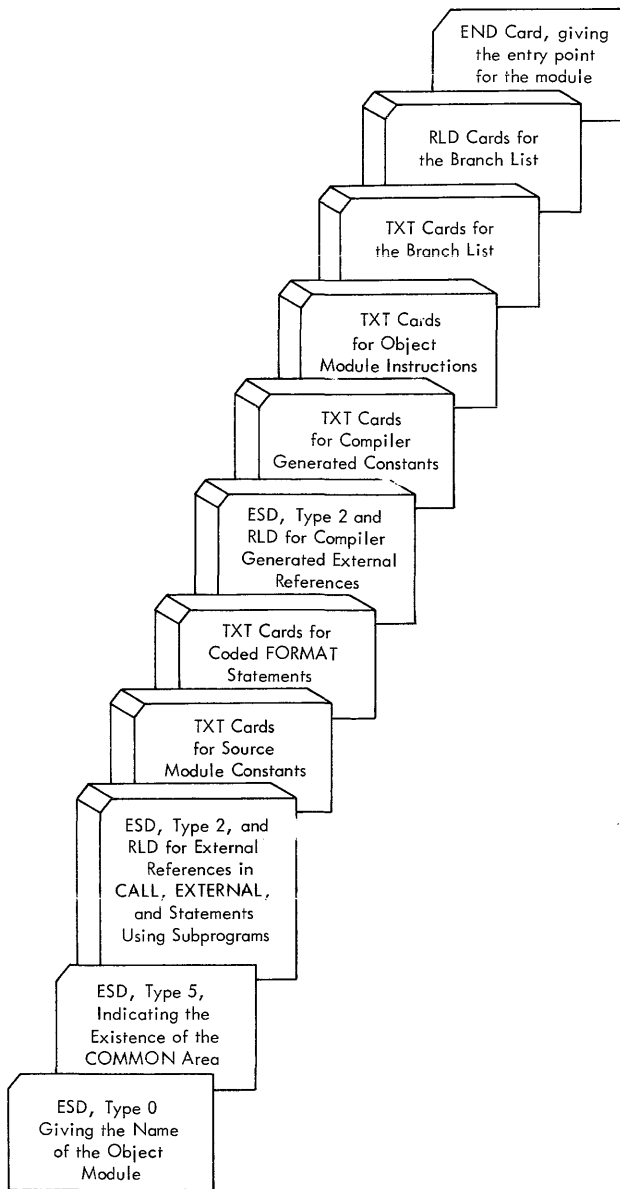
Figure 57. Object Module Deck Structure
