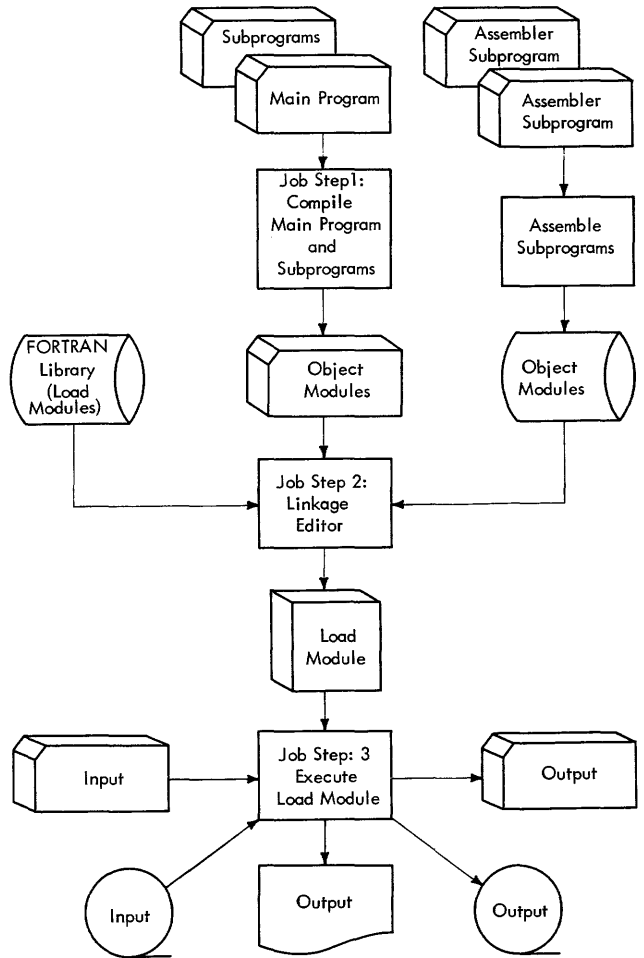
Figure 3. Typical FORTRAN Processing
