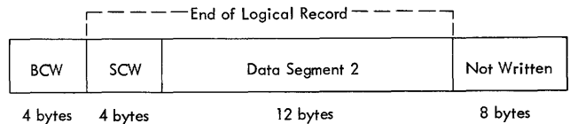
Figure 45. Variable-length Unblocked Records, No FORMAT Control, Two Record Segments
