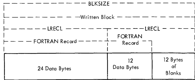
Figure 40. Fixed-Length Blocked Records Written Under FORMAT Control
