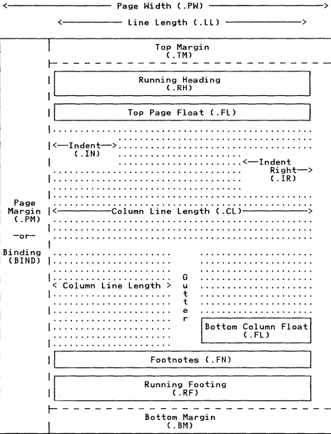
SCRIPT/VS Terms for Parts of the Page.
