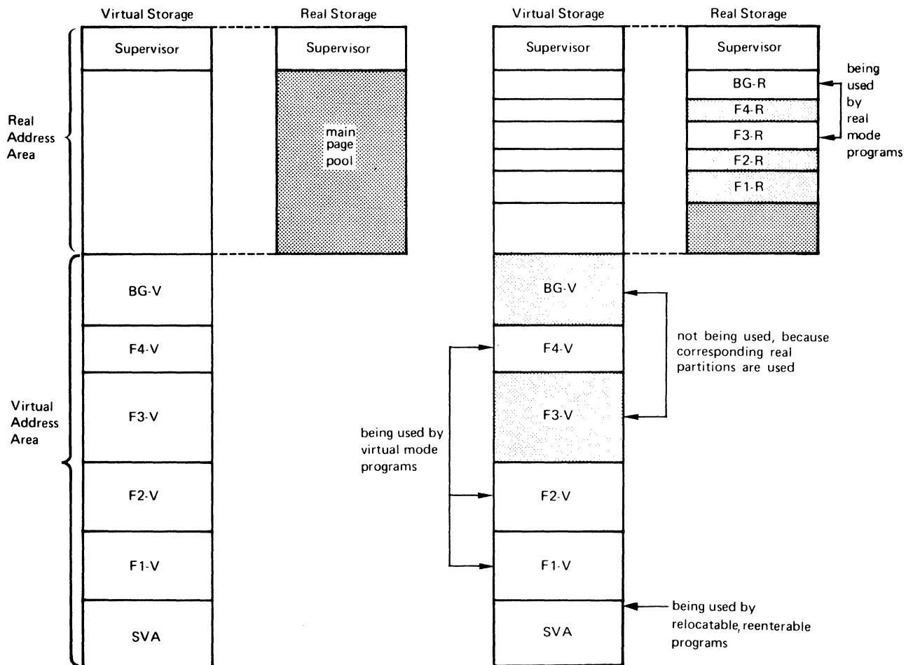
Figure 1.5. A System With and Without Real Partitions
