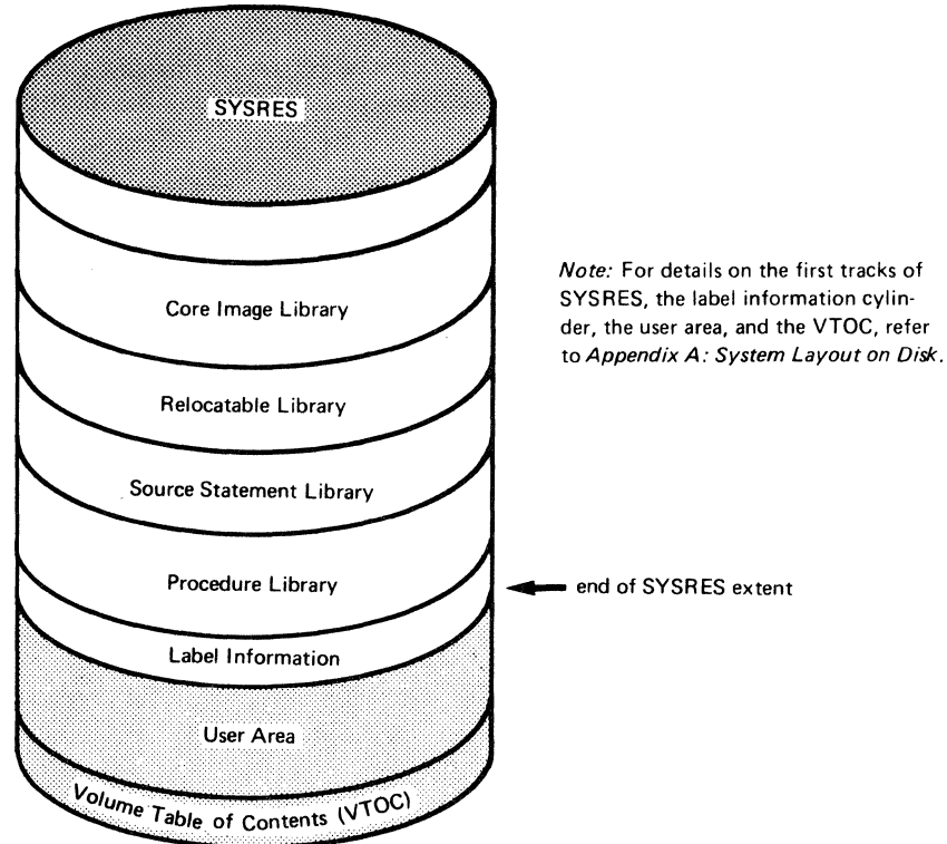
Figure 3.10. The Relative Location of the Four System Libraries
