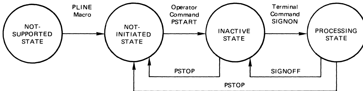
Figure 8.3. Transition between RJE Line States
