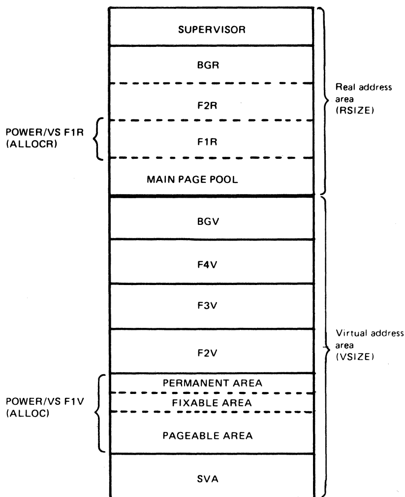
Figure 3.8 POWER/VS Partition Allocations
