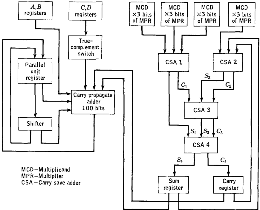
FIG. 14.7. Parallel arithmetic unit.
