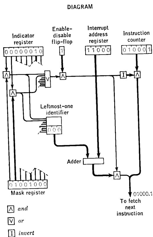
FIG. 10.3. Program-interrupt example. One-instruction fix-up.
