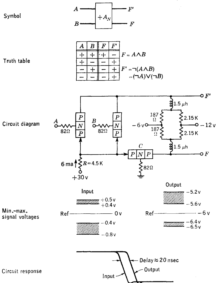
FIG. 14.16. Current-switching circuit, PNP. Symbols: \wedge and , \vee or , \neg not .
