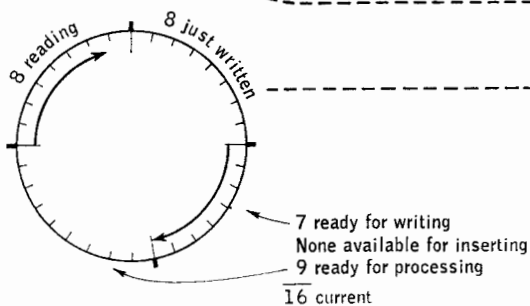
FIG. 11.10. Control-word diagram for file maintenance.
