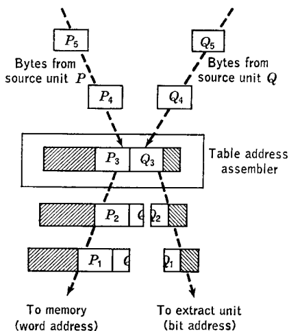
FIG. 17.5. Formation of look-up address.
