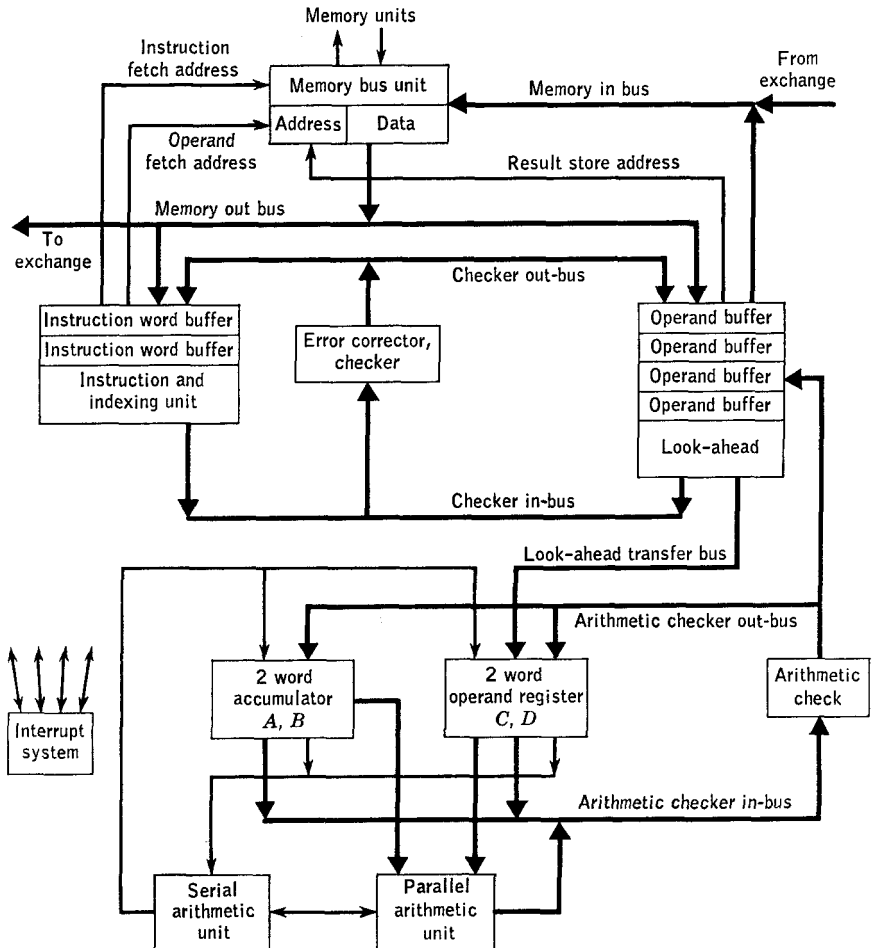
FIG. 14.4. Computer units and bus system.
