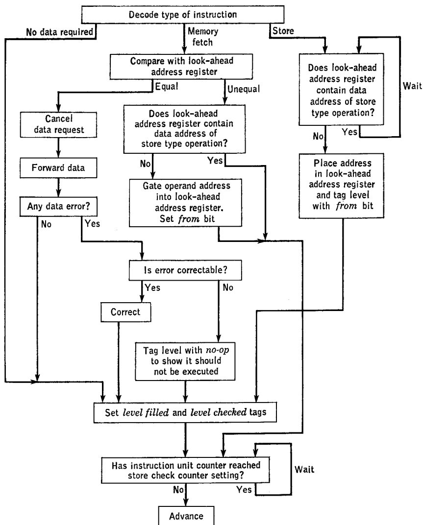
FIG. 15.7. Instruction-unit counter advance sequence.
