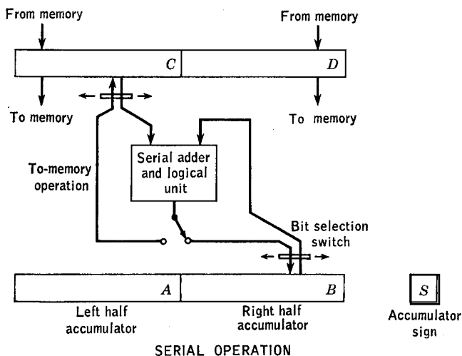
FIG. 3.2. Simplified register structure of arithmetic unit.
