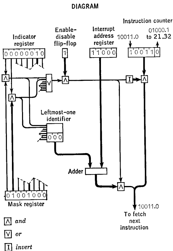
FIG. 10.4. Program-interrupt example. Interrupt subroutine with further interrupts inhibited.
