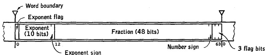
FIG. 4.1. Data unit for floating-point arithmetic.
