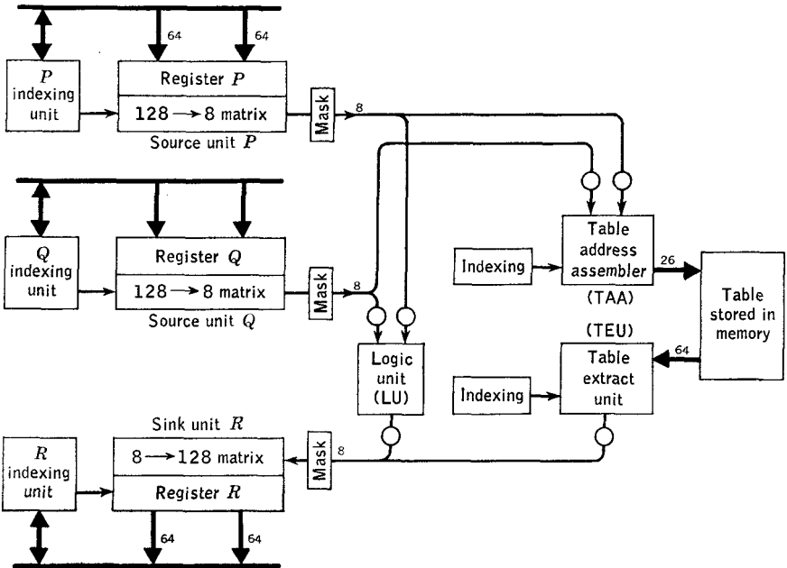
FIG. 17.4. Transformation facilities.
