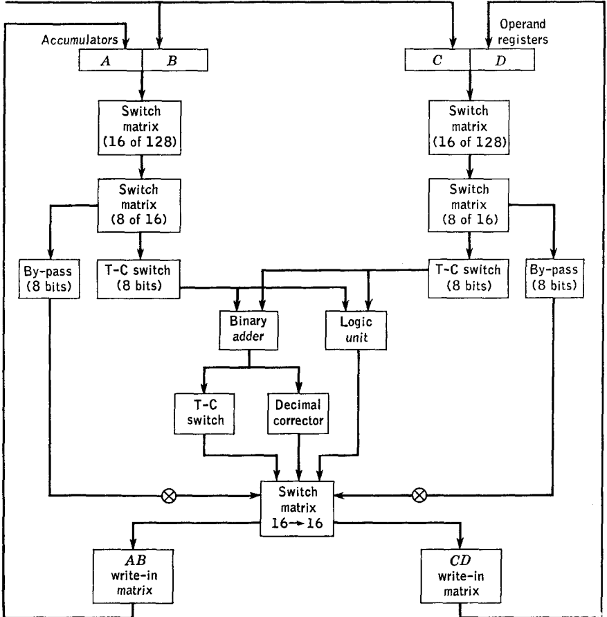
FIG. 14.6. Serial arithmetic unit. T-C: true-complement.
