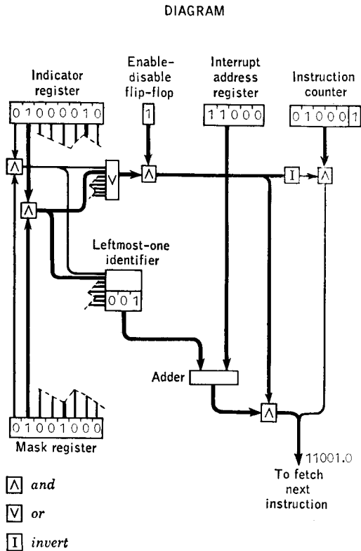
FIG.10.2. Program-interrupt example. Condition masked on: interrupt occurs.
