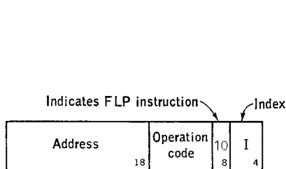
FIG. 8.1. FLP instruction format.
