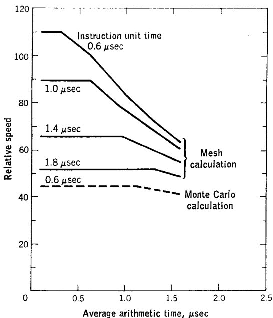
FIG. 15.3. Computer speed vs. arithmetic times for various instruction-unit times. Four levels of look-ahead; four units of 2.0- \mu sec memory; two units of 0.6- \mu sec memory.
