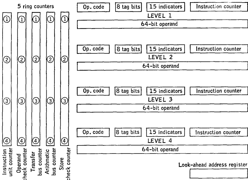
FIG. 15.6. Look-ahead registers.
