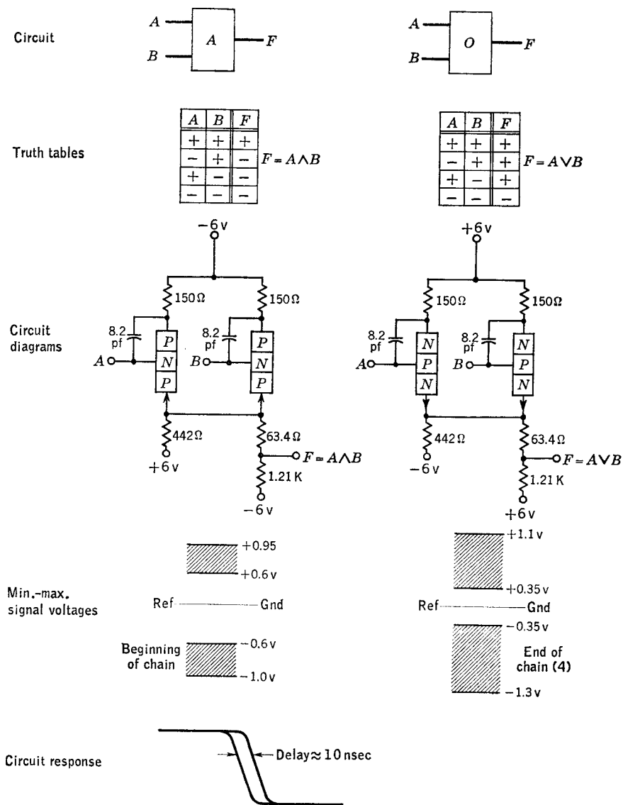
FIG. 14.19. Emitter-follower logic.
