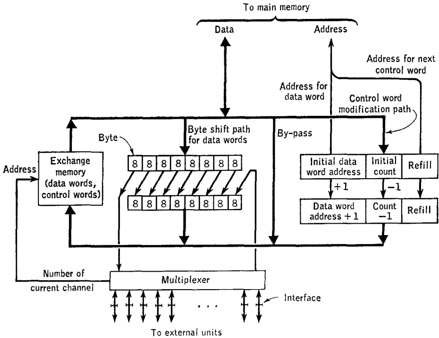
FIG. 16.1. Data-flow paths of exchange.
