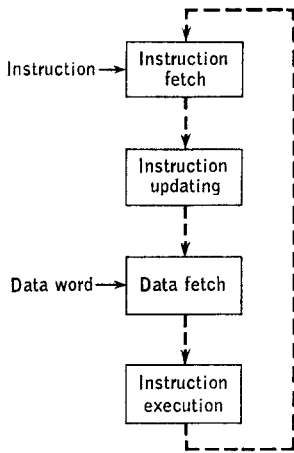
FIG. 14.2. Sequential operation.
