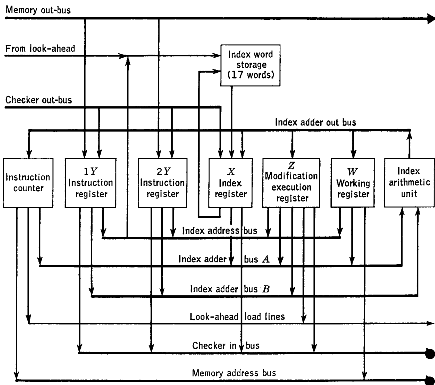
FIG. 14.5. Instruction unit.
