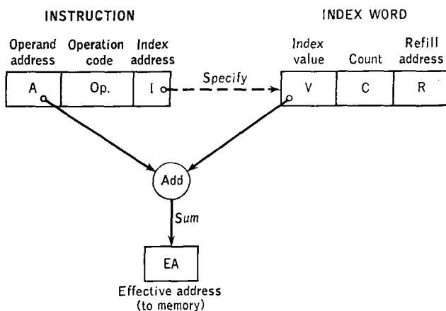
FIG. 11.4. Address modification.
