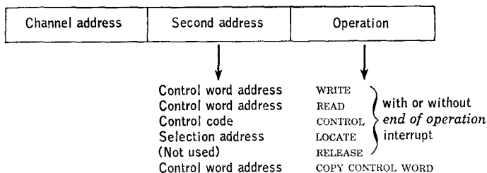
FIG. 12.1. Principal parts of input-output instructions.
