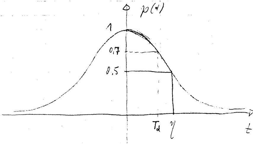
Fig. 4 Lorentzian readback pulse ( \eta - inflection point)
