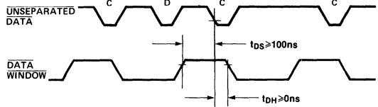
Figure 9. PLO Data Window Timing
