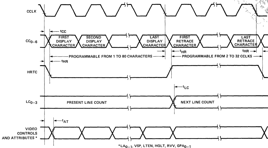
Figure 26. Line Timing
