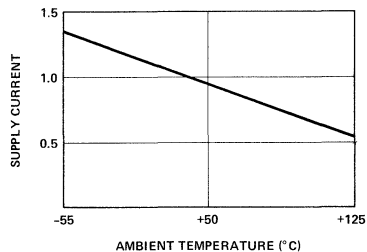
Figure 1. Typical Supply Current vs. Temperature, Normalized[3]
