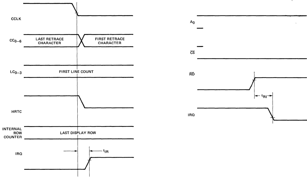
Figure 29. Interrupt Timing
