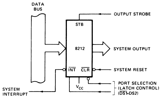
Figure 8. 8080 Status Latch
