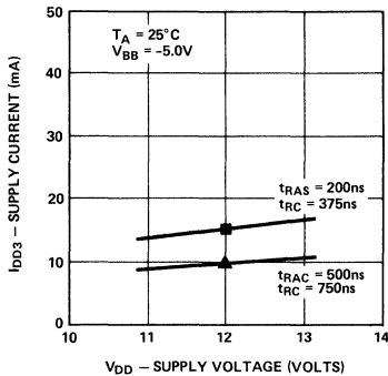
GRAPH 11 TYPICAL \overline{RAS} ONLY REFRESH CURRENT I_{DD3} VS. V_{DD}
