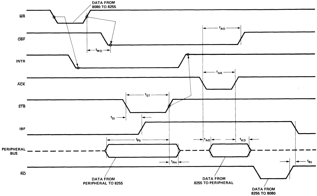
Figure 32. MODE 2 (Bidirectional)
