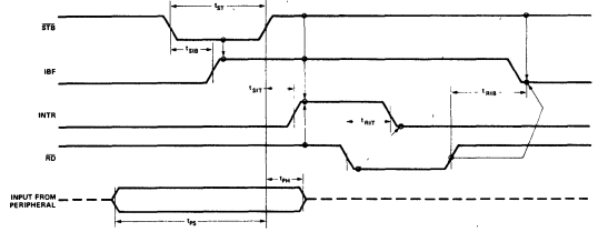
Figure 28. MODE 1 (Strobed Input)
