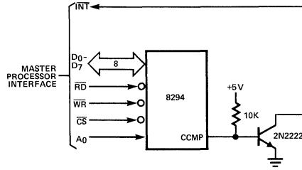
Figure 2. Single Interrupt Interface
