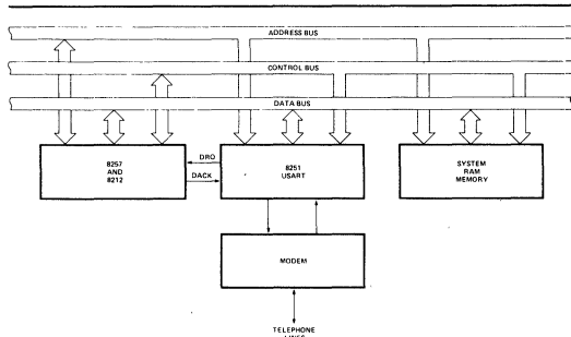
Figure 11. High-Speed Communication Controller
