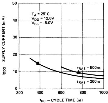
GRAPH 10 TYPICAL \overline{RAS} ONLY REFRESH CURRENT I_{DD3} VS. t_{RC}
