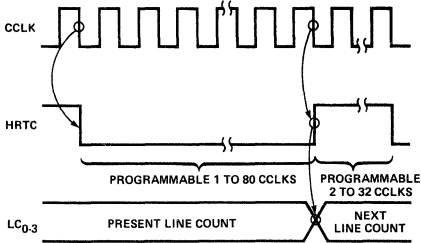
Figure 15. Line Timing
