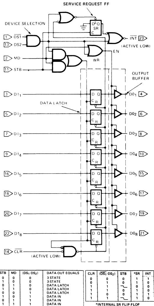
Figure 1. Service Flip-Flop Function
