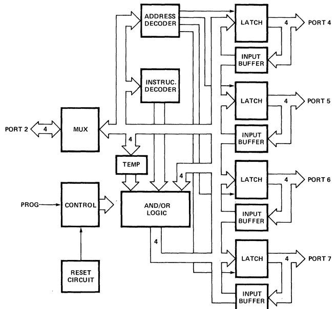
BLOCK DIAGRAM
