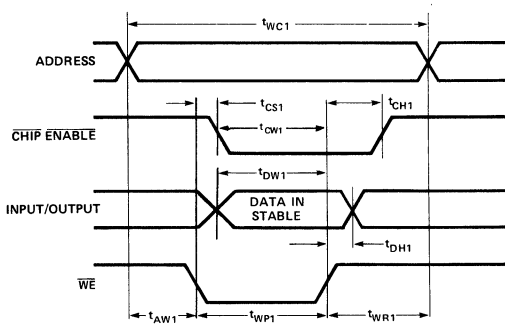
WRITE CYCLE #1
