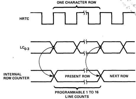
Figure 16. Row Timing
