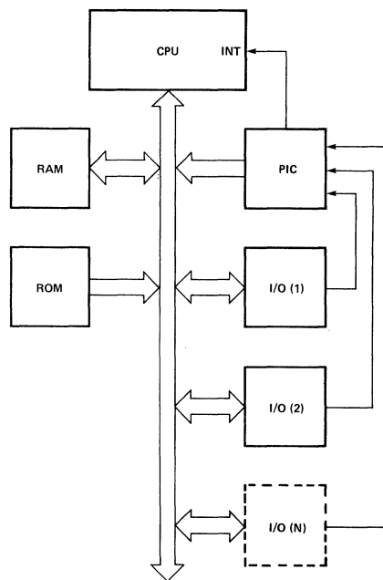
Figure 2. Interrupt Method
