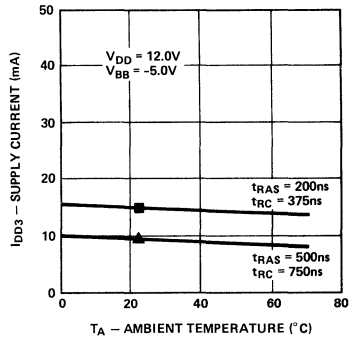
GRAPH 12 TYPICAL \overline{RAS} ONLY REFRESH CURRENT I_{DD3} VS. AMBIENT TEMPERATURE
