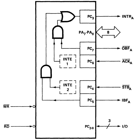
Figure 12. MODE 2
