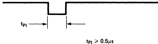
Figure 15. Index Timing
