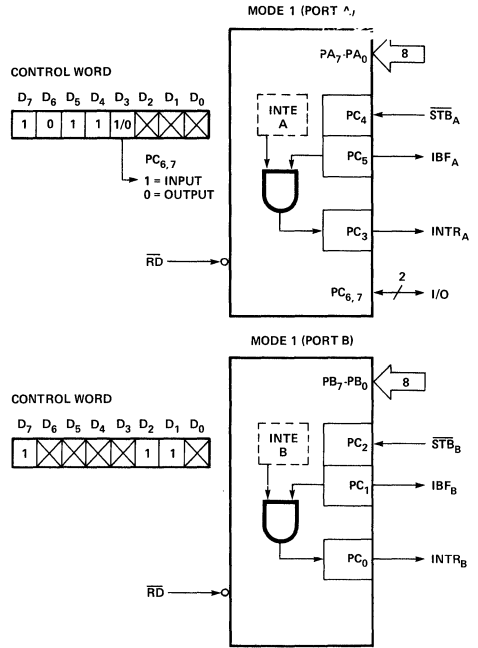
Figure 6. MODE 1 Input
