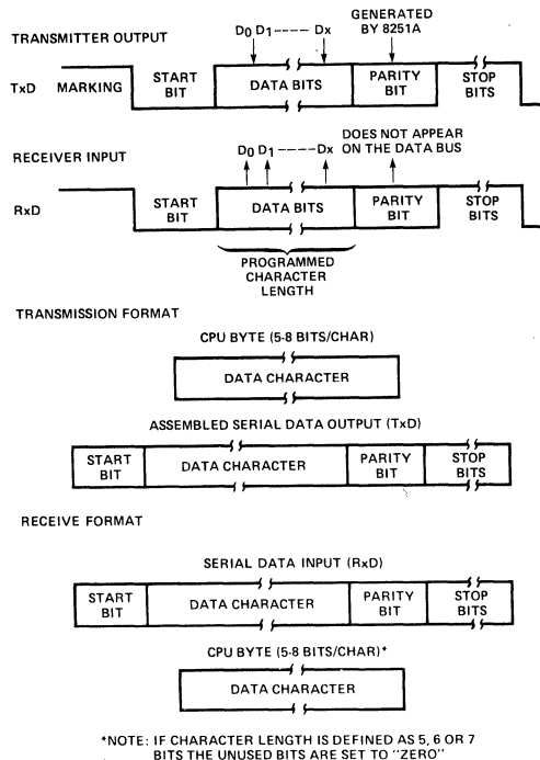
Figure 7. Asynchronous Mode
