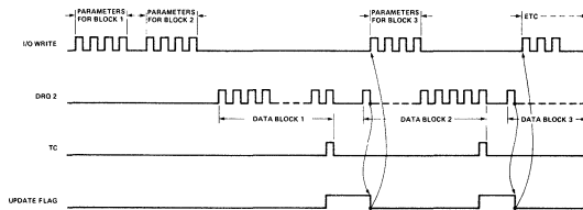
Figure 5. Autoload Timing
