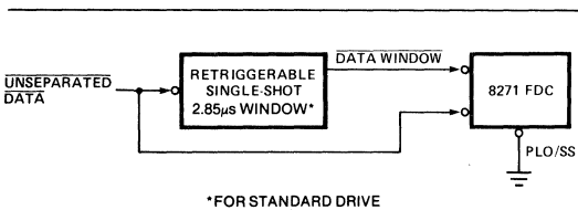
Figure 6. Single-Shot Data Separator Block Diagram
