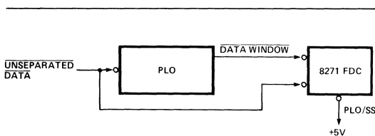
Figure 8. PLO Data Separator Block Diagram
