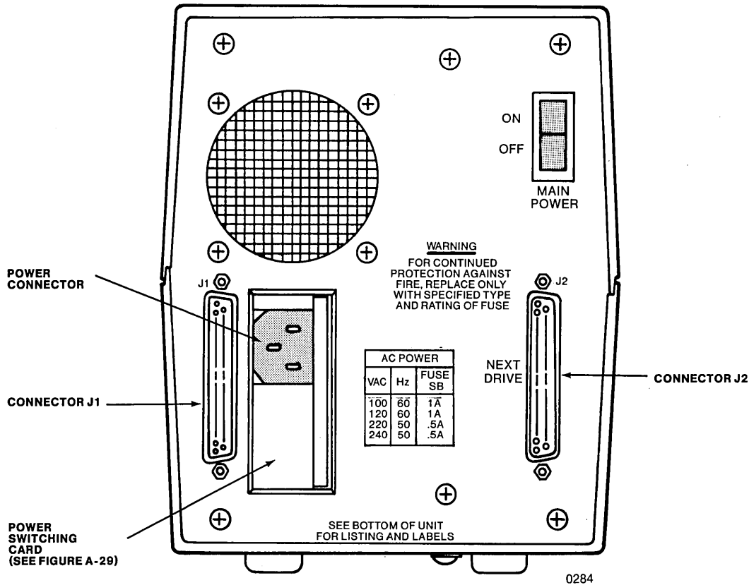
Figure A-30 Rear Panel of the iPDS™-130 Drive
