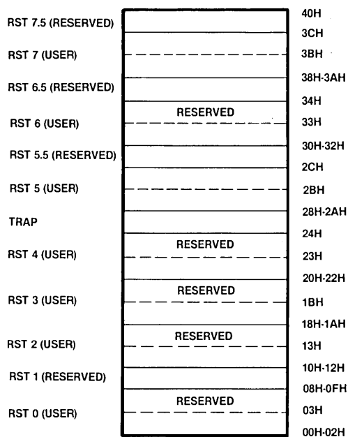
Figure 8-5 Interrupt Vectors
