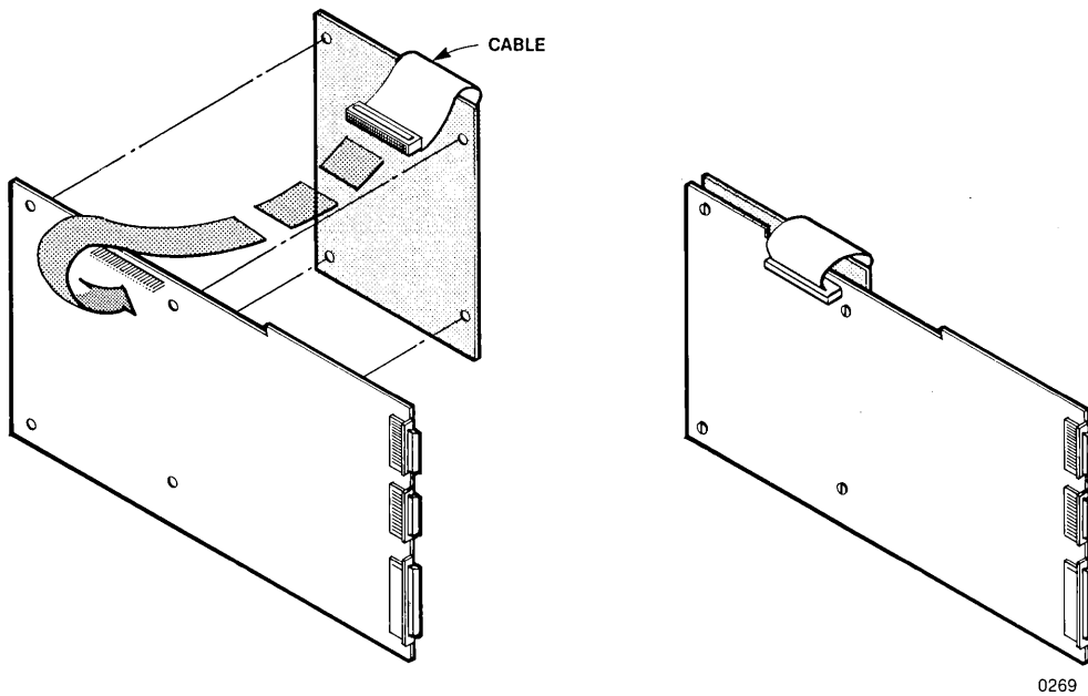
Figure A-15 Aligning the Optional Processor Board
