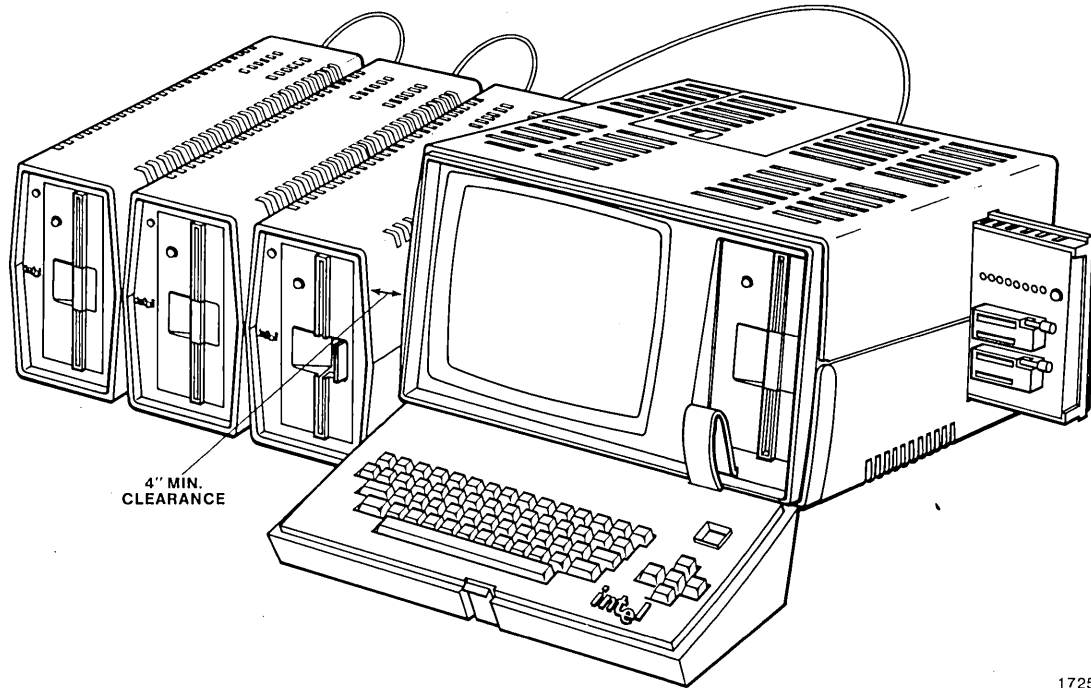
Figure 1-4 System with Options
