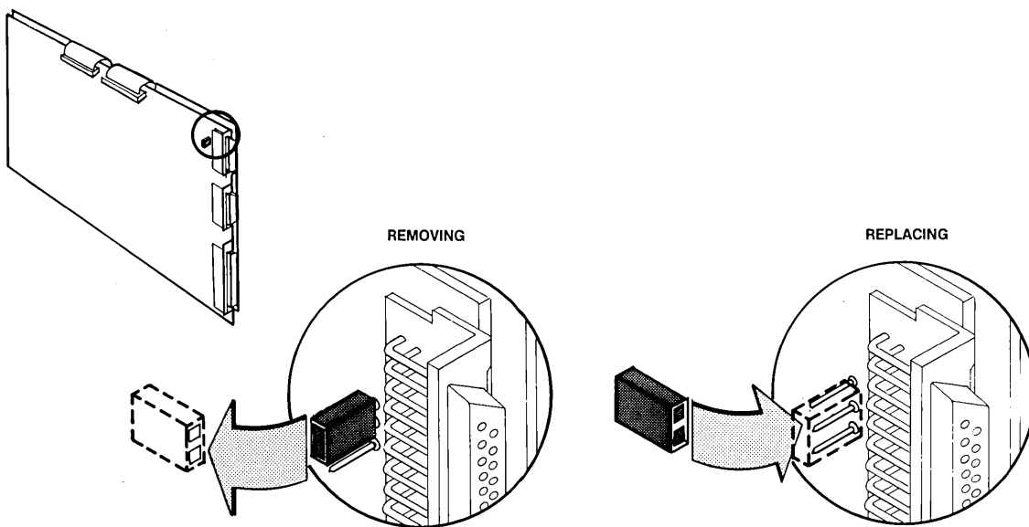
Figure A-12 Removing and Replacing the Plug-in Type Jumpers
