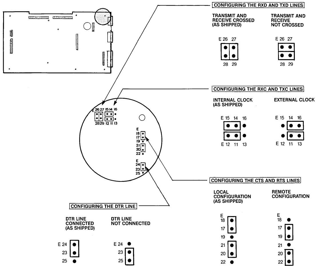
Figure A-11 Removable Jumper Location and Configuration
