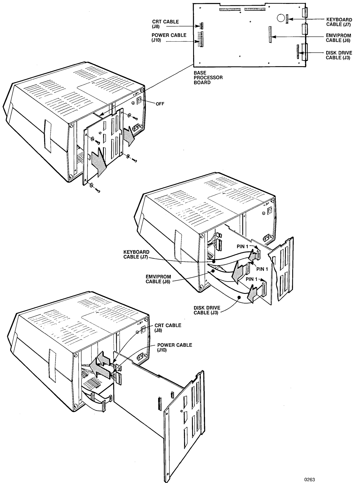
Figure A-7 Removing the I/O Panel
