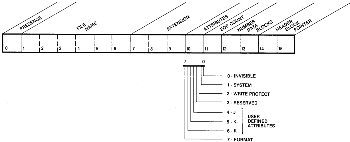
Figure 8-16 Directory Entry
