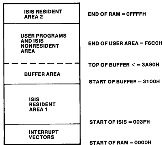
Figure 8-4 Memory Map
