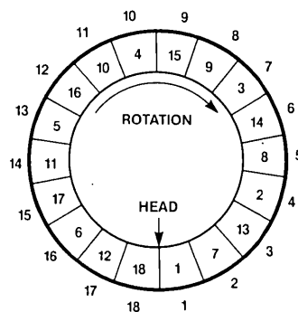
Figure 8-15 Sector Interleaving
