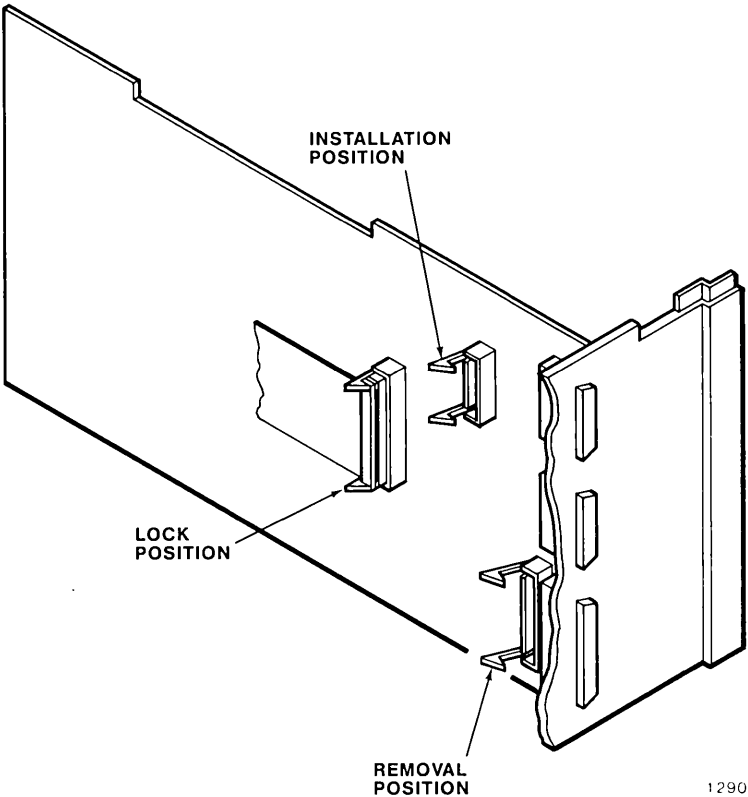
Figure A-8 Using the Connector Locks
