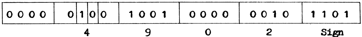
Figure 6-4. Packed Decimal Representation in the Computer.
