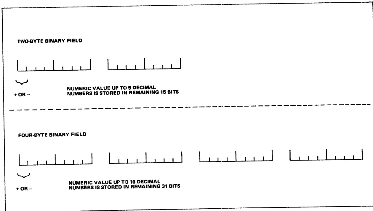
Figure 6-6. Binary Format.
