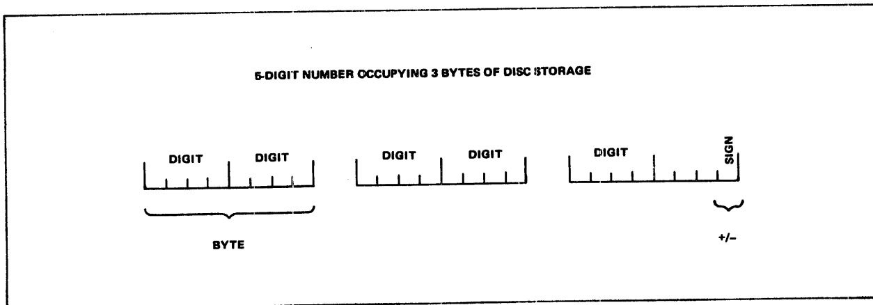
Figure 6-3. Packed Decimal Format.
