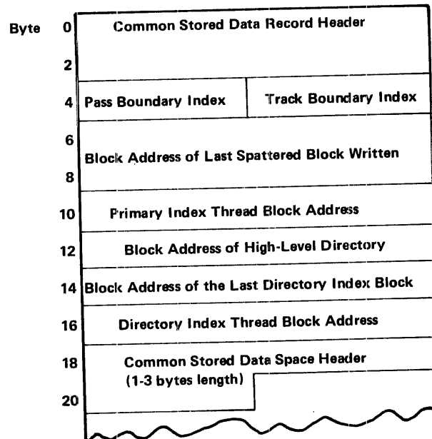
Figure J-2. Information Block
