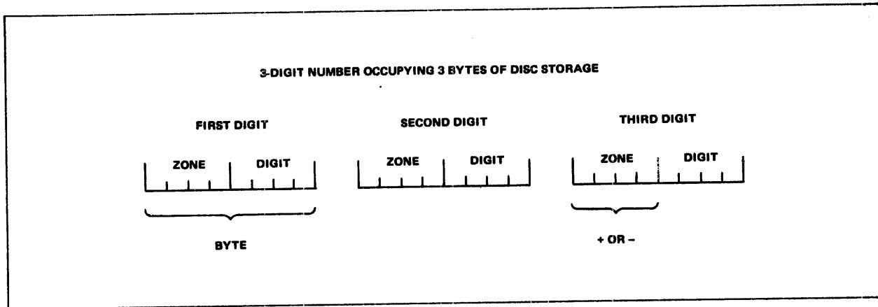
Figure 6-2. Unpacked Decimal Format.
