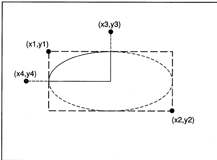
Figure 4.3 Bounding Rectangle
