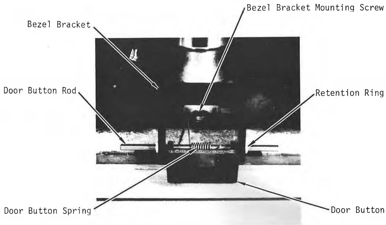
Figure 4-5. Door Button Assembly
