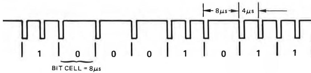
Figure 3-21: FM Encoding
