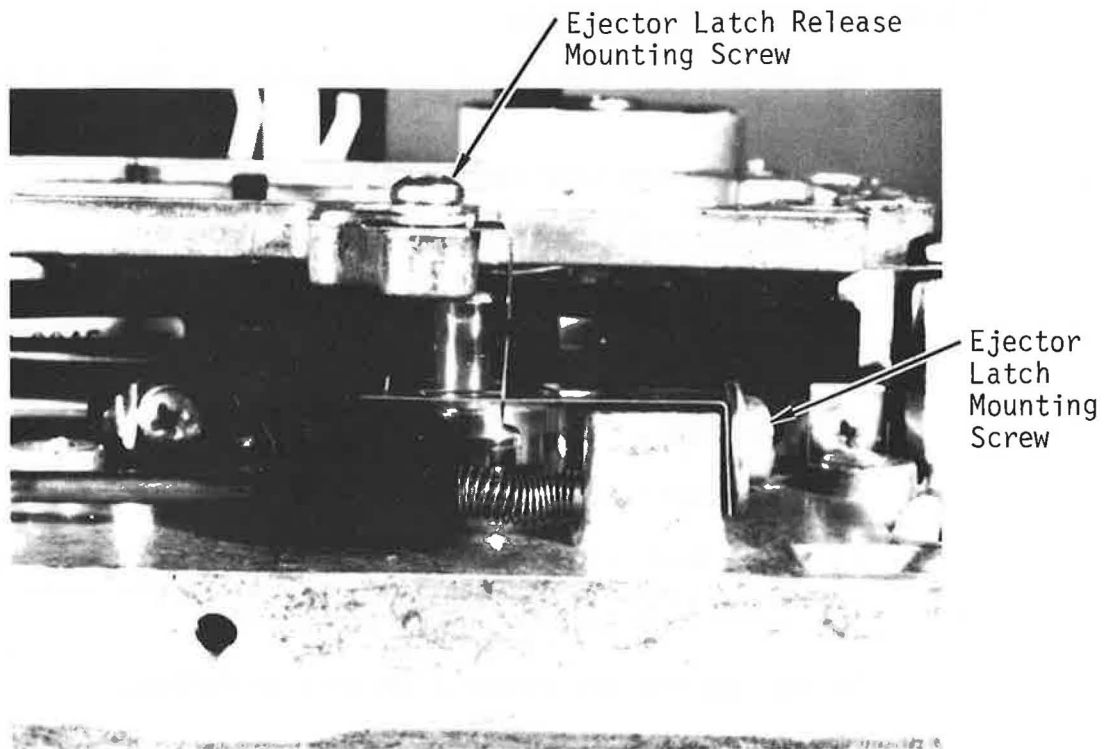
Figure 4-7 Ejector Assembly
