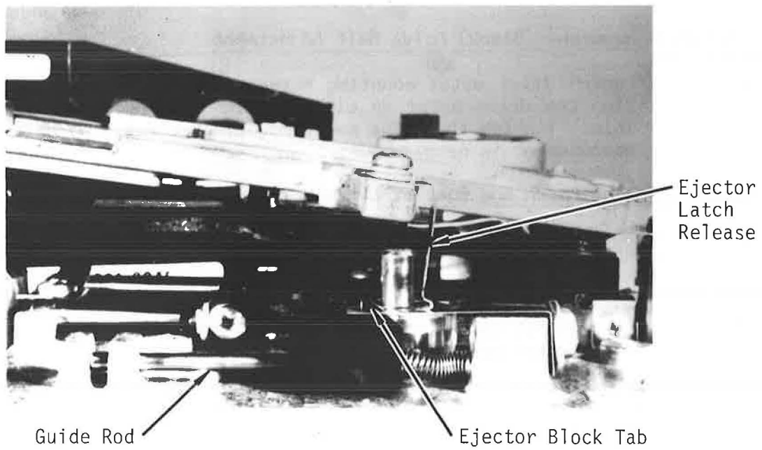
Figure 4-11: Ejector Assembly
