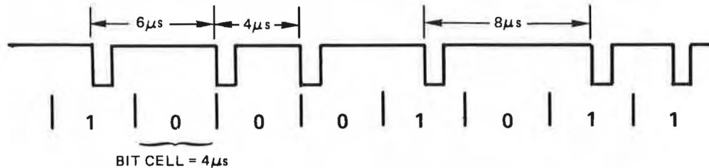
Figure 3-22: MFM Encoding
