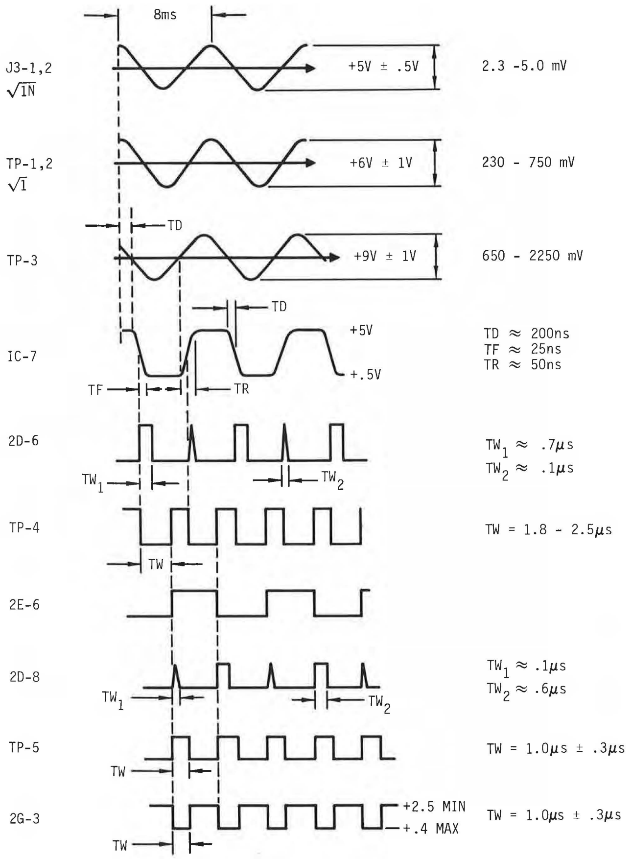
Figure 3-20: Read Timing
