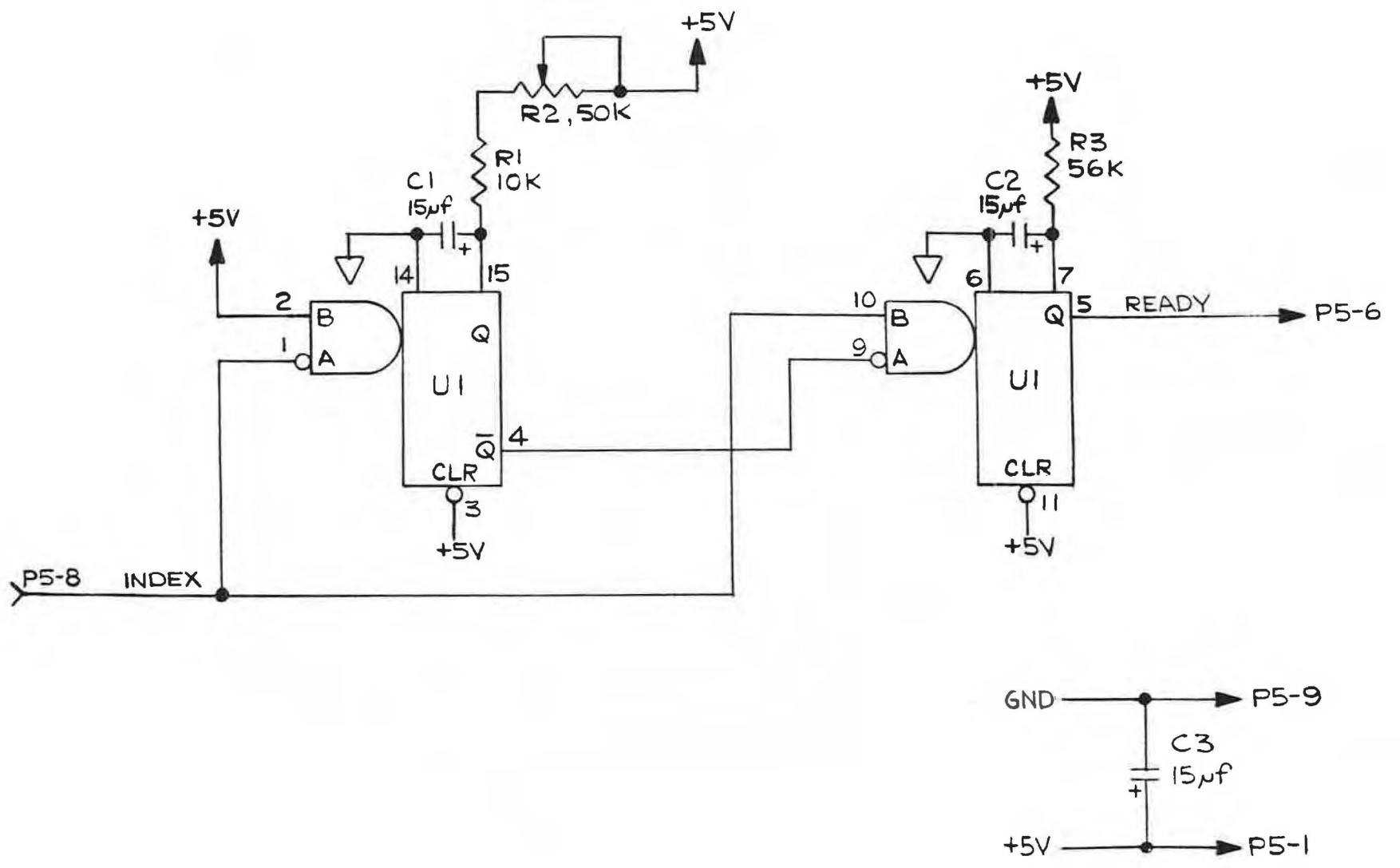
Figure B-4: Ready PCBA Schematic B-6
