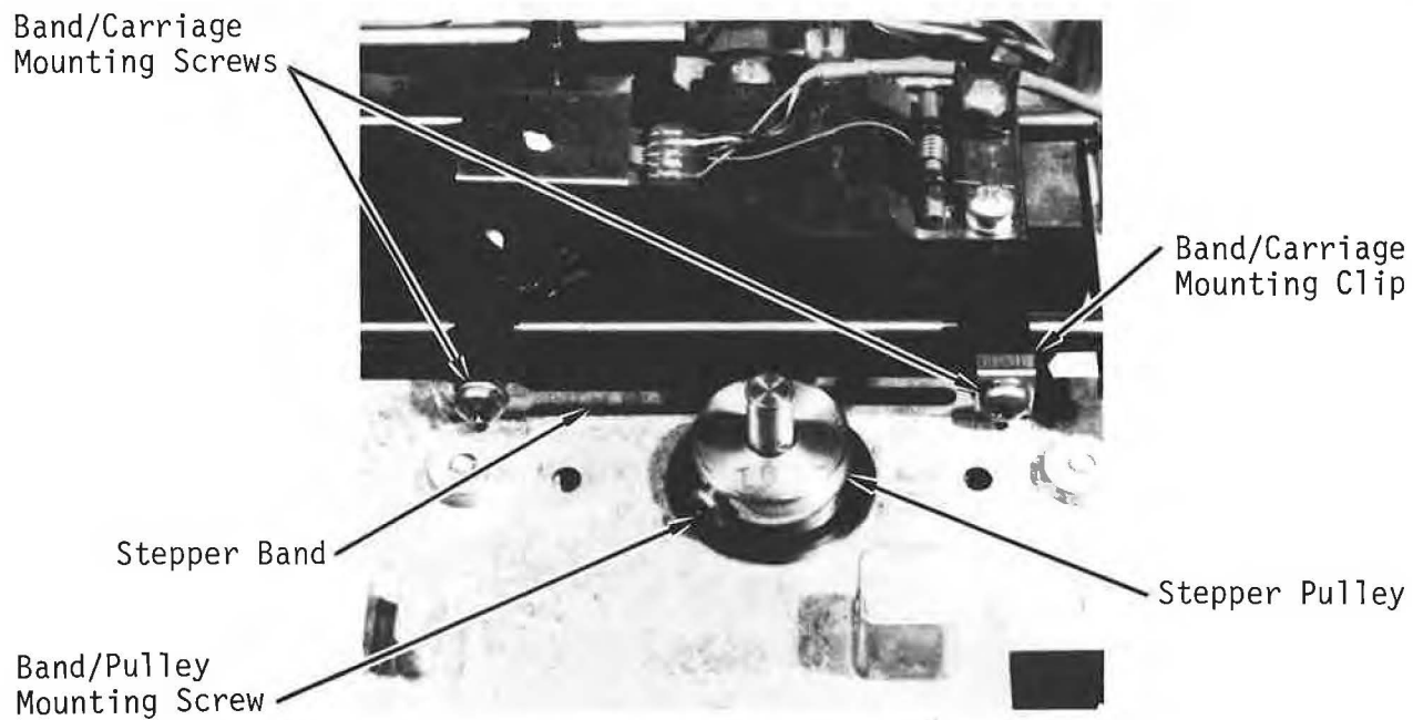
Figure 4-6. Stepper Band
