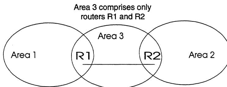
Figure 6-4: Address Summaries Exported Between Two NLSP Areas
