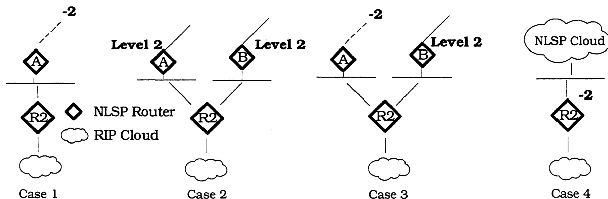
Figure 9-2: Advertising a -2 Network
