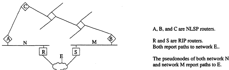
Figure 8-4: Multiple XRoutes for a Destination
