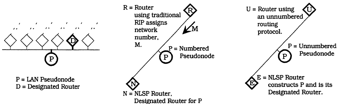
Figure 5-1: Pseudonodes
