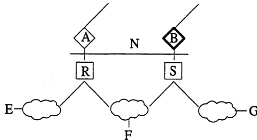
Figure 8-1: Routing between NLSP and RIP
