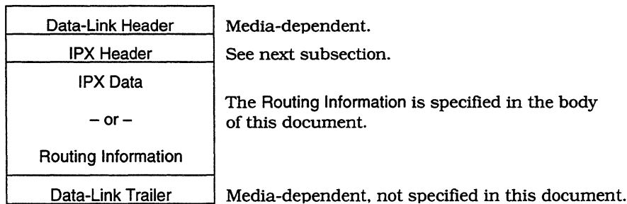
Figure 2-12: Data-Link Packet
