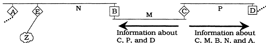
Figure 8-6: Split Horizon
