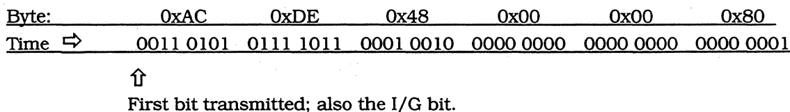
Figure 12-2: Standard Transmission of Universal Address
