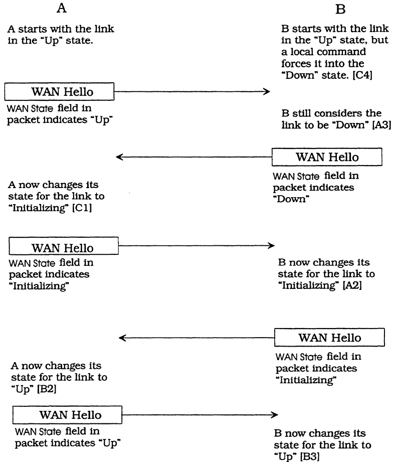
Figure 4-3: Recovering a WAN Adjacency
