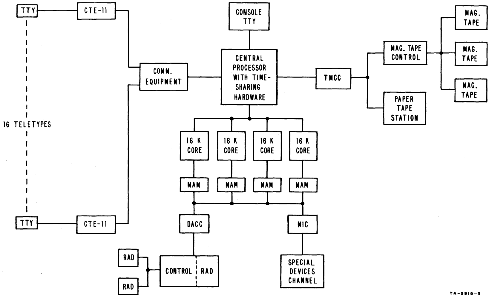
FIG. III-1 FACILITY CONFIGURATION OF SDS 940 COMPUTER
