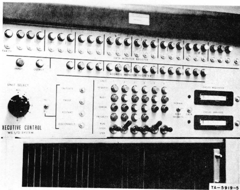
FIG. III-3 EXECUTIVE CONTROL DEBUGGING PANEL
