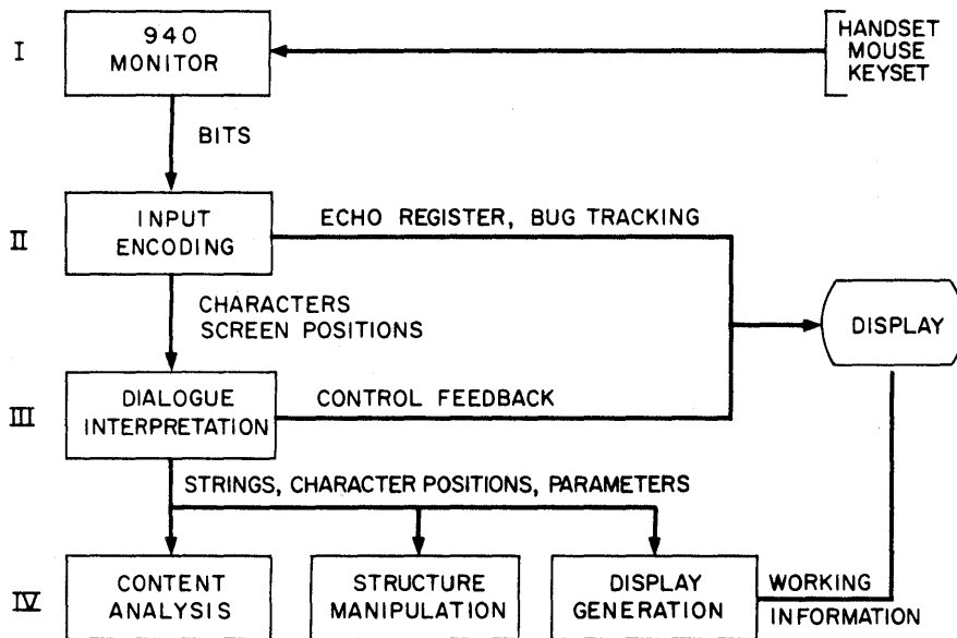
FIG. II-1 FUNCTIONAL ORGANIZATION OF NLS 940
