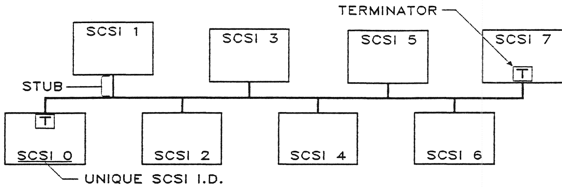
FIGURE 7 MAXIMUM SCSI CONFIGURATION
