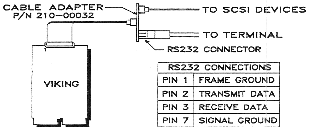
FIGURE 8 SERIAL PORT CABLE ADAPTER
