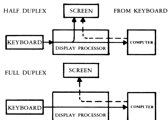
Figure 3-1 Model 910 Communications Flow
