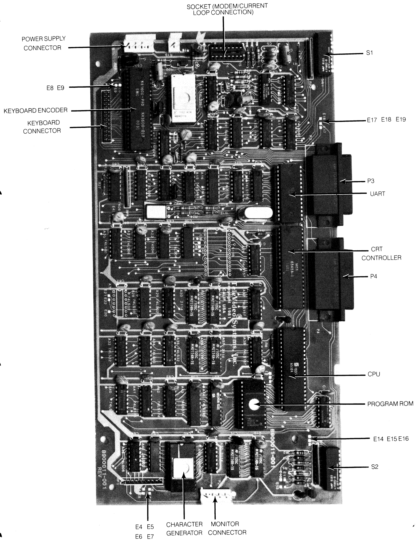
Figure 2-3 Logic Board
