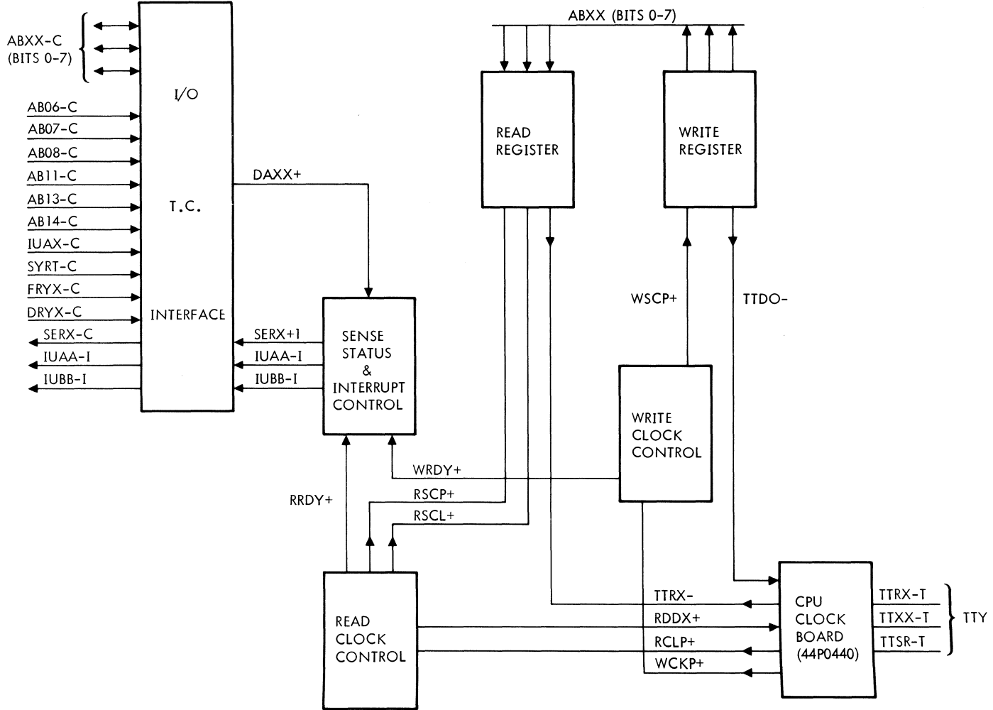
Figure 4-1. TTY Functional Block Diagram
