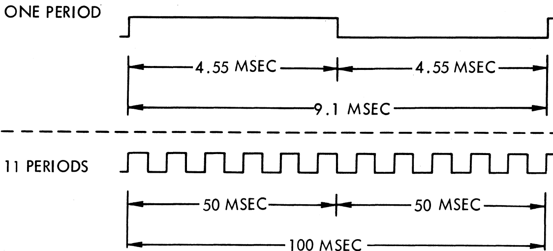
Figure 5-4. Waveforms for Transmit Clock Adjustment
