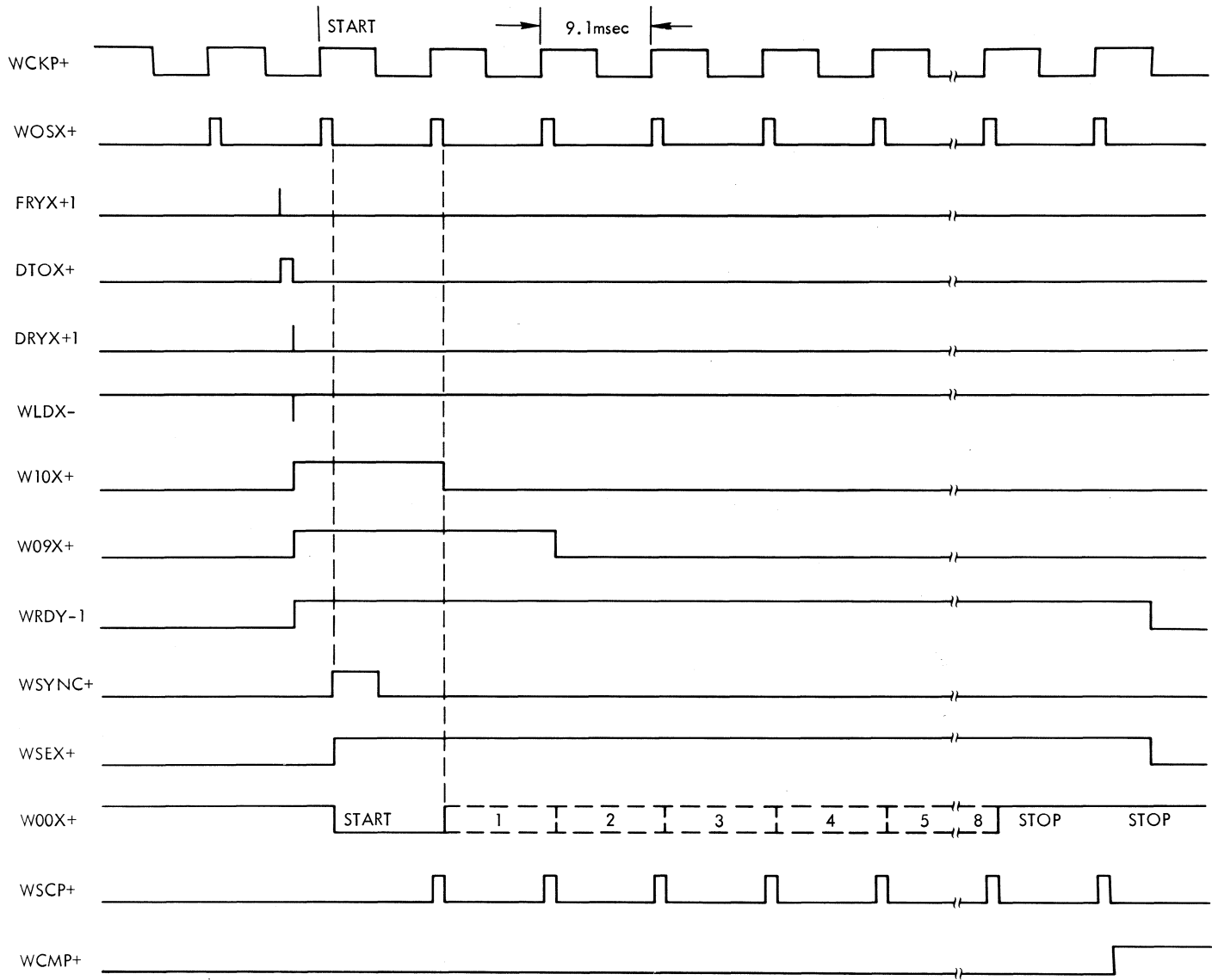
Figure 4-2. External Control Timing
