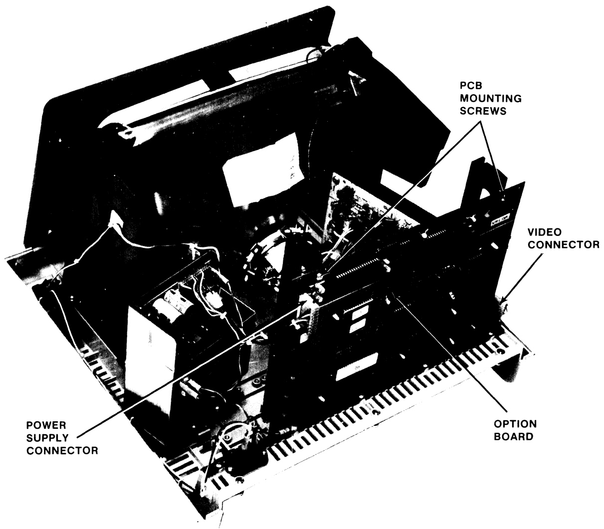
Figure 9-2. PCB Mounting
