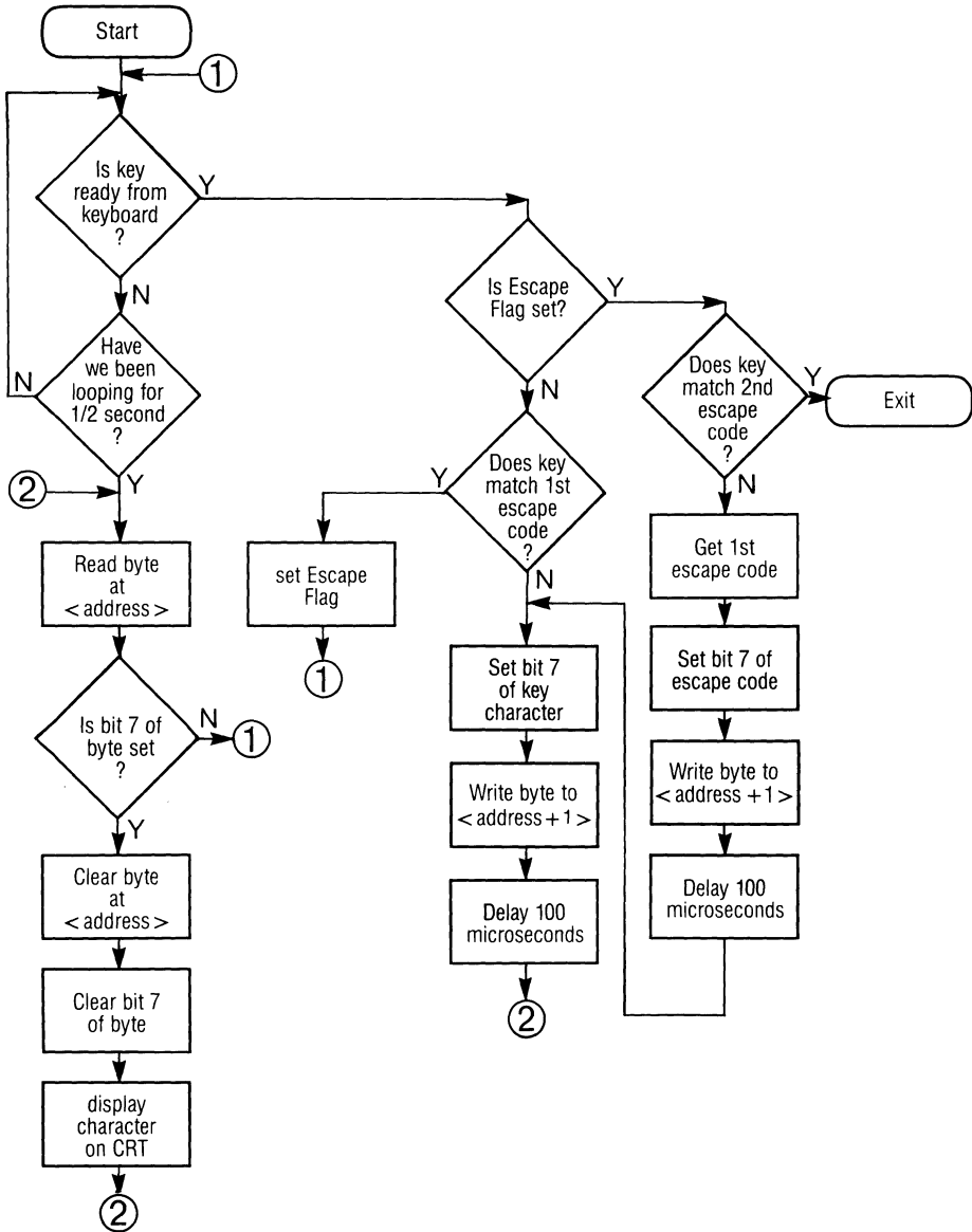
Figure 6. Flow Chart
