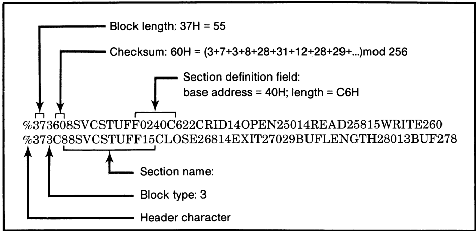
Figure 21. Tekhex Symbol Block
