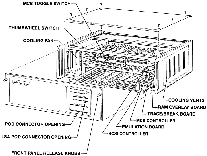
Figure 2. Control Boards
