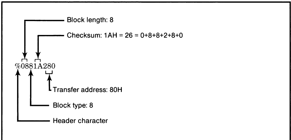
Figure 20. Tekhex Termination Block
