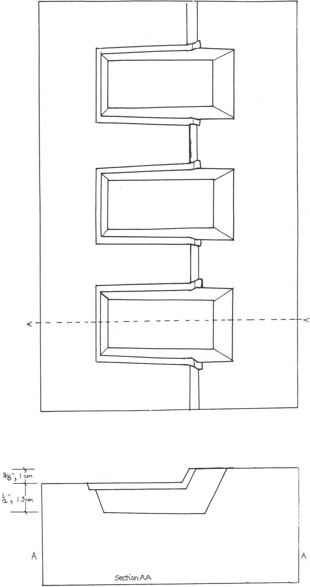
Second pothole potrest mould Scale 1:1
