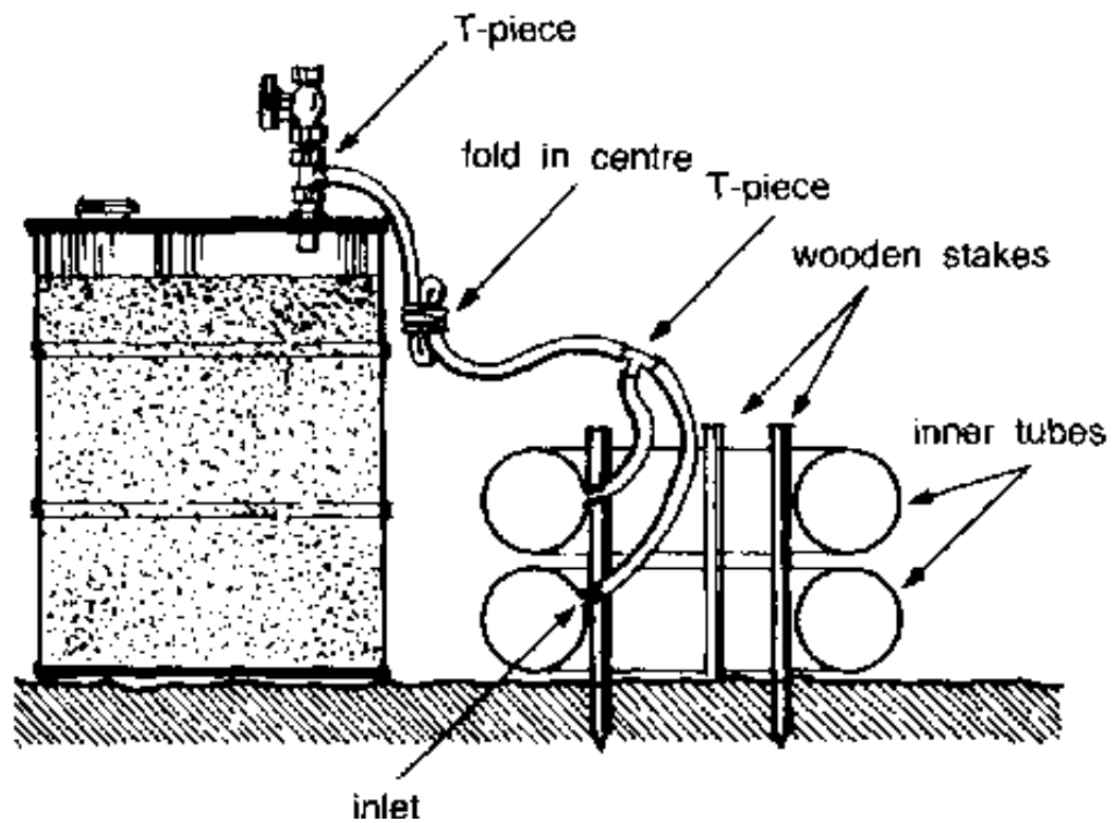
Biogas unit
