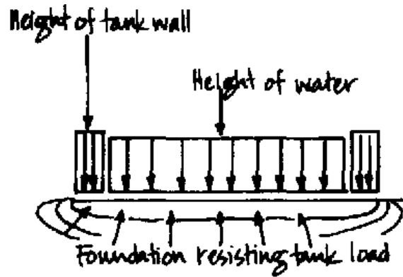
Figure 6B: Walls and floor separate
