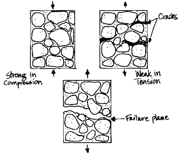
Figure 3: MORTAR UNDER LOAD
