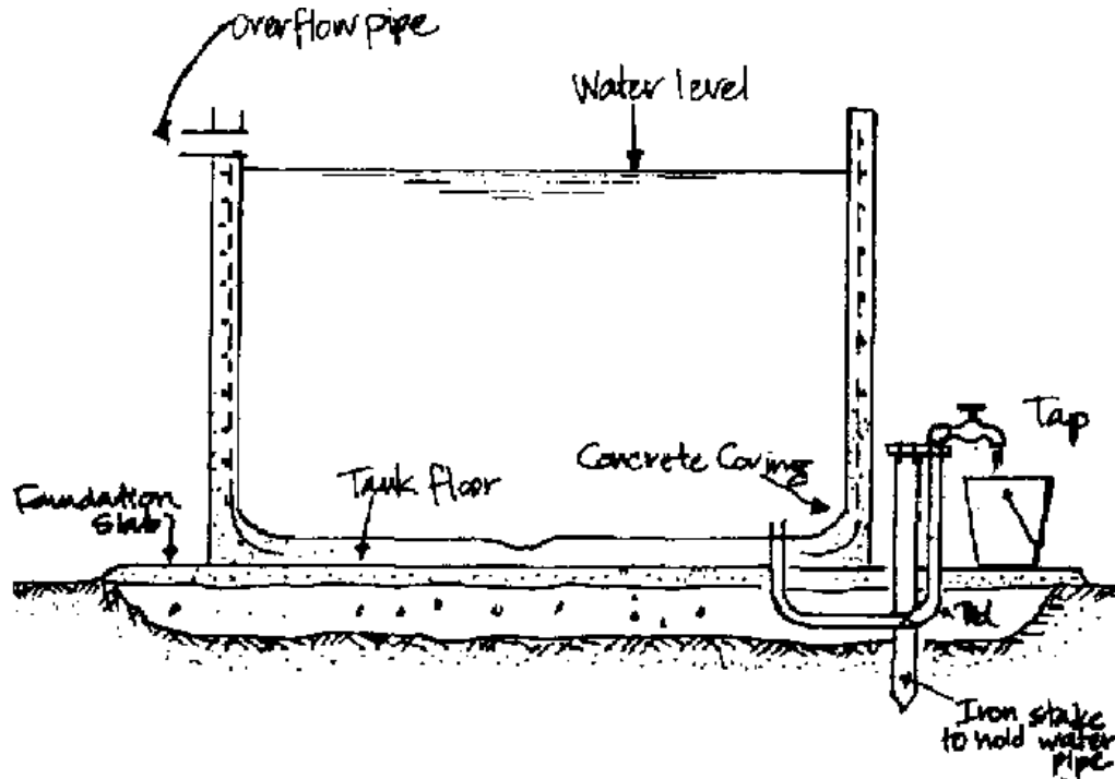
Figure 22: The completed tank
