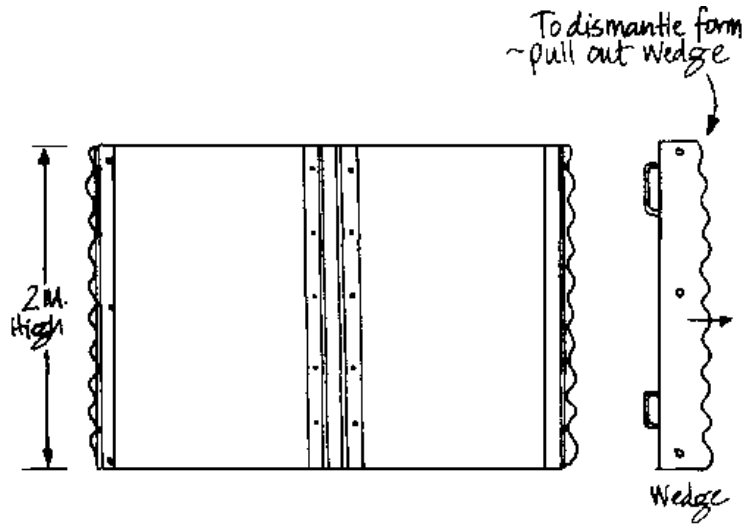
Figure 18: Standard formwork for 10 cubic meter tank - cross section of form
