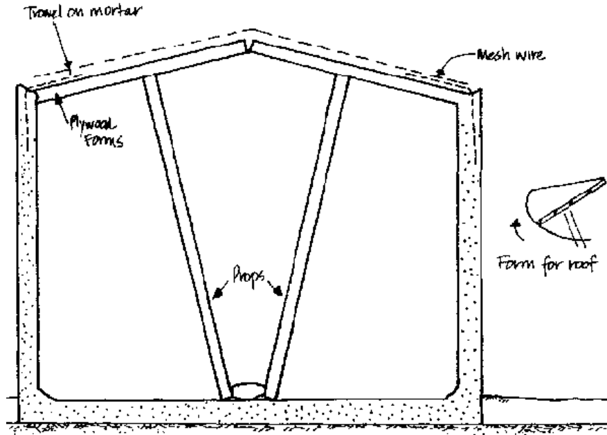
Figure 31: Constructing the roof
