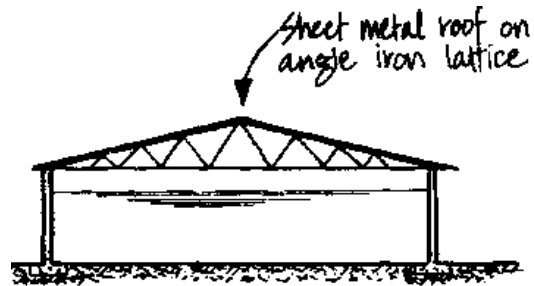
Figure 12: Roof for larger tank
