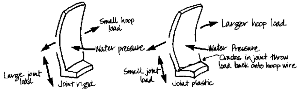
Figure 9: How the loads are taken
