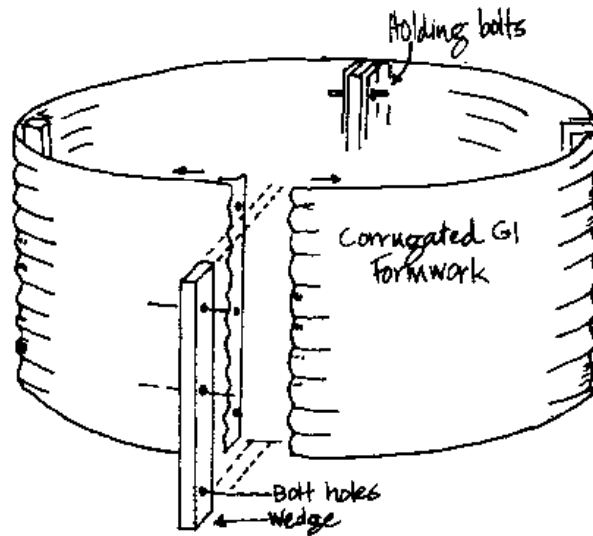
Figure 19: Tank foundation
