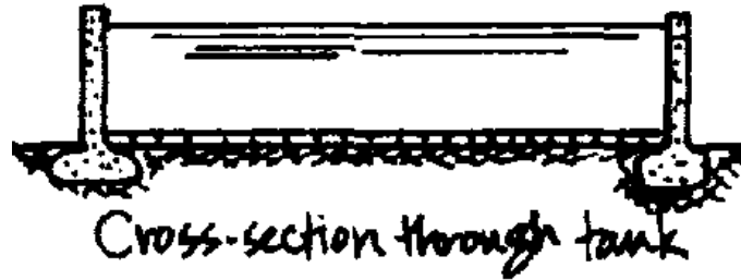
Figure 6A: Foundation of Large open tank -
