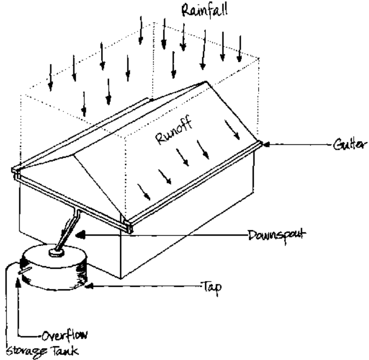
Figure 1: Catching and using the rain water from a roof
