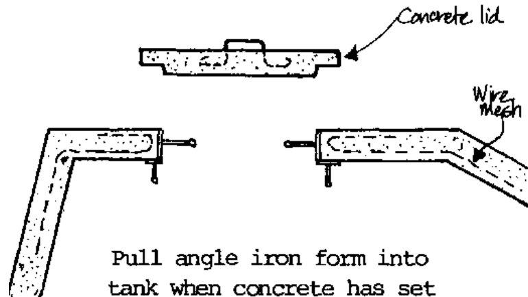
Figure 32A: Making the access hatch
