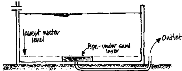
Figure 14: Slow sand filter in tank over outlet
