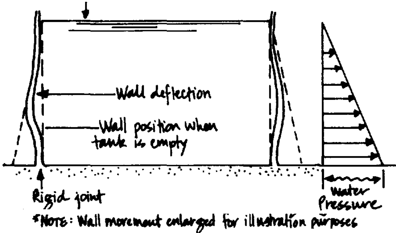
Figure 8: WALLS JOINED WITH FLOOR
