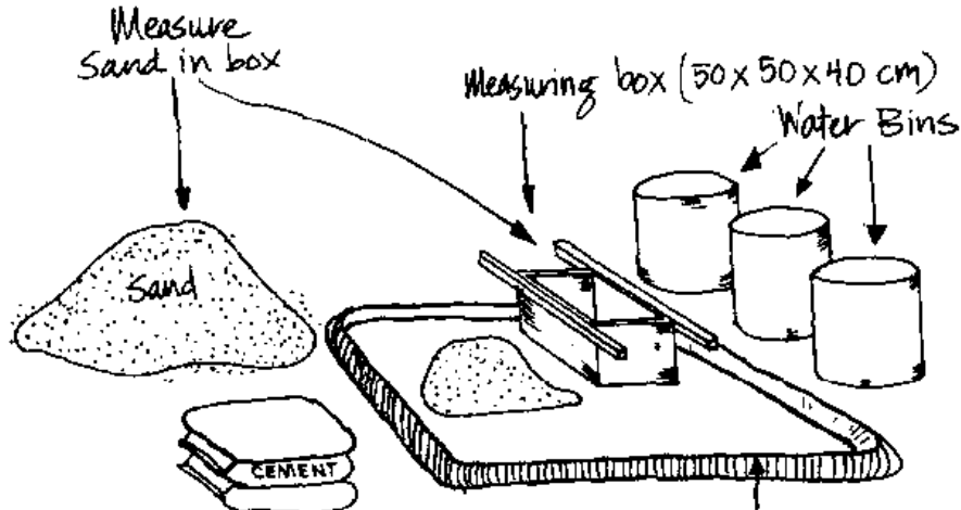
Figure 15: Mixing the concrete by hand
