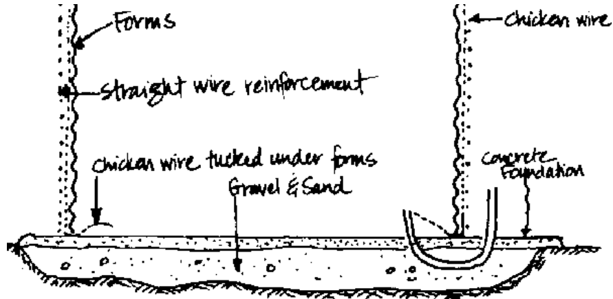
Figure 21: Erecting formwork and winding on reinforcing wire
