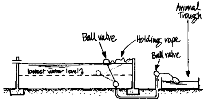
Figure 13: Ball valves for cattle watering
