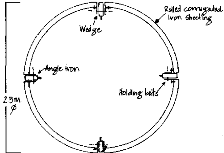
top view of formwork
