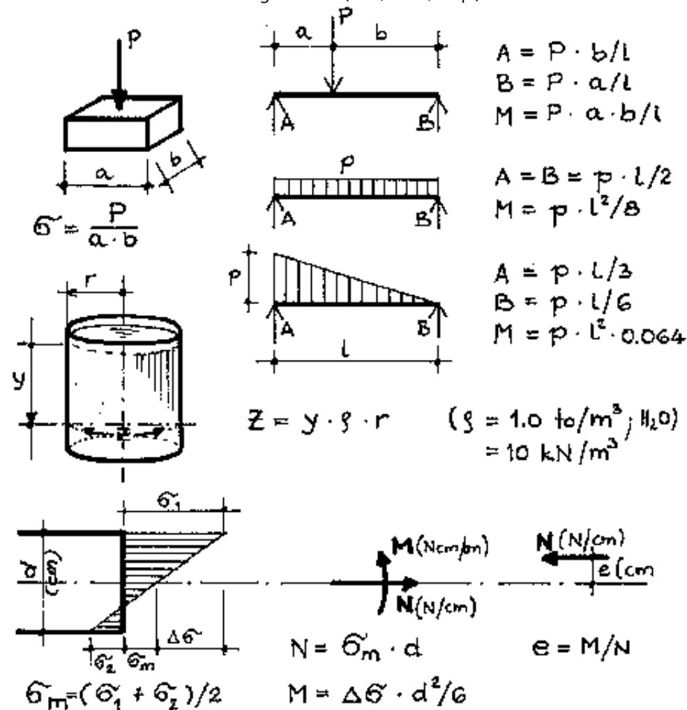
Fig. 56: Fundamental static formulae Static calculations are not usually necessary for small, simple biogas plants. For larger plants, a rough calculation should be carried out to determine whether the loads and stresses are likely to be high enough for an exact calculation to be necessary. Spherical and conical shells are complicated forms. They are very difficult to estimate by rough calculation. As a rule, only the edges are loaded to the permissible limit.
