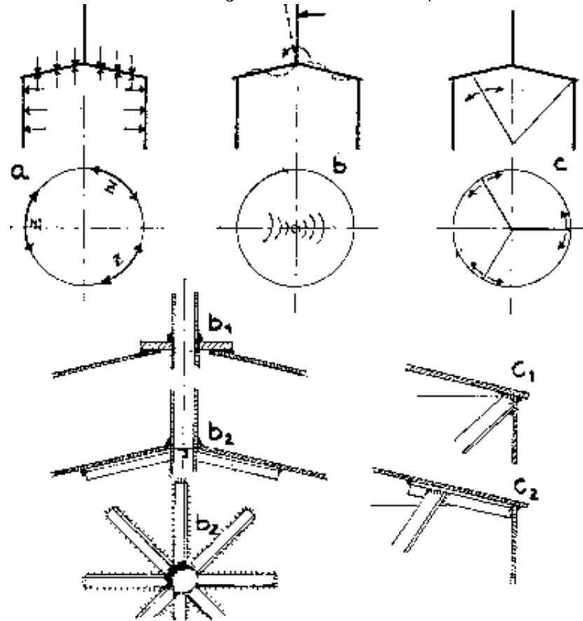
Fig. 30: Forces on the gas drum The gas pressure and the weight of the metal itself give rise only to tensile forces in the jacket sheet. No reinforcements are necessary for these to be withstood (a). The loads from the guide tube must be reliably transmitted to the cover plate (b). A flange plate (b1 ) or angle iron (b2) is required for this purpose. The braces are stressed when the drum is rotated (c). They should not simply butt on to the metal but end in a corner (c1 ) or at an angle (c2).
