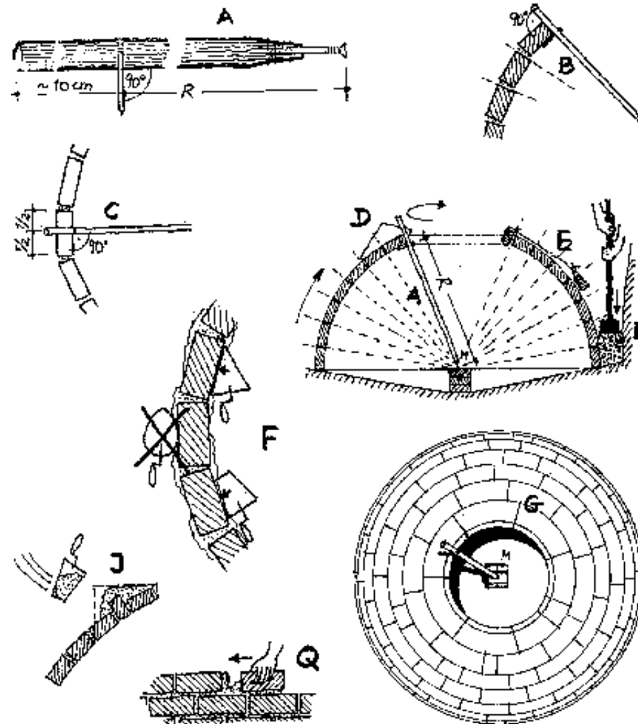
Fig. 21: Construction of a spherical shell from masonry
