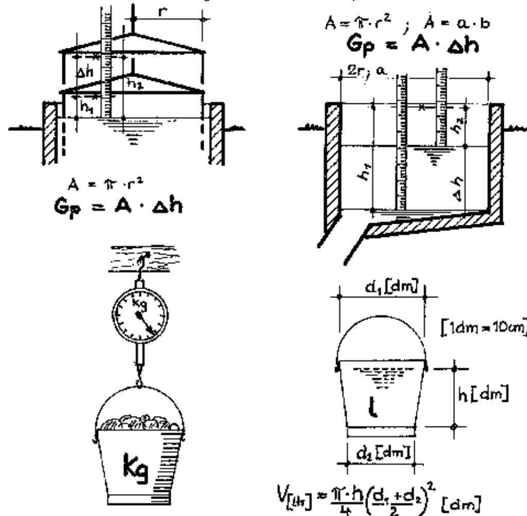
Fig. 15: Measuring gas production on the plant In a floating-drum plant, the height of the gasholder is measured (top left), In a fixed-dome plant, the height of the slurry level is measured (top right). The manure is either weighed or measured in litres before introduction to the plant. Containers whose shape is easy to calculate are more accurate. If the lengths are measured in dm (1 dm = 10 cm), the volume in litres is obtained directly.
