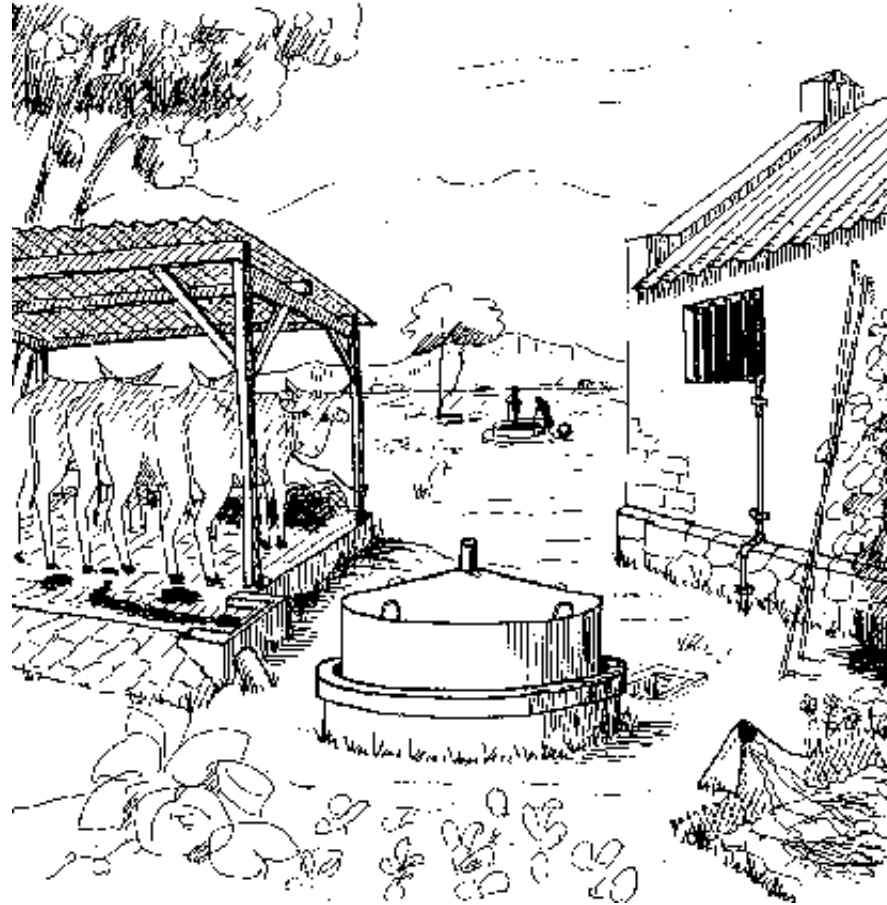
Fig. 1: A farmyard biogas plant This is a floating-drum plant with internal gas outlet. The gas pipe is securely mounted on the wall and leads directly to the kitchen. Ideally, as in this example, the digester should be located directly beside the animal shelter, which should have a paved floor. Urine and dung can be swept into the inlet pipe with little effort. The plant has a sunny location, and the vegetable garden is situated directly adjacent to the digested slurry store. The well is an adequate distance away from the biogas plant.
