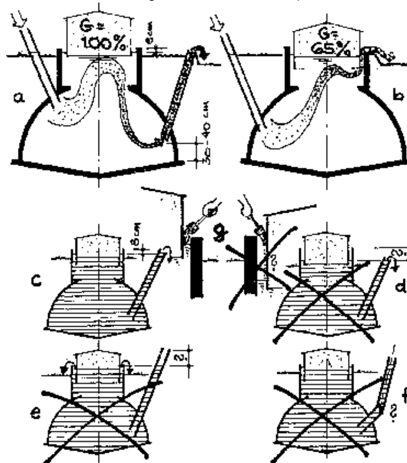
Fig 28: Outlet (overflow) of a floating-drum plant The outlet should be placed below the middle of the digester, otherwise too much fresh feed material will flow out of the plant too soon, thus reducing gas production by as much as 35 % (b). The height of the outlet determines the level of the surface of the fermentation slurry (c-f). This should be 8cm below the top edge of the wall. If this is not the case, difficulty will be experienced in painting. If the outlet is too low, digester volume is lost (d). If it is too high, the slurry will overflow the edge of the wall (e).
