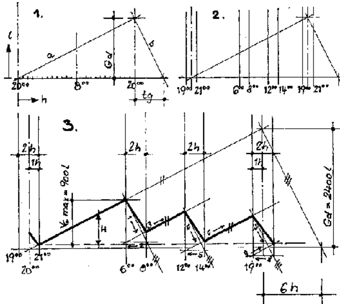
Fig 9: Graphic determination of required gasholder volume in accordance with the first example, page 21/22. Working steps: 1. Plotting of gas production curve (a) and gas consumption curve (b). 2. Plotting of gas consumption times. 3. The
