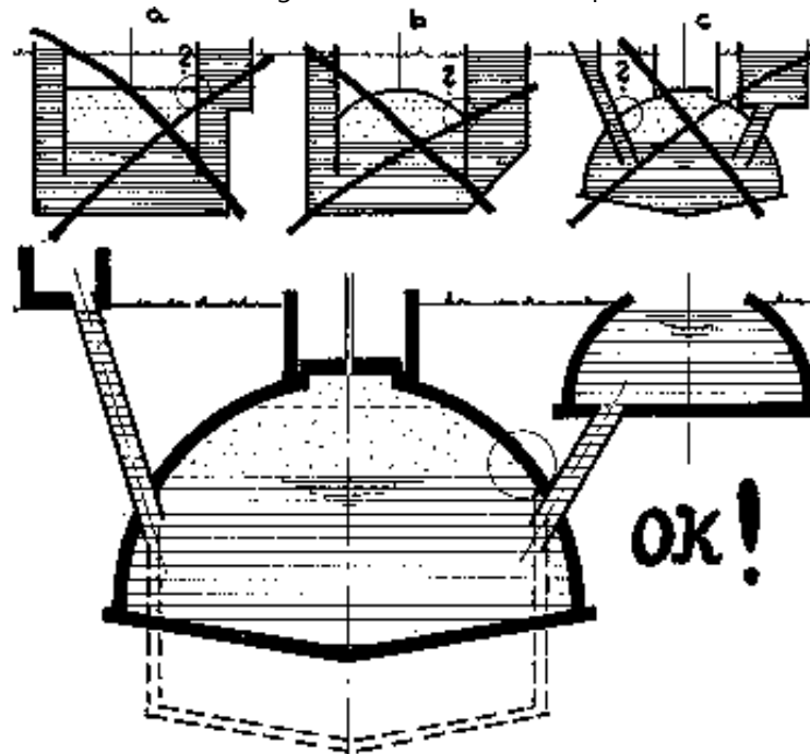
Fig. 19: Cracks in the gas space of a fixed-dome plant Angular gas spaces must on no account be used (a)! The transition from the roof arch to the wall must never be at a higher level than the lowest slurry line (b). Inlet and outlet penetrations must never be situated in the gas space (c). The gas space must remain undisturbed. Only the entry hatch at the top is allowed, because it can easily be checked.
