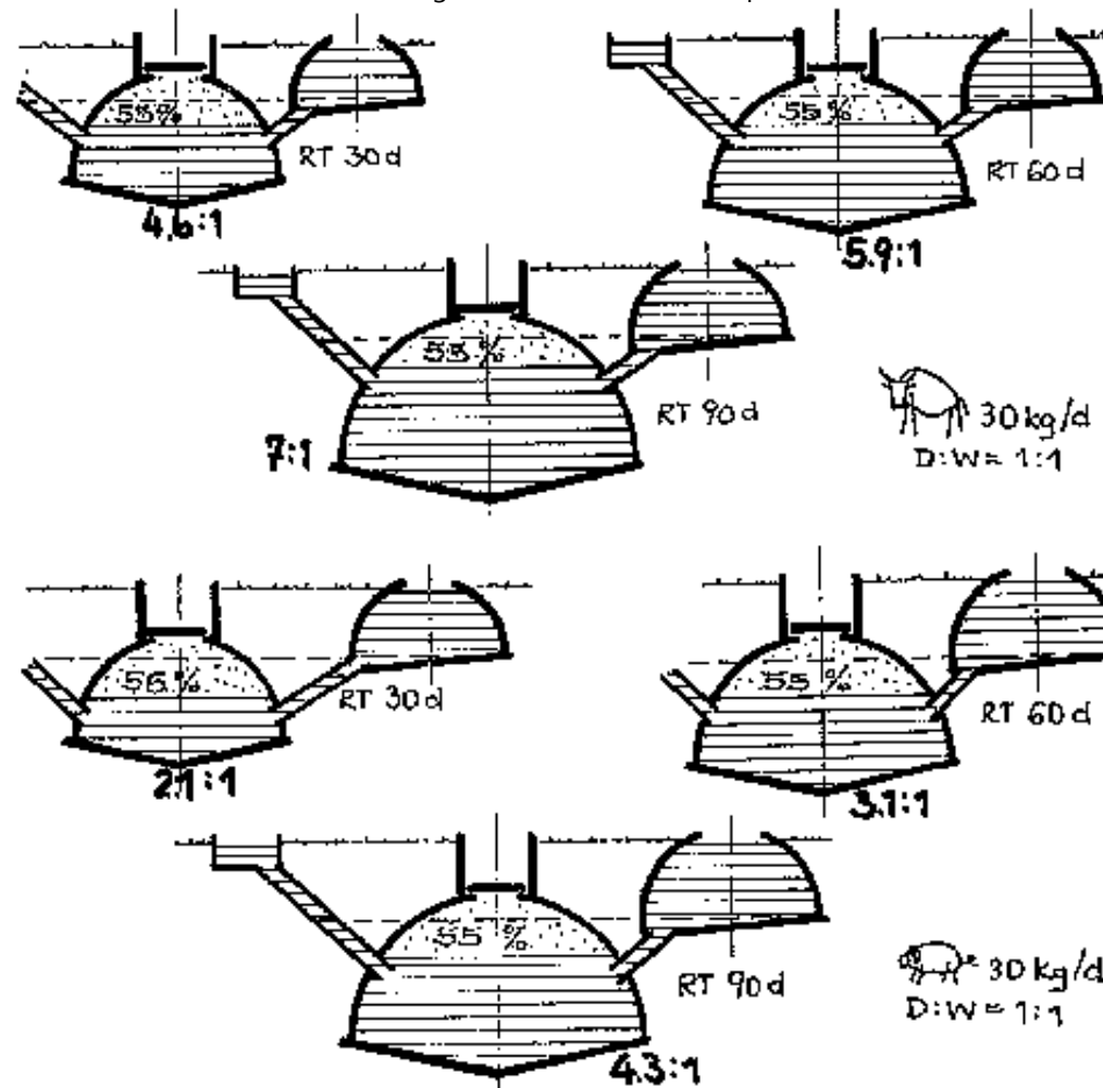
Fig. 13: Dependence of shape on retention time on a fixed-dome plant (cattle dung above; pig manure below) The filling volume and gasholder capacity ( C = 55\% ) are the same in each case. The differences in digester/ compensating tank ratios result solely from the different retention time (Gd as a result of RT, Figures 7 and 8).
