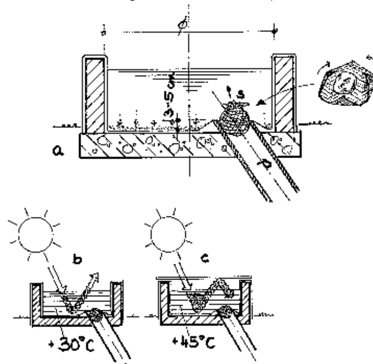
Fig. 23: Mixing tank at inlet Grit and stones settle at the bottom of the mixing tank. For this reason the inlet pipe (p) should be 3-5 cm higher than the tank bottom. A round, cylindrical shape is cheapest and best for the mixing tank. If the tank is filled in the morning and then covered, the slurry heats up in the sun until the evening (c). Only then is the plug removed (s).
