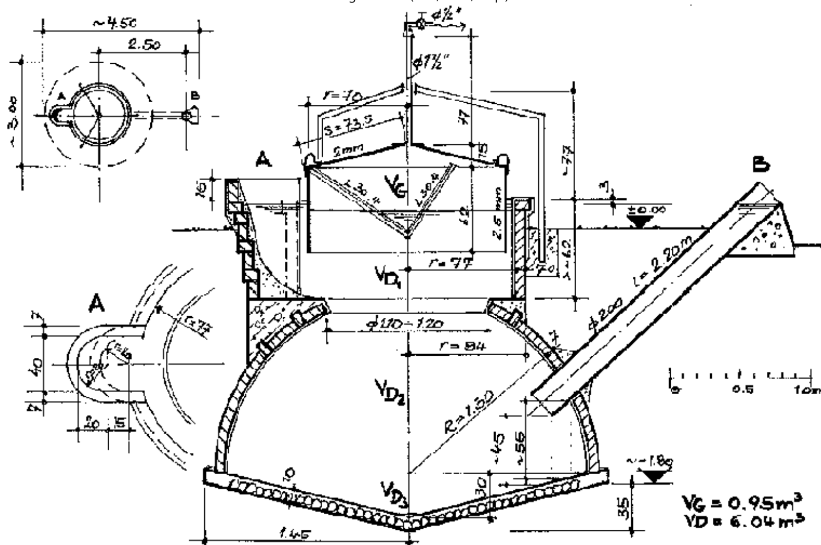
Fig. 43: Constructional drawing of a floating-drum plant with filler funnel for long-fibre feed material; external guide, external gas outlet.
