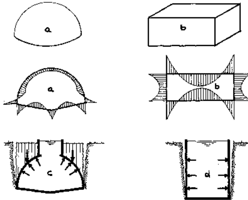
Fig. 17: Same volume - different shape Different shapes have different stress patterns under the same load (a and b). The round shape has lower stresses. The angular shape has high stresses and many stress peaks. Different shapes are often loaded differently. In a vaulted shape, the loads acting in different directions are more reliably balanced than with a vertical wall (c and d).
