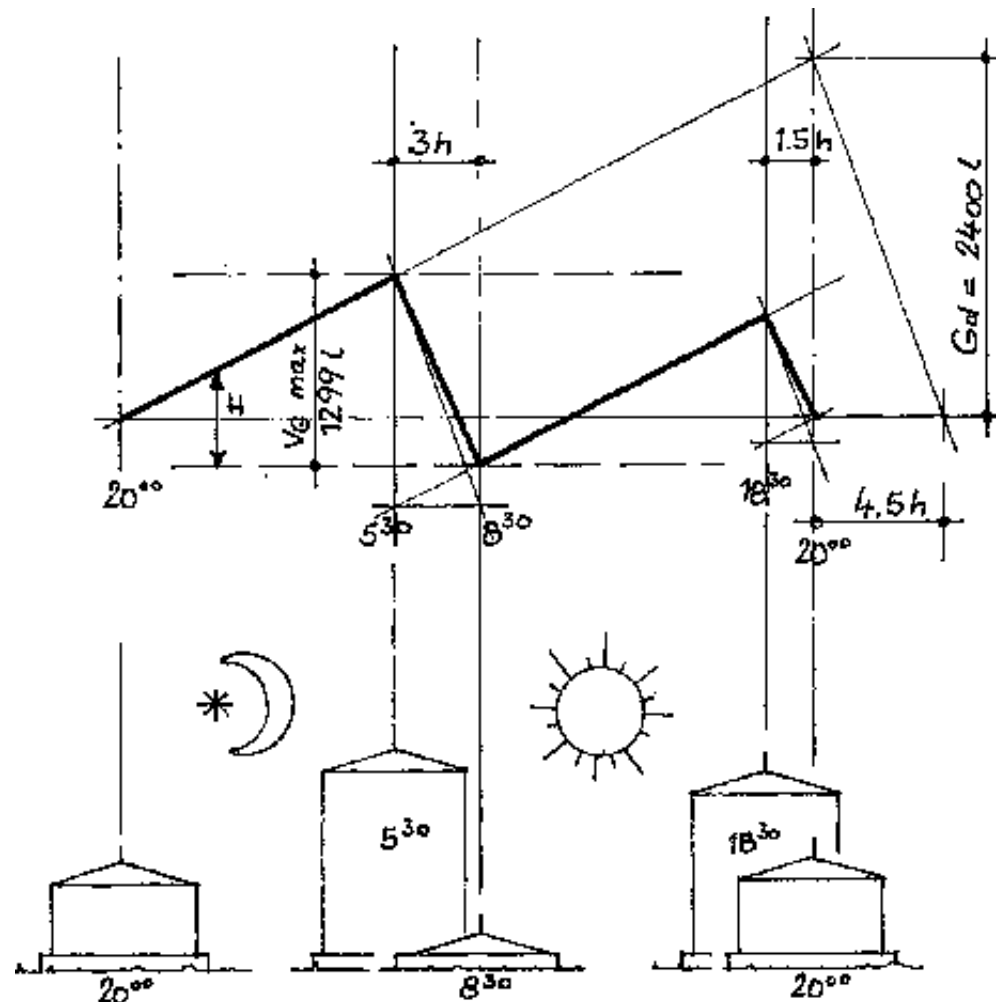
Fig. 10: Graphic determination of the required gasholder volume in accordance with the second example on page 23/24. The safety margin of 25 % for fluctuating gas production must be added to the value VG. The distance H can also be regarded as the height of the floating gas drum. Experience shows that about the
