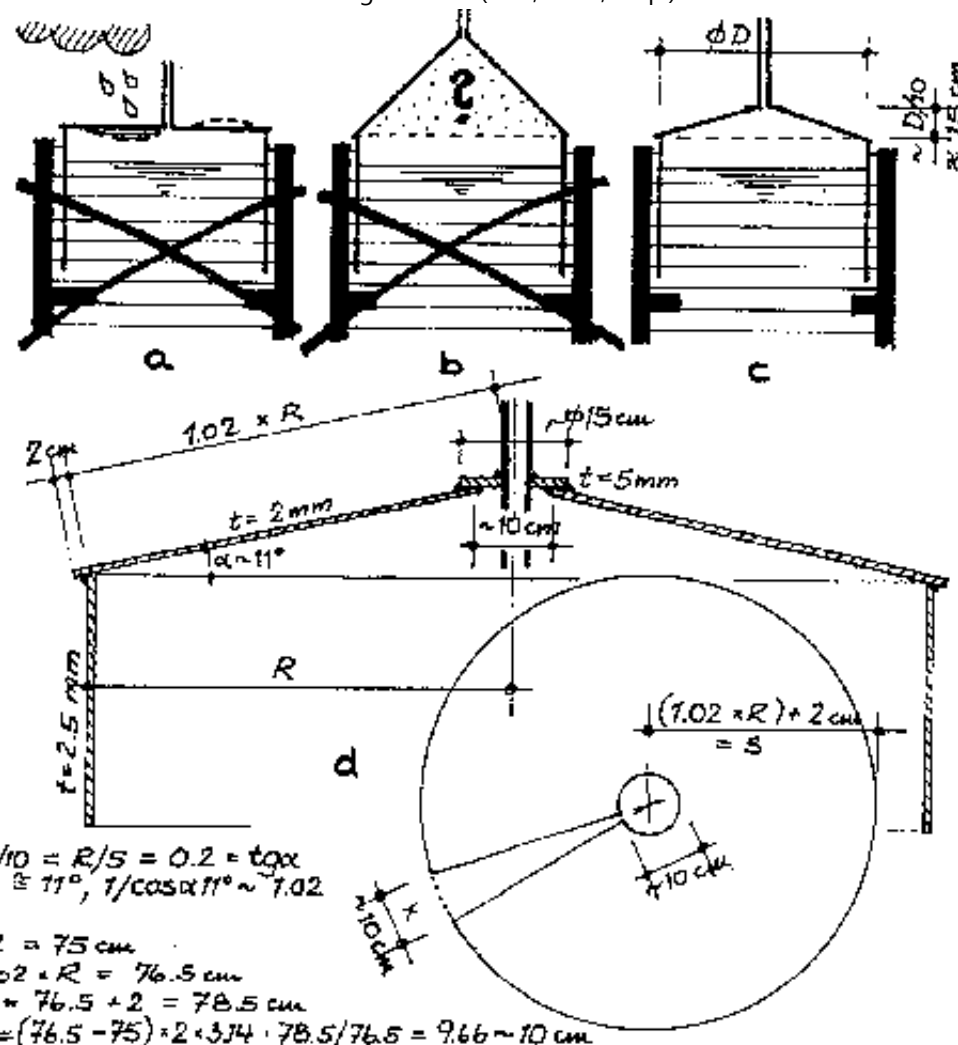
Fig. 29: The gas drum The gas drum should have a slightly sloping roof. When the cover plate is cut, a wedge (k) should be cut out. The cover plate must be rather larger than the diameter of the drum (see calculation at bottom left). Inaccuracies can more easily be corrected if a lateral overhang of 2 cm is allowed.
