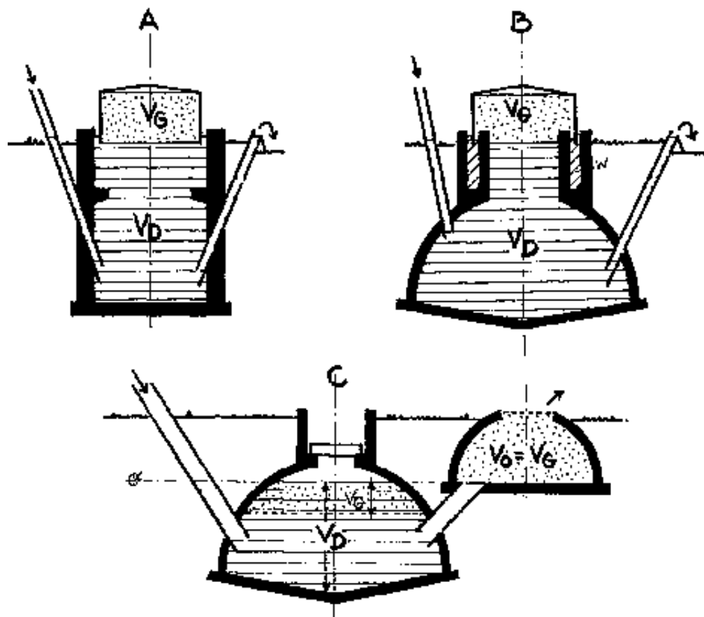
Fig. 6: Digester and gasholder Each biogas plant consists of a digester (VD) and a
