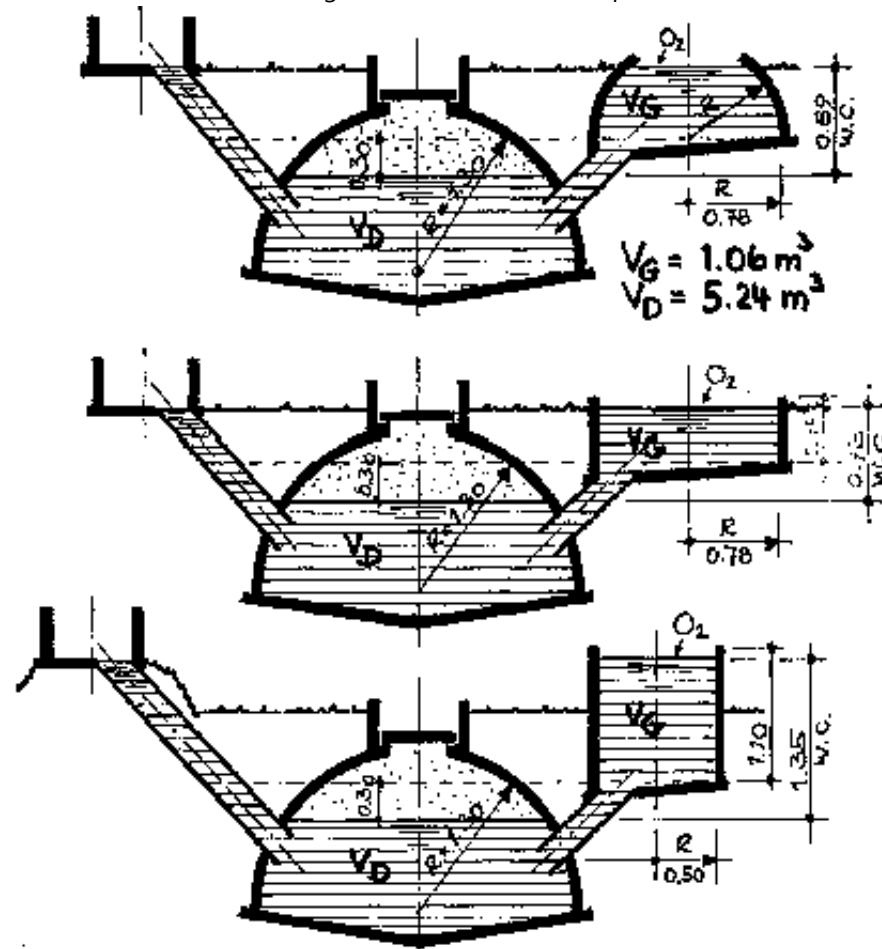
Fig. 36: Shape of compensating tank The shape of the compensating tank determines the height of the slurry surface and hence the gas pressure (cm WC). The lower the compensating tank, the lower and more even the gas pressure. However, the lower the tank, the larger the area exposed to atmospheric oxygen. Differences in building costs due to shape are slight.
