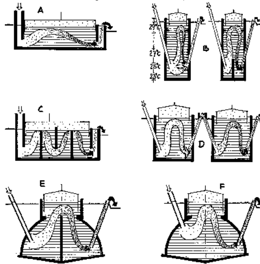
Fig. 25: Path of the fermentation slurry in the digester Fresh fermentation material is lighter than fully digested sludge. For this reason the former quickly rises to the surface and then sinks only gradually. The digestion process has two phases. The better these phases are separated, the more intensive the gas production. The fermentation channel (A) satisfies these conditions best. Tandem plants are expensive and complicated (D). The deeper the digester, the lower and less uniform its temperature.
