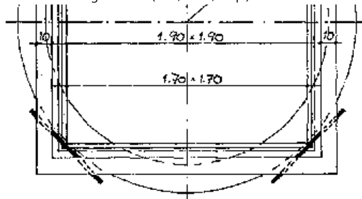
Fig. 52: Constructional drawing of a channel-type digester with folia (Henning system) The digester walls consists of netting-wire-reinforced rendering on the surrounding ground. The balloon serving as gasholder is mounted on a wooden frame. A plywood panel or straw mat on lathing serves as a sunshade. Weights placed on top make the gas pressure higher.
