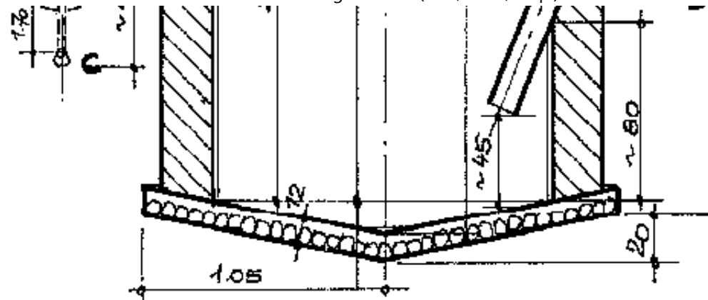
Fig 50: Constructional drawing of a floating-drum plant for quarrystone masonry (vertical plant)
