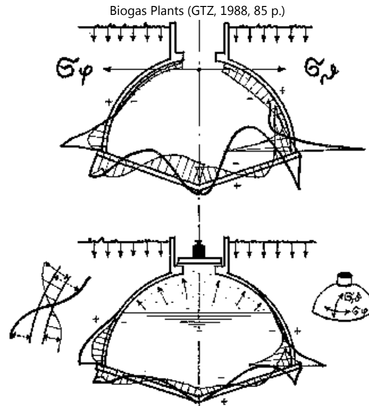
Fig. 18: Pattern of stresses in a fixed-dome plant of masonry construction Top: empty; bottom: filled and with maximum gas pressure. The peak stresses shown are those resulting from the first approximation calculation. In practice they are reduced by deformation (with or without cracking). Positive (+) tensile stresses do not occur in the gas space.
