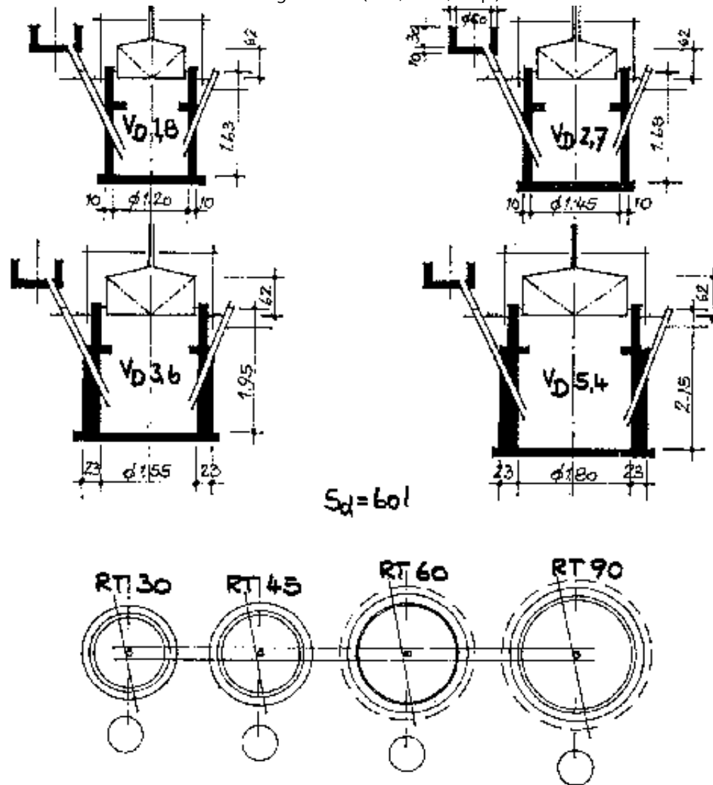
Fig. 14: Biogas plants for a test programme for determination of gas production The length of the retention time (RT) has the greatest effect on digester size (VD). Test plants may have any shape. However' they should all be identical and should preferably conform to the type to be used later in a biogas programme. The test plants must be filled regularly for at least three months before gas production is measured. The gasholders must be all the larger, the longer the time between
