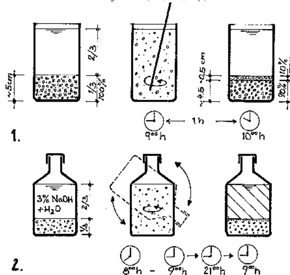
Fig. 22: Testing of mortar sand 1. Fines (loam, dust): Water glass 1/3 sand, 2/3 water. stir vigorously. Leave to stand for one hour. Measure fines. A maximum of 10 % of the amount of sand is permissible. 2. Organic matter: Bottle with stopper (not cork) to be filled with 1/3 sand and 2/3 soda lye (3 %). Shake repeatedly within an hour. Leave to stand for 24 hours. Water colour clear or light yellow: good; red or brown: bad.
