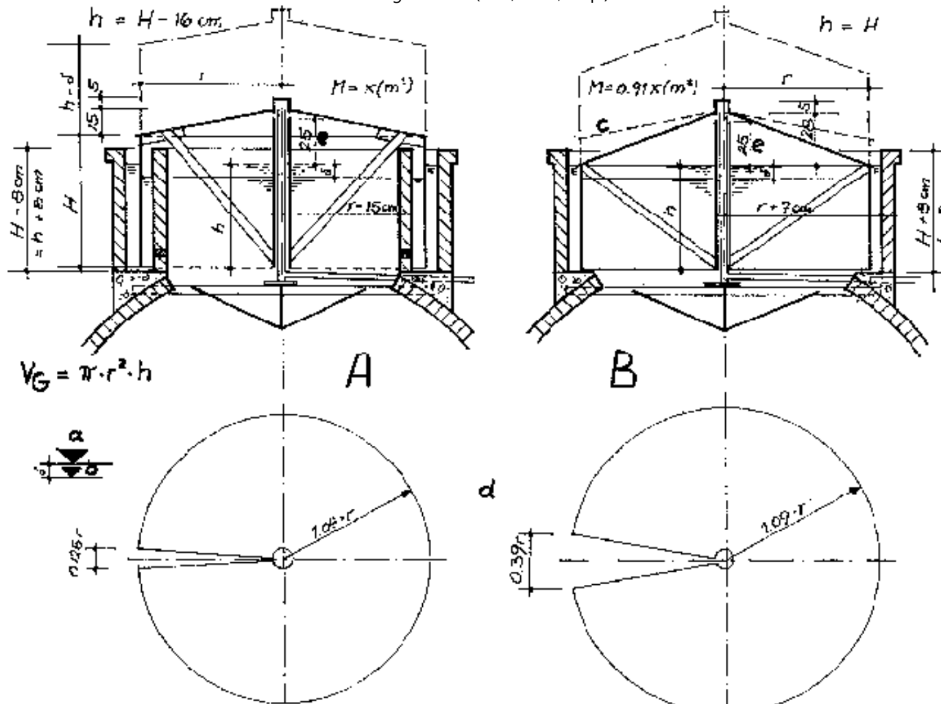
Fig. 34: Comparison of floating drums for water-jacket plants (A) and for plants with internal gas outlet (B): Both types of plant are assumed to have the same gas-holding capacity. The distance between the top rim of the gas outlet pipe and the slurry level (A) depends on the shape of the drum. a: Overflow level or unpressurized slurry level; b: Pressurized slurry level; c: gasholder configuration as in A; d: Comparison of sheet metal cutouts for drum lids.
