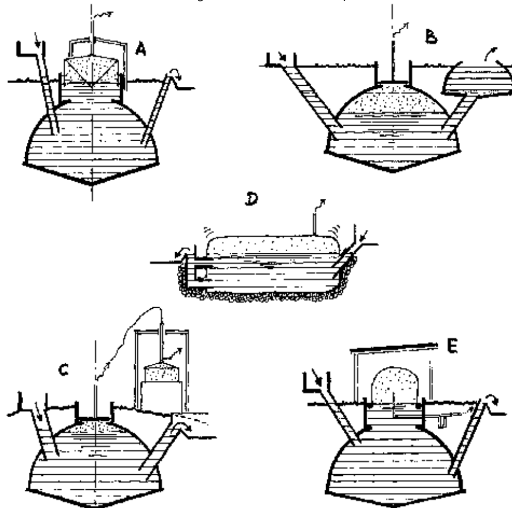
Fig. 3: Simple biogas plants A Floating-drum plant B Fixed-dome plant C Fixed-dome plant with separate gasholder. The gas pressure is kept constant by the floating gasholder. The unit can be operated as a continuous overflow-type plant with no compensating tank. The use of an agitator is recommended. D Balloon plant E Channel-type digester with folia and sunshade
