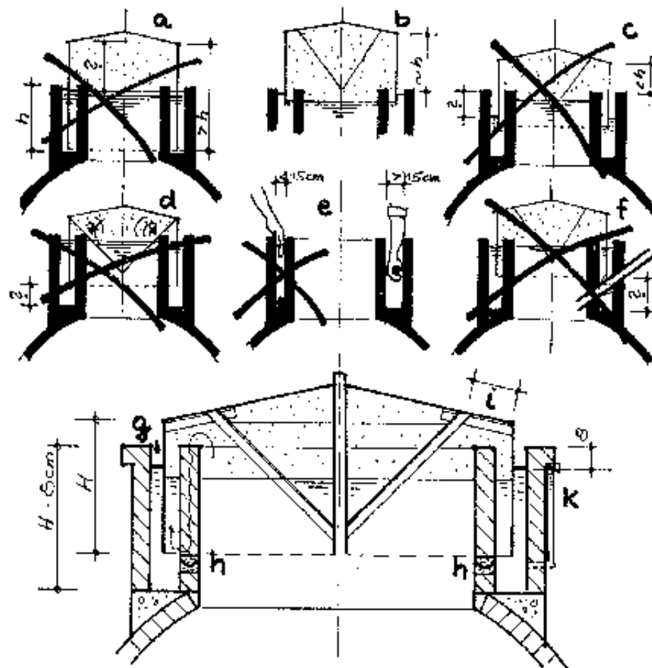
Fig. 33: The water jacket
