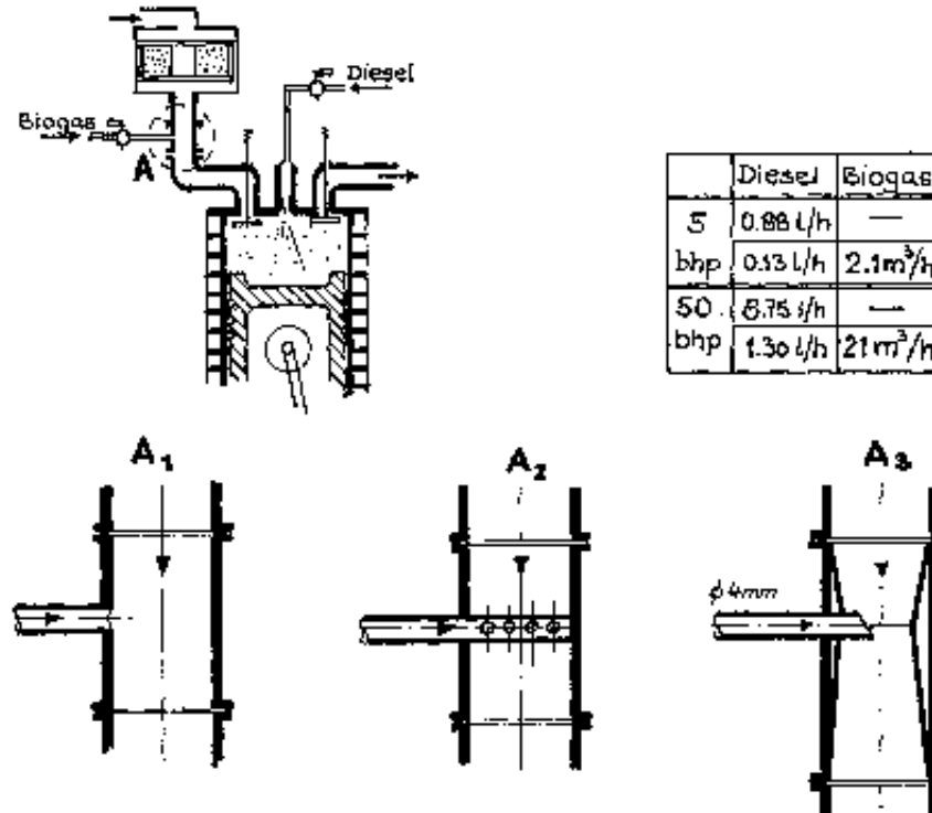
Fig. 42: Gas connection to diesel engine
