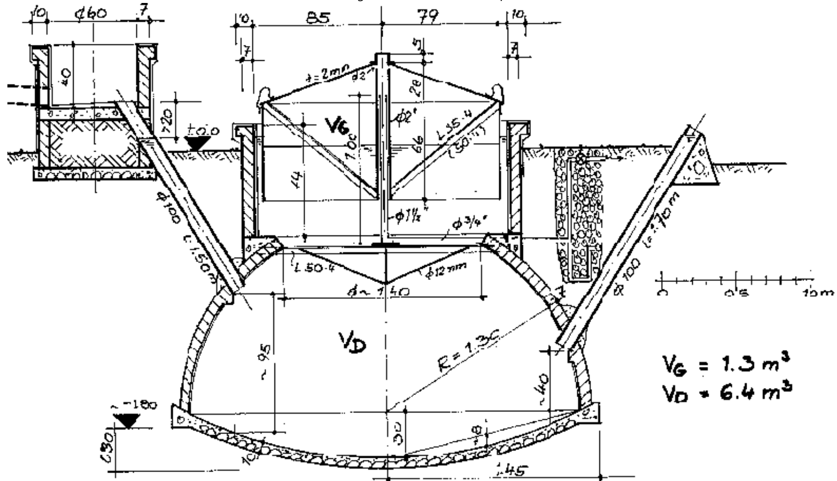
Fig. 45: Constructional drawing of a floating-drum plant with an internal gas outlet and no water jacket
