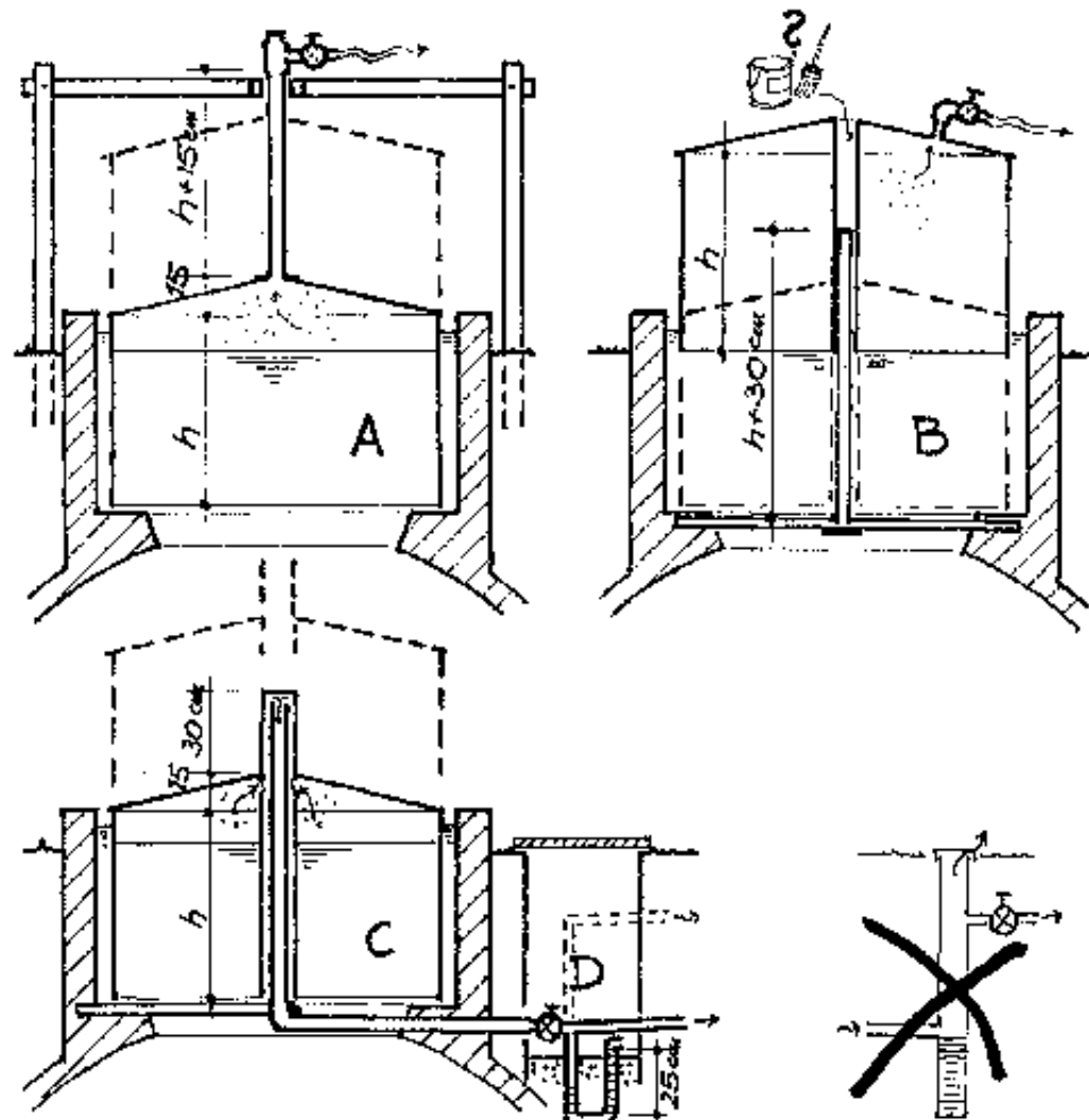
Fig. 31: Floating drum guide frame An external guide frame (A) is cheapest. It is
