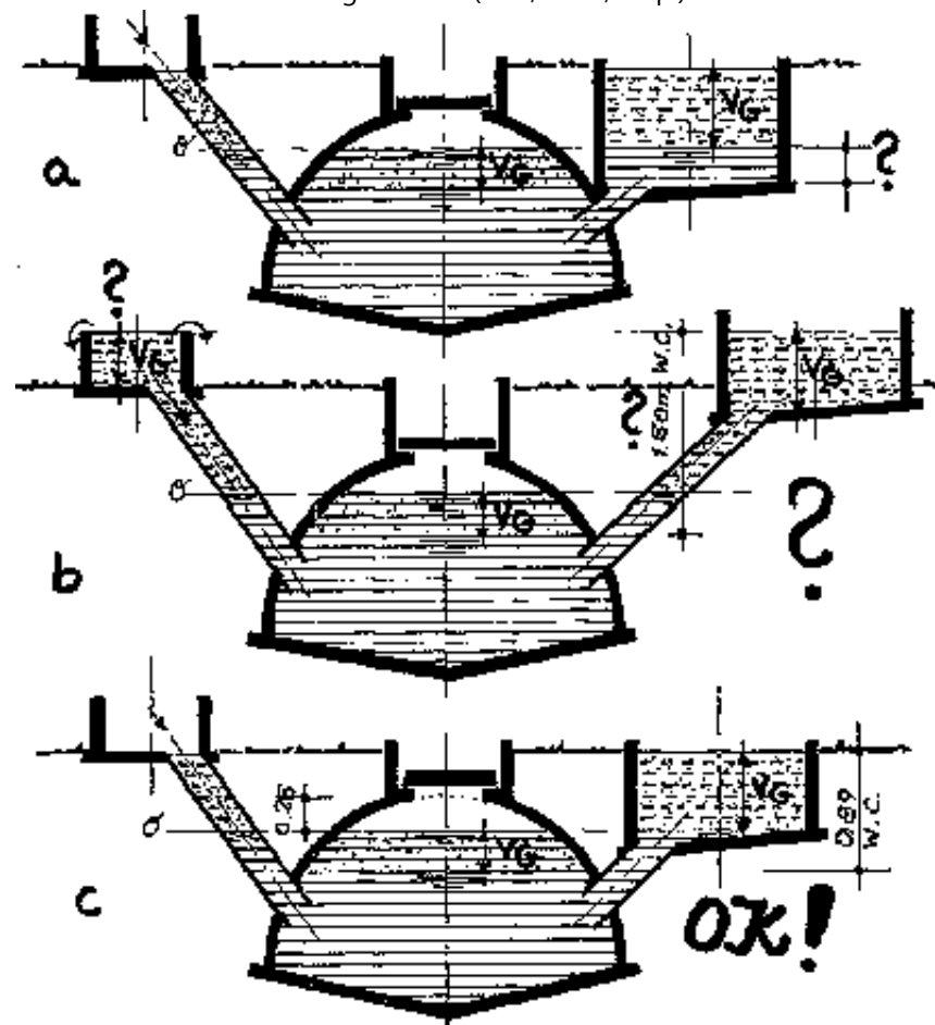
Fig. 35: Correct height of compensating tank The bottom of the compensating tank is at the level of the zero line (filling line). The zero line is 25 cm below the head of the digester dome (c). Wrong: (a) the bottom of the compensating tank is too low. Part of the slurry is always in contact with air. Gas is lost. Unnecessary cost. (b) The bottom of the compensating tank is too high. The gas pressure rises very fast and to a very high level.
