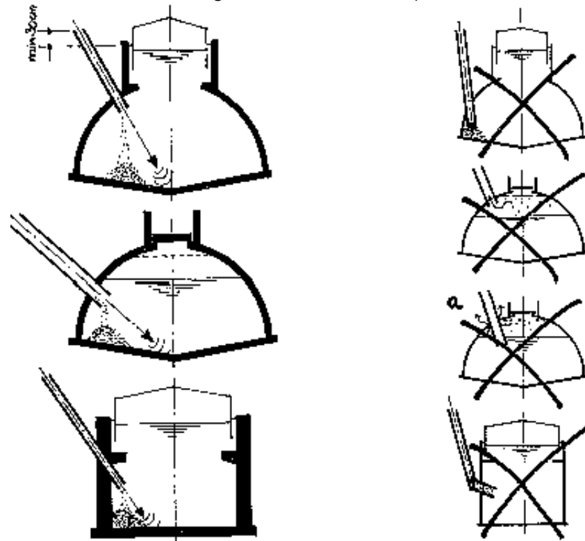
Fig. 24: The inlet must be straight. The axis of the inlet pipe should, as far as possible, be directed into the centre of the digester. This facilitates stirring and poking. The inlet should be as high as possible, so that gritty deposits do not block the inlet pipe. In fixed-dome plants, the inlet pipe must not pass through the gas space (a). For fibrous feed material, the diameter should be 200-400 mm.
