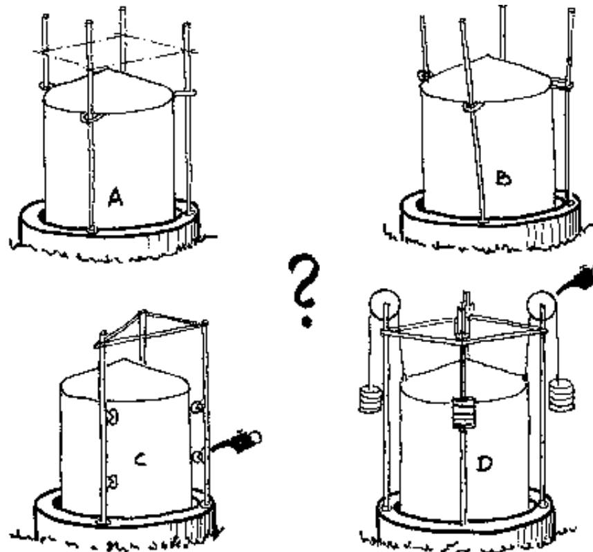
Fig. 32: Unsuitable guidance systems for floating drums With these guides, the gas drum cannot be rotated. This means that floating scum cannot be broken up. The rollers and bearings must be lubricated. In arrangement (C), the paintwork of the drum is damaged. Plant (B) is jammed if only one of the guide rods is not vertical. A central guide tube is always better!
