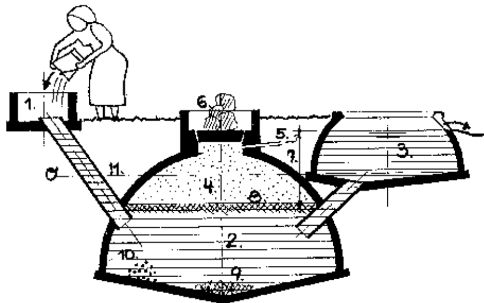
Fig. 4: Fixed-dome plant 1. Mixing tank with inlet pipe. 2. Digester. 3. Compensating and removal tank. 4. Gasholder. 5. Gaspipe. 6. Entry hatch, with gaslight seal and weighted. 7. Difference in level = gas pressure in cm WC. 8. Supernatant scum; broken up by varying level. 9. Accumulation of thick sludge. 10. Accumulation of grit and stones. 11. Zero line: filling height without gas pressure.
