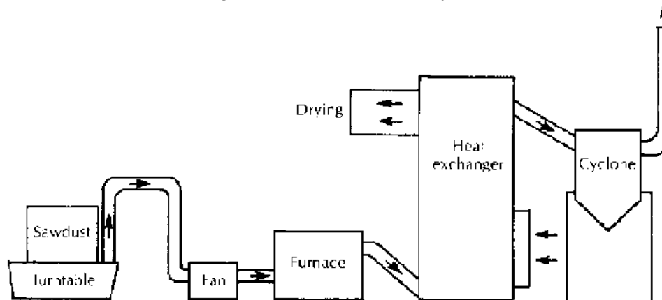
Figure 1 Diagram of the experimental system
