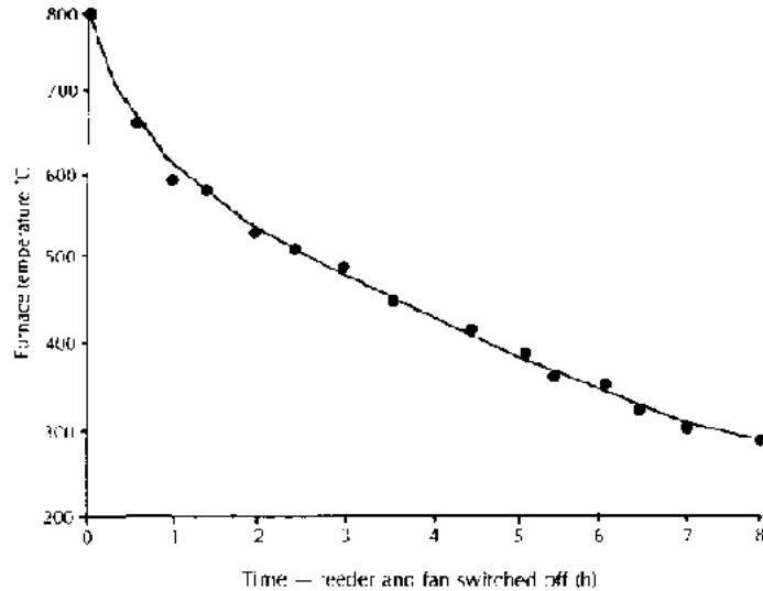
Figure 3 Furnace cooling curve
