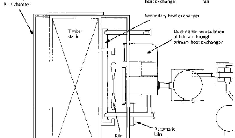
Cross section through unit
