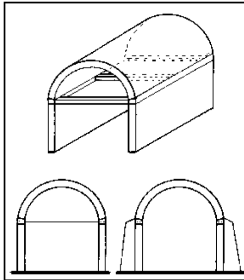
15-1 Ring beams stabilized by tensors or buttresses
