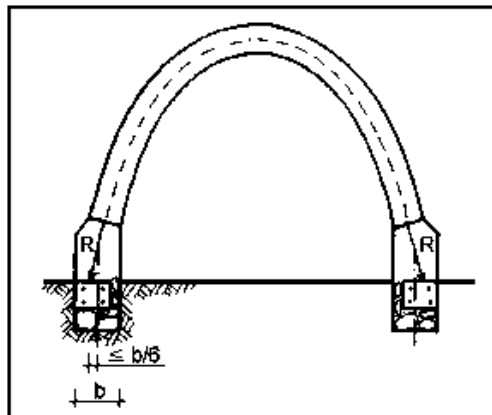
15-2 Permitted eccentricity
