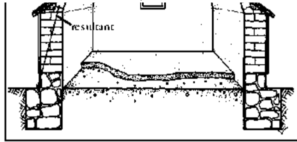
15-4 Badly designed plinth with eccentric thrust line
