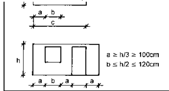
13-5 Recommendable dimensions of openings
