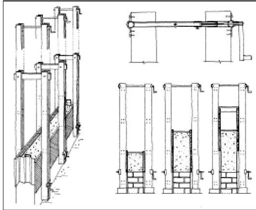
6-4 Climbing formwork (Minke 2000)
