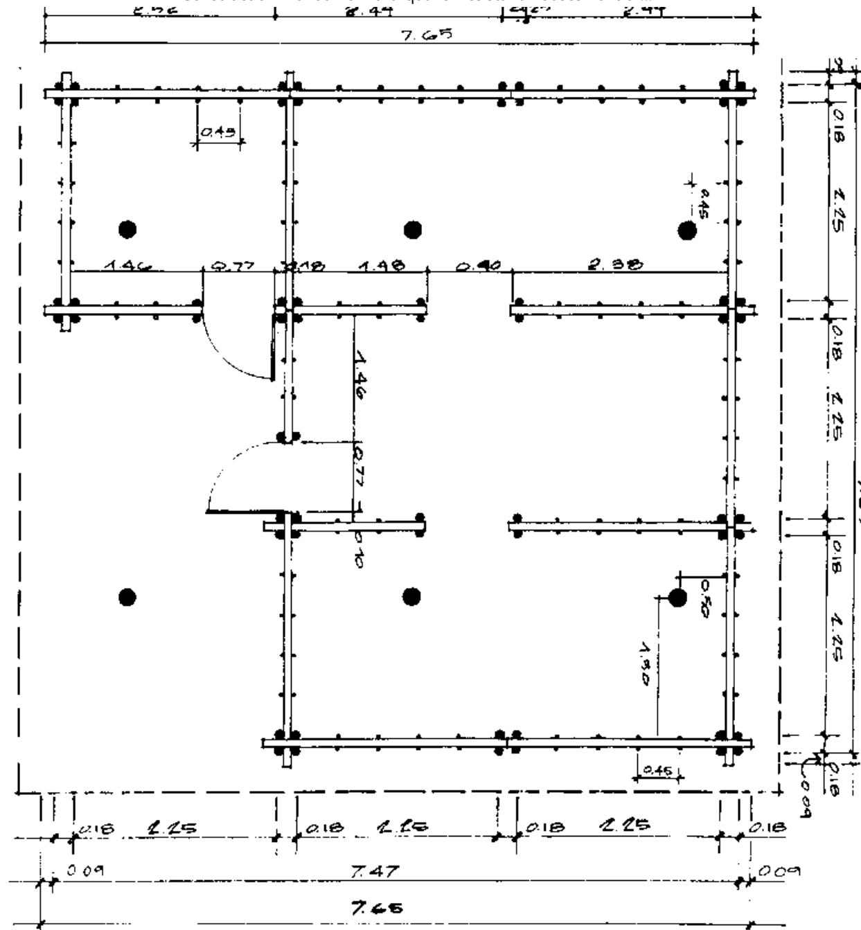
9-8 Earthquake resistant low-cost housing prototype, Guatemala 1978
