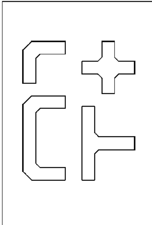
6-9 Elements with correct corner details
