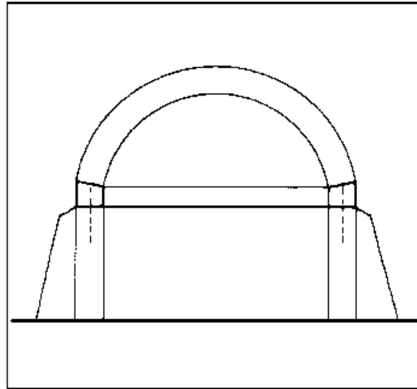
14-3 Ring beam stabilized by buttresses
