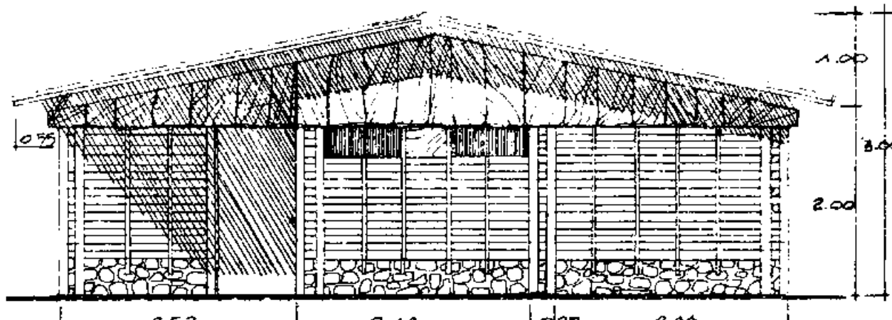
9-7 Earthquake resistant low-cost housing prototype, Guatemala 1978
