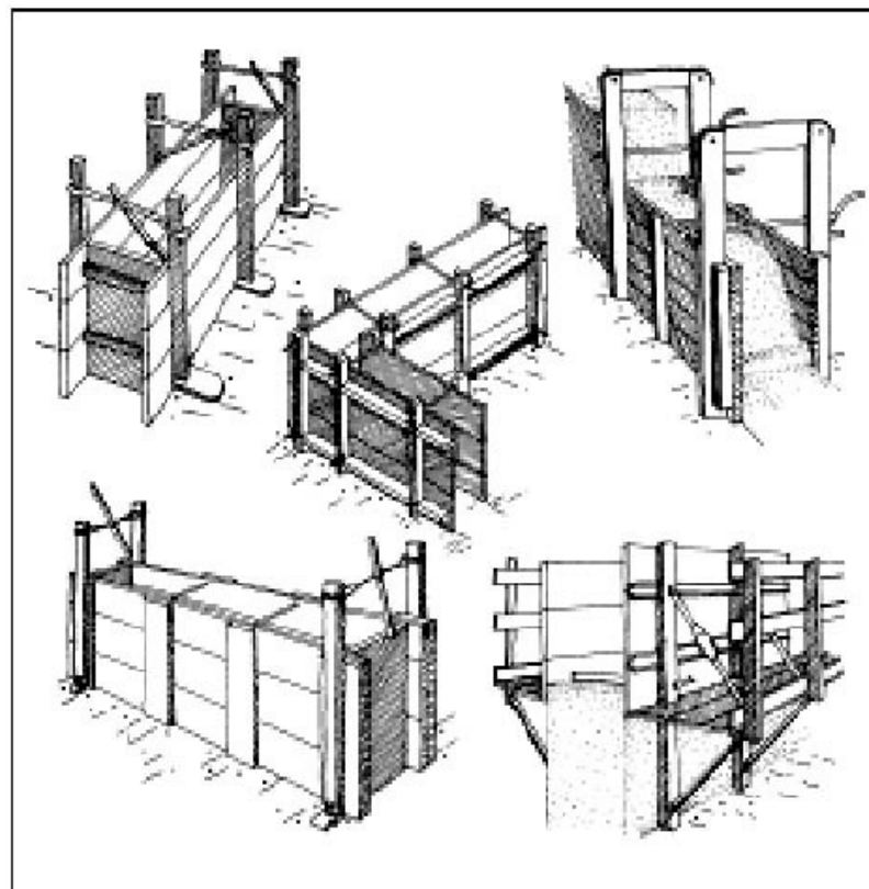
6-3 Formwork for rammed earth (Minke 2000)
