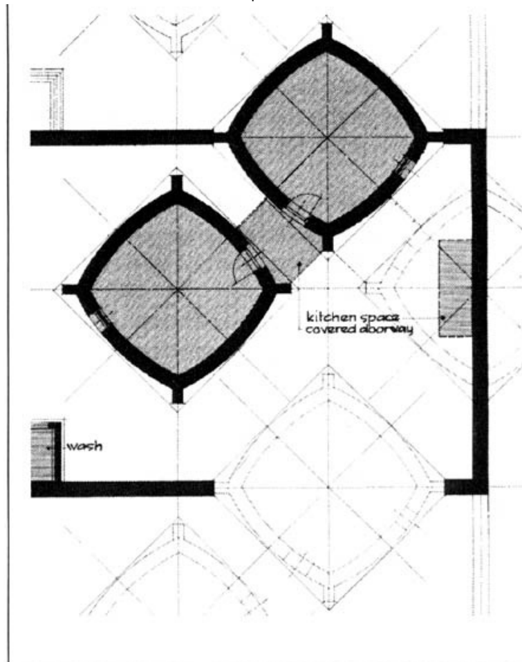
3-9 Plan of seismic-resistant houses, Afghanistan (Sibtain 1982)
