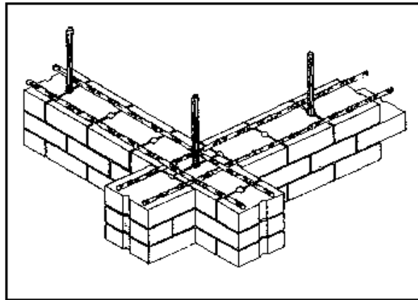
7-5 System ININVI, Peru
