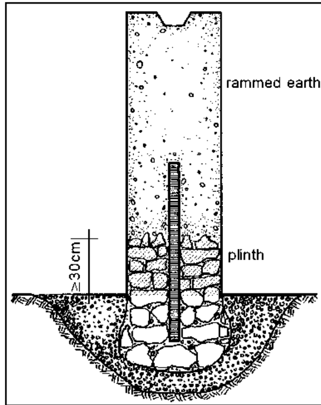
10-3 Floating foundation
