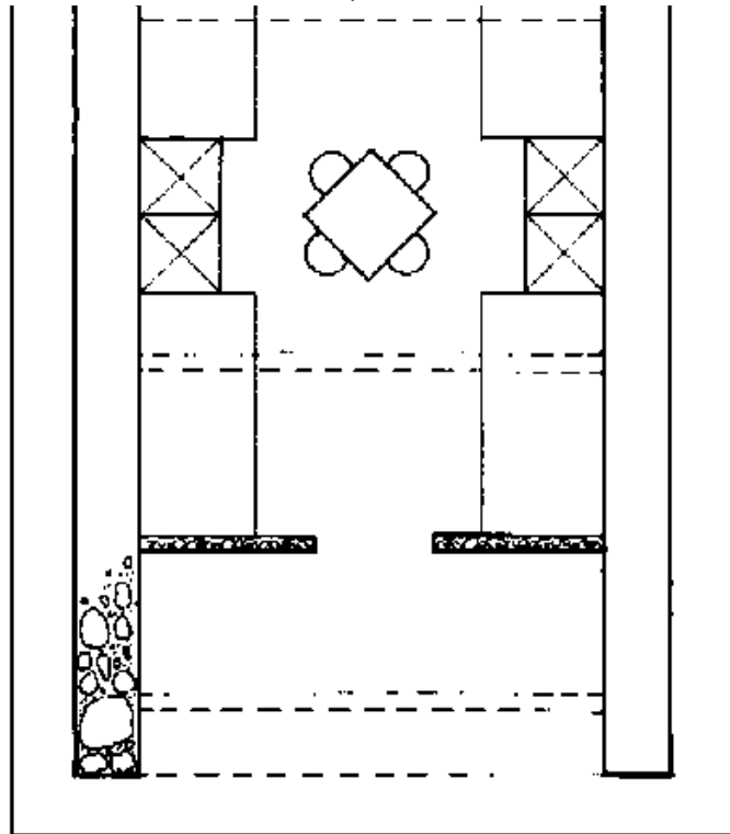
15-5 Proposal for an earthquake resistant vault structure for India
