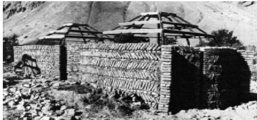
4-4 Earthquake-proof houses, Afghanistan (Sibtain 1982)
