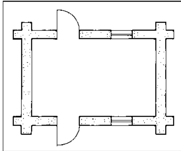
13-6 Recommendable positions of openings
