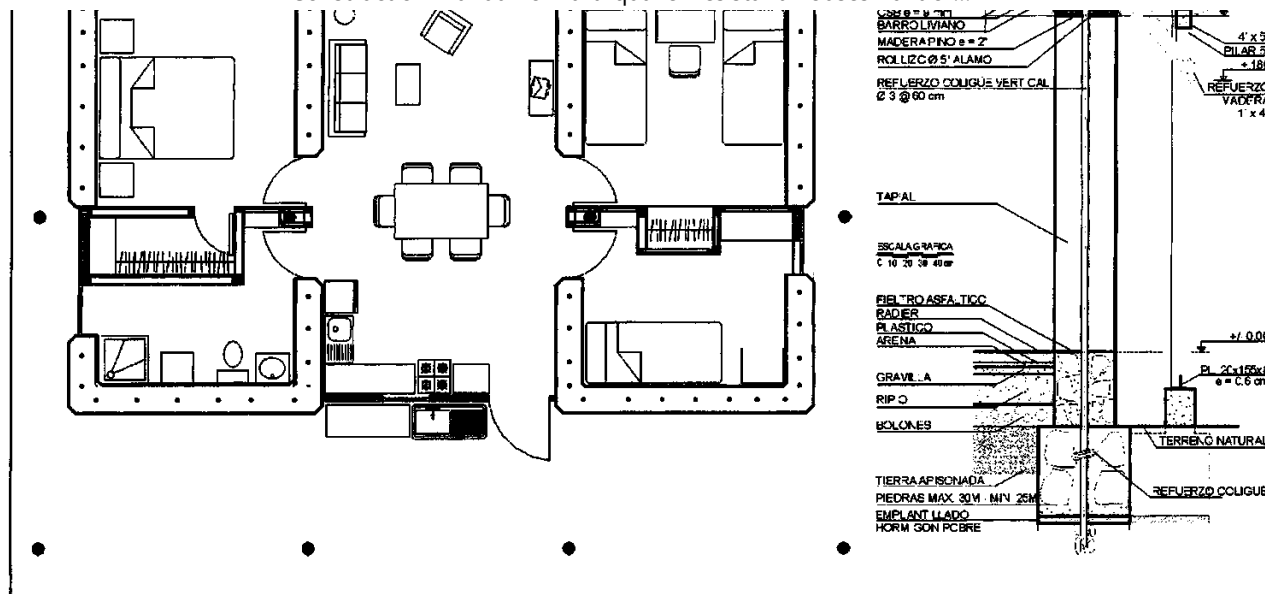
6-20 and 6-21 Earthquake resistant prototype building, Alhué, Chile 2001
