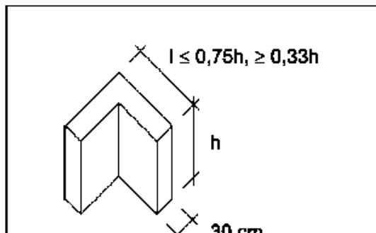
6-5 Wall elements stabilized by their shape
