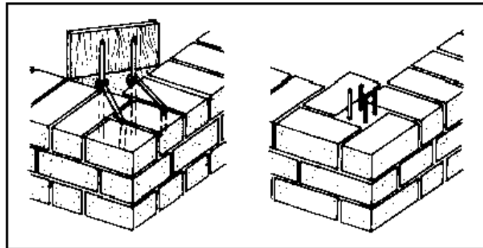
7-10 Stabilized corners
