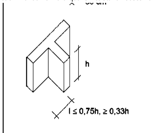
6-6 Recommended proportions
