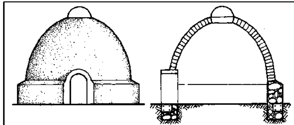
14-4 Stabilization of dome entrance
