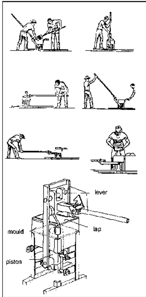
7-3 CINVA-Ram, Colombia
