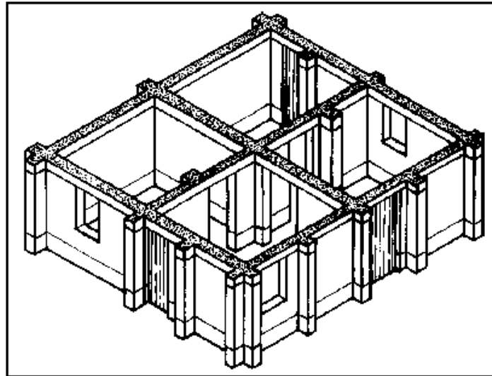
7-9 Adobe walls reinforced by butresses
