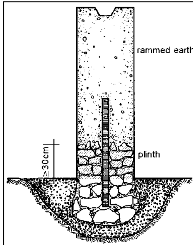
10-3 Floating foundation
