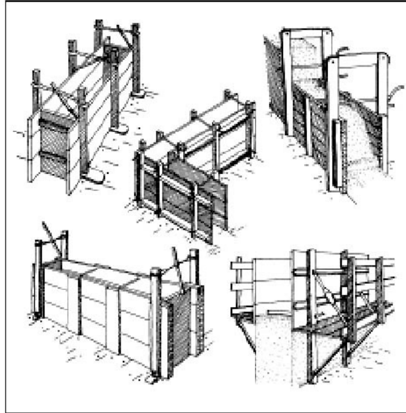
6-3 Formwork for rammed earth (Minke 2000)
