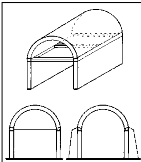
15-1 Ring beams stabilized by tensors or buttresses
