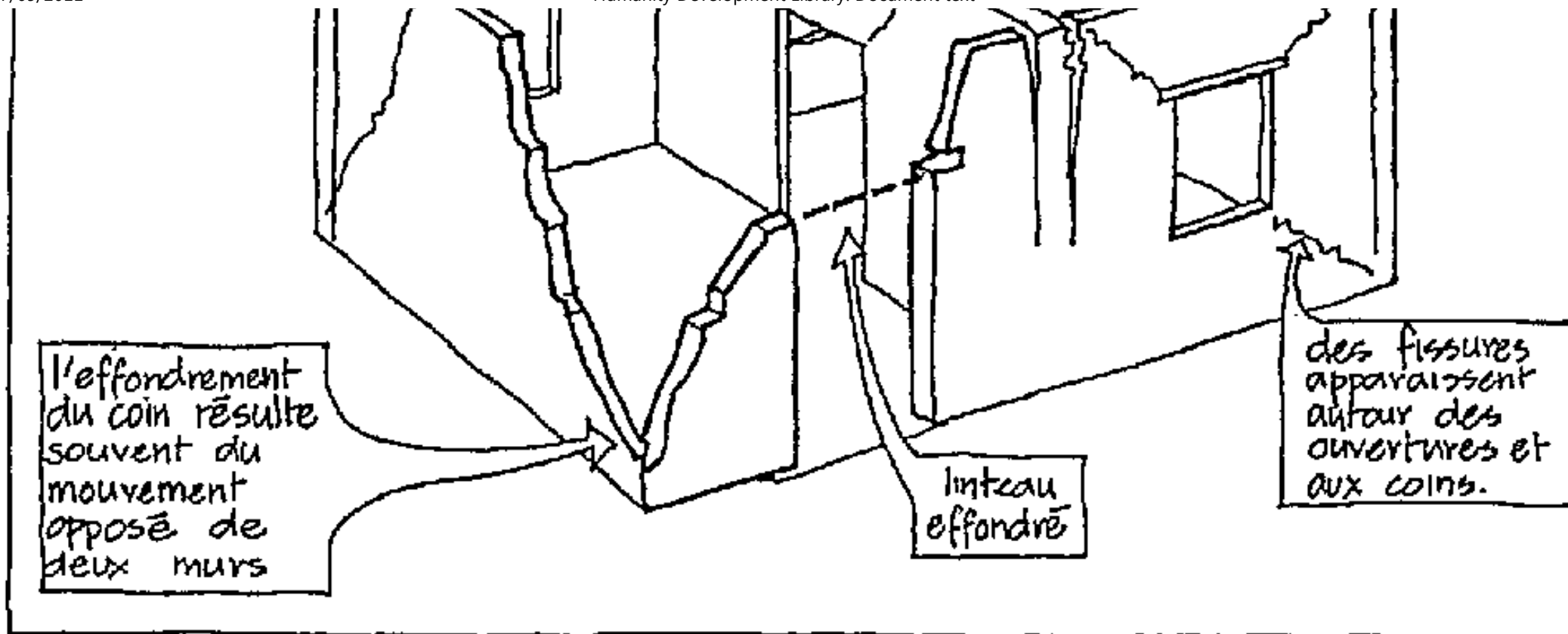
Typical earthquake effects and damage (drawings by John Norton, Bibl. 25.10)
