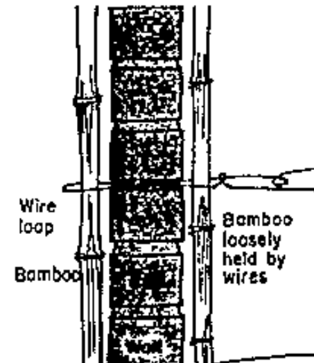
Bamboo tightened by pulling on short sticks attached to wire ends
