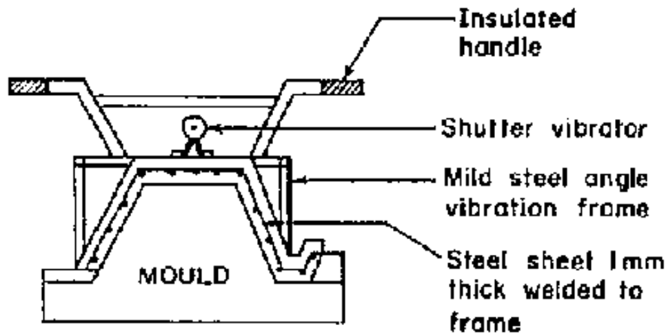
SERC vibration frame placed on mould
