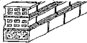
BEAM INTEGRATED IN A CAST-IN-PLACE FLOOR SLAB
