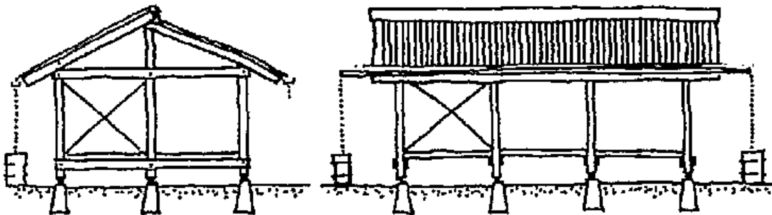
FRAME - CONSTRUCTION
