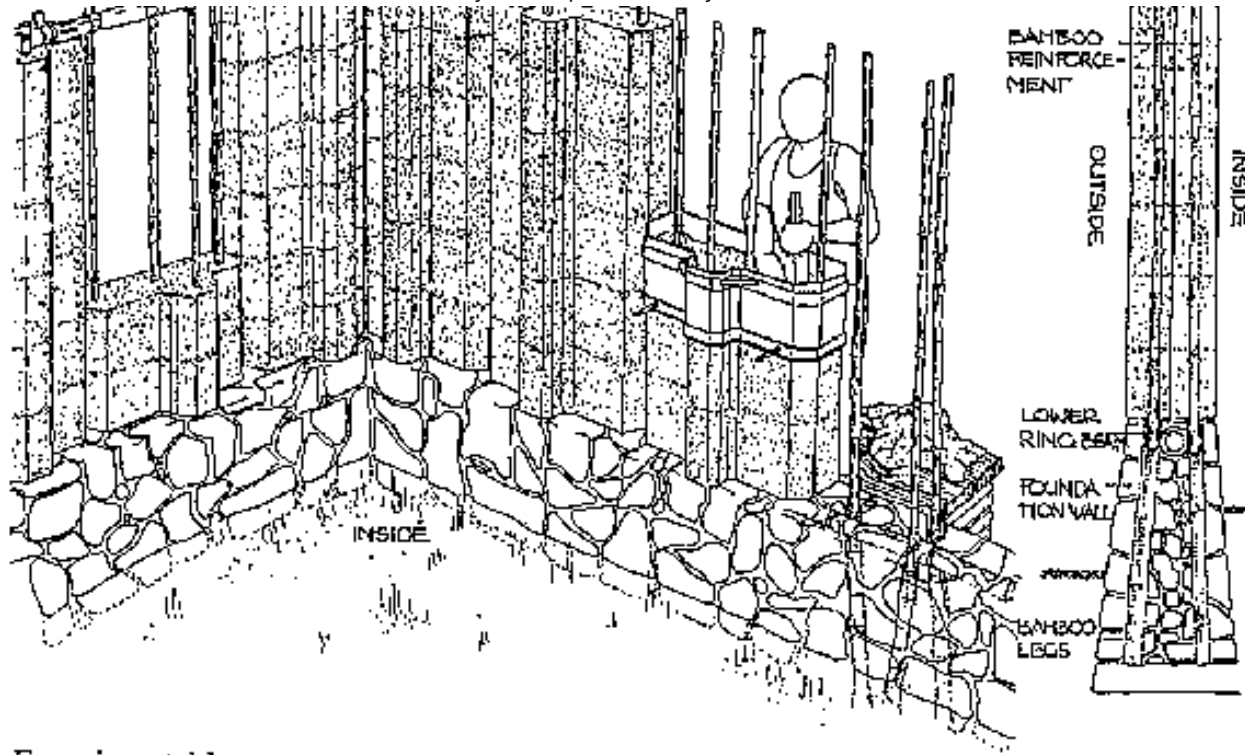
Experimental low-cost earthquake resistant house in Guatemala (top: Bibl. 22.09; bottom: Bibl. 22.05)
