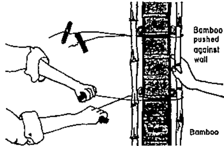
Bamboo tightened by pulling on short sticks attached to wire ends
