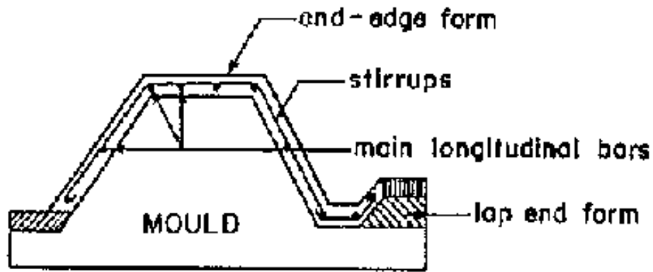
Cross-section showing cage preparation
