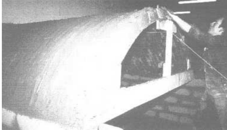
Building a barrel vault in "slices"
