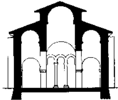
Section of church, Valladolid, Spain
