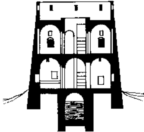
Section of house in Sfax, Tunisia
