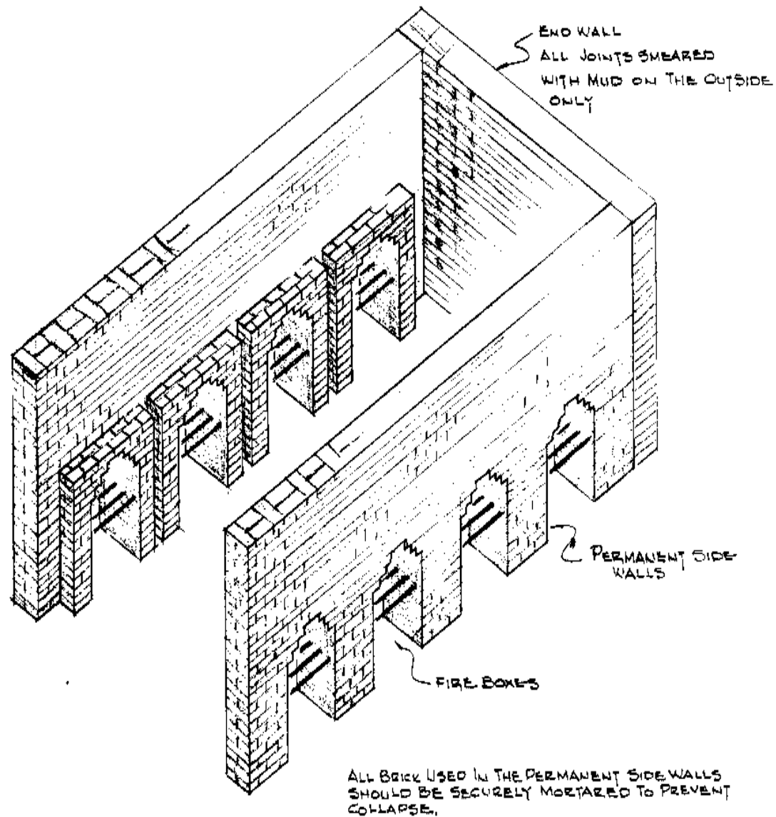
ILLUSTRATION N o 5 PERMANENT SIDE WALLS OF KILN - SHOWN WITH ONE END WALL
