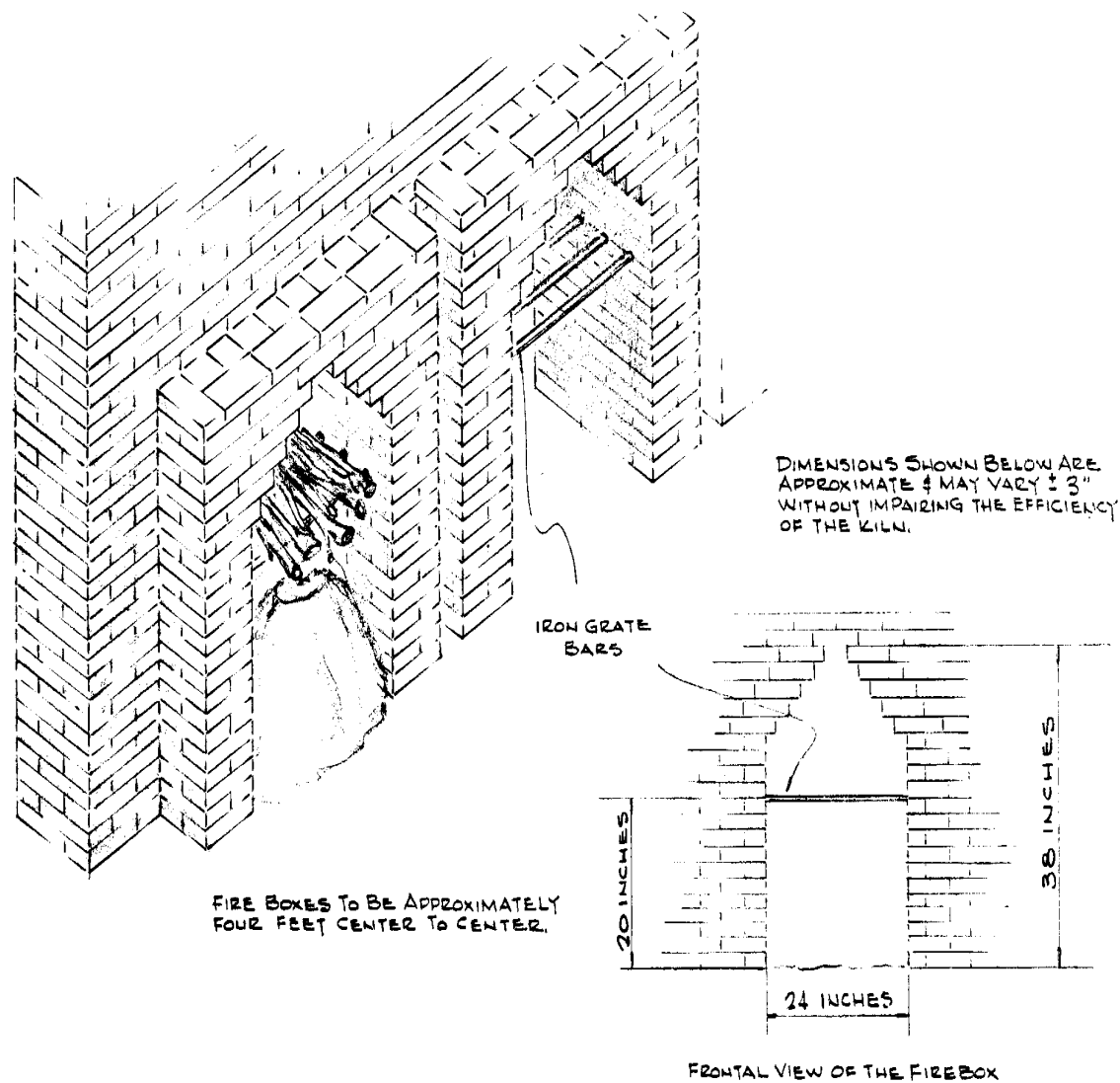
ILLUSTRATION N o 4 - VIEW OF FIREBOX. NOTE THAT THE FIREBOX EXTENDS ABOUT 10 INCHES INTO THE BRICK SETTING AREA.
