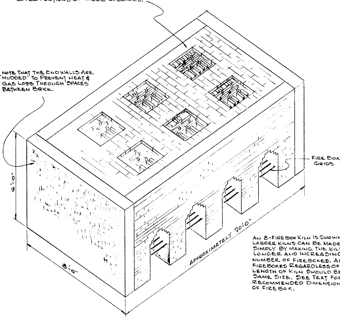
ILLUSTRATION N o 6 EIGHT - FIREBOX KILN
