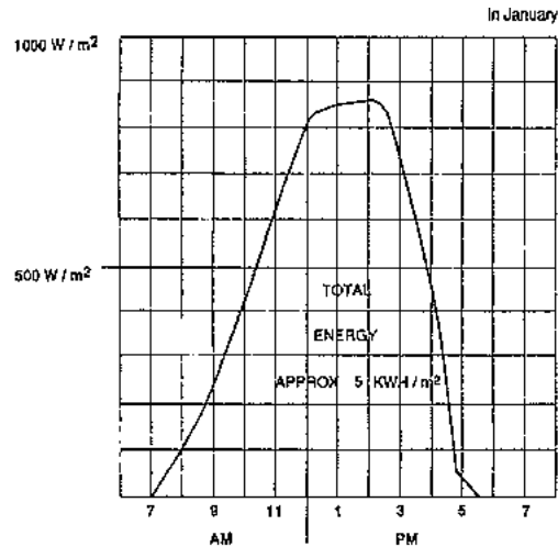
Fig 2/6 Sun intensity on a south-facing, inclined surface in January during a clear day, latitude 27° North
