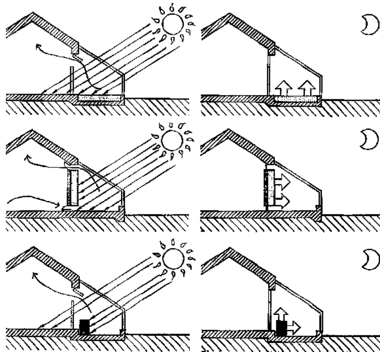
Fig 3/172 Solar gain by attached greenhouse shown during day and night function
