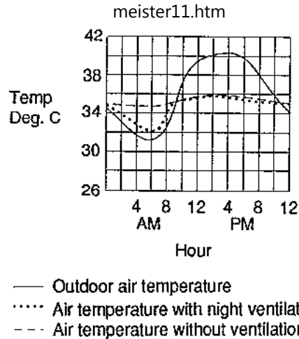
Fig 4/2 Influence of increased night ventilation, measured air temperatures in the middle of the rooms
