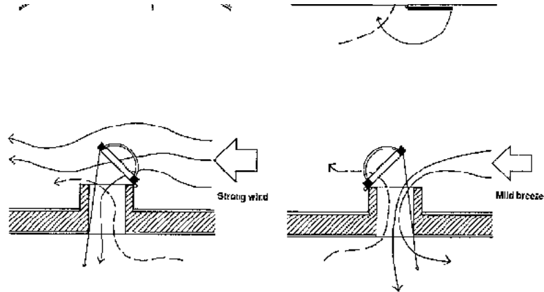
Fig 3/78 Examples of devices using external winds
