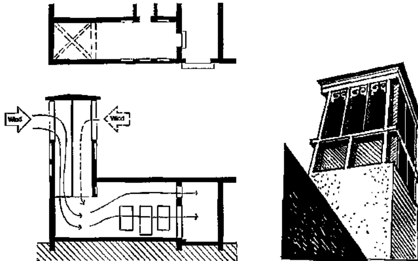
Fig 3/115 Multi-directional roof windcatcher (-tower); plan, section and perspective view
