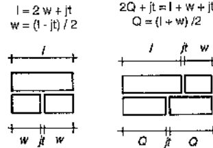
THICKNESS OF THE MORTAR JOINT (jt) (FIG.48)
