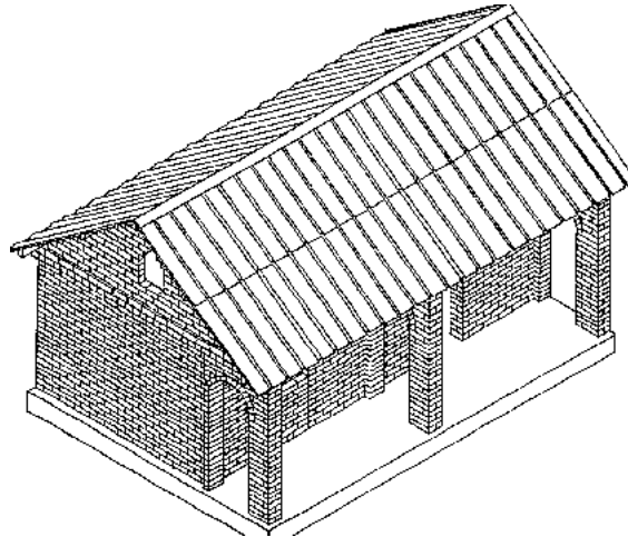
Fig. 205: Roof covering of galvanized steel roofing sheets with peripheral overhang.
