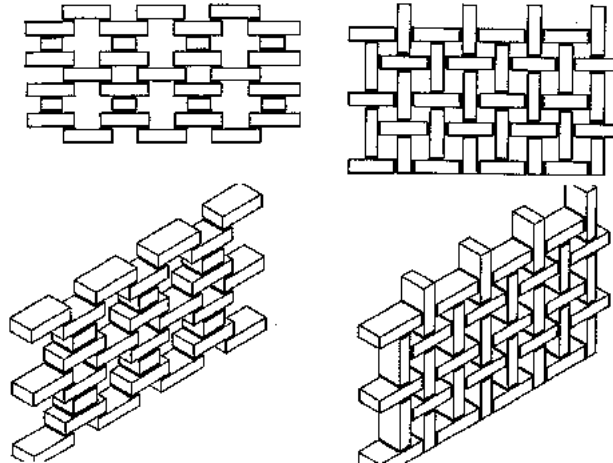
Fig. 158: Simple claustra-work designs with criss-cross motifs (full and half blocks) or the woven effect of stretchers with vertical blocks.
