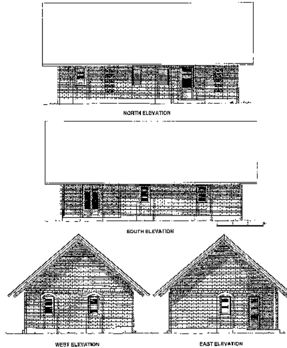
Fig. 281: Elevations of the four elevations of the T4 type single-storey house.
