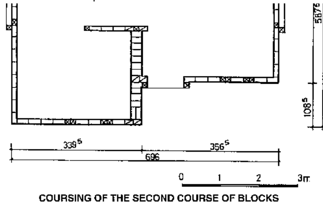
Fig. 265: Coursing of the bonding of the CEBs for the wall masonry of the ground floor. First course (top plan), second course (bottom plan).
