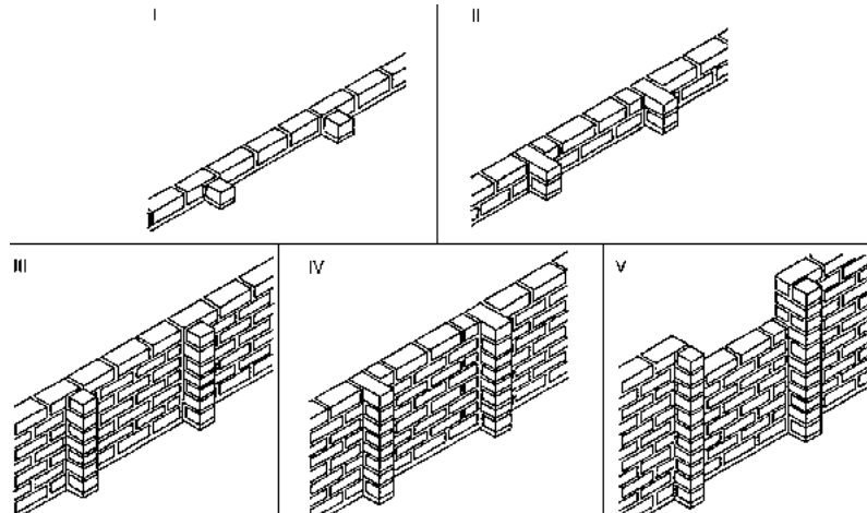
Fig. 217: Building an independent window-breast using alternately full and half-blocks (sequence I to V).
