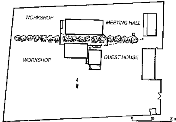
Fig. 284: Site plan for the project as a whole.
