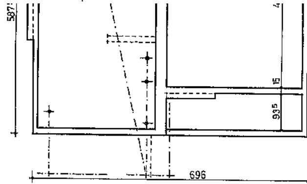
Fig. 263: Plans of foundations. Above, blinding concrete poured into gullies on which rests a reinforced concrete ground beam (lower plan).
