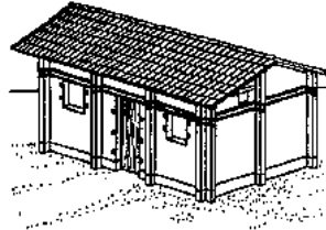
Fig. 119: Thin walls, buttresses and reinforcement.
