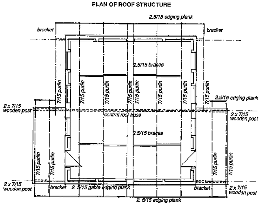
Fig. 312: Plan of roof structure detailing the wood sections and the principle of horizontal wind-bracing by bridging the purlins.
