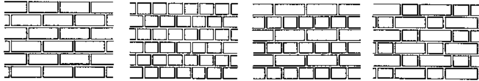
Fig. 45: Fundamental rules of bonding patterns to avoid superimposed vertical joints. (A;B;C;D)
