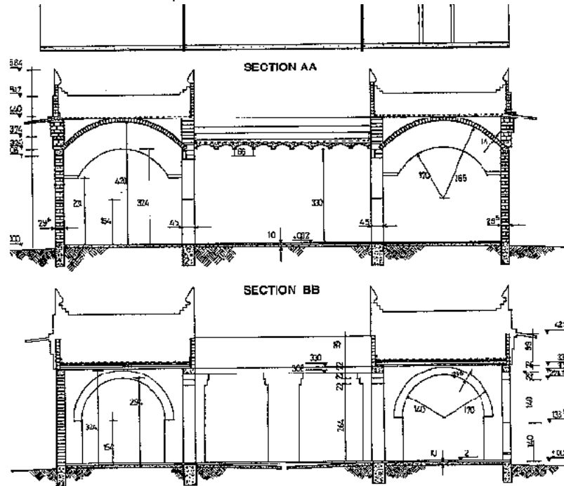
Fig. 320: Elevation of pavilion elevations and sections of exhibition galleries (M) and courtyard (BB) showing the use of flat and domed roofs.
