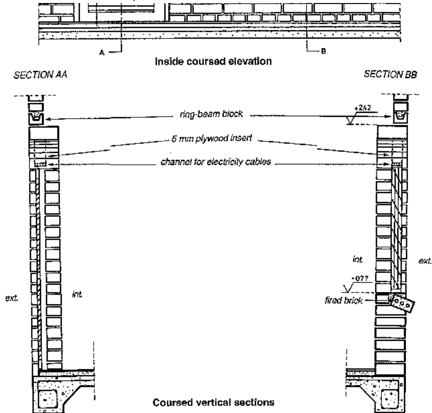
Fig. 68: Example of vertical coursed of a faade and of vertical sections of a wall with openings.
