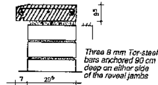
WINDOW-SILL
