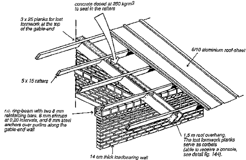
Fig. 145: Housing protect, Cameroon. Anchoring of rafters into the gable-end wall using a concrete seal poured at the top of the wall in a lost formwork made of planks.
