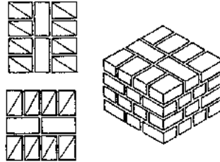
Fig. 61 c: Classic bonding pattern for a 60 × 60 cm pillar.
