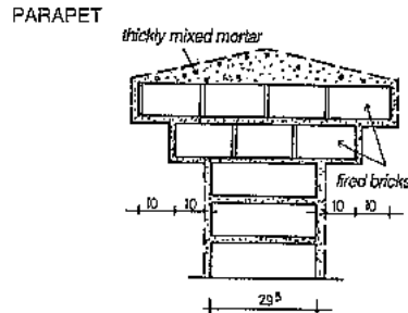
Fig. 247: Detail of the cornice of the parapet with its fired brick corbelling.
