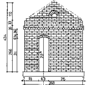
RIGHT-HAND GABLE WALL
