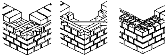
Fig. 122: Ring-beams of mesh embedded in the mortar or in reinforced concrete.
