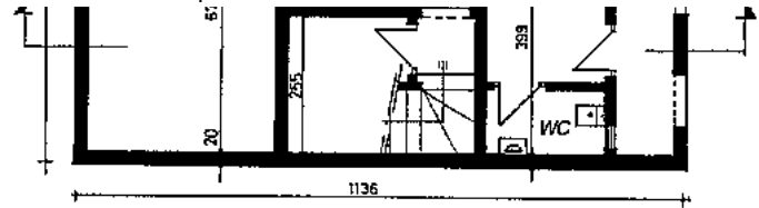
GROUND-FLOOR PLAN
