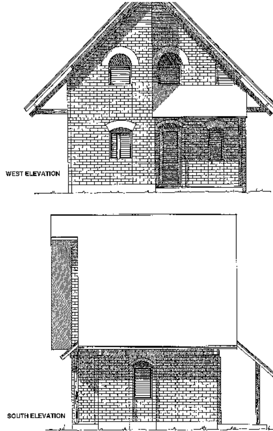
Fig. 262: West and south elevations: access to the main elevation is by a small stepped verandah.
