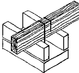
Fig. 272: Detail of systems for anchoring joists into the wall masonry.
