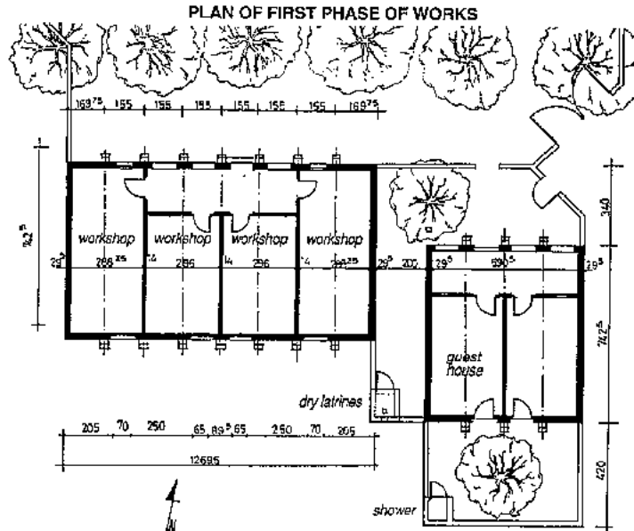
Fig. 285: Plan of first phase of work: guest house and first workshop block.
