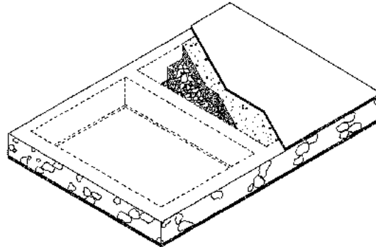
Fig. 198: Infilling the footings using the waste material from sifting gravel.
