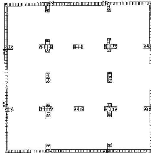
Fig. 324: Coursing of wall bonding patterns and arch and cupola pillars, for even number courses.
