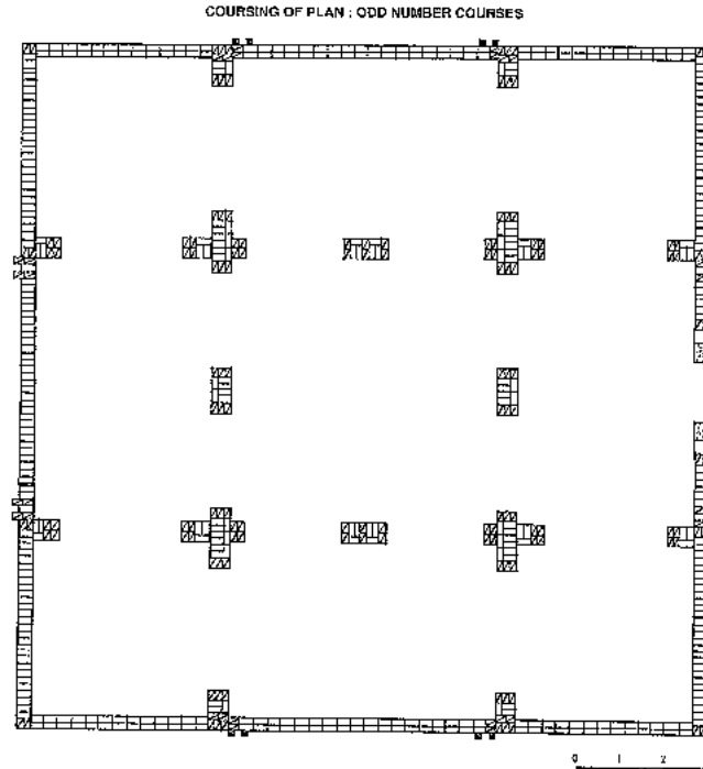
Fig. 321: Coursing of wall bonding patterns and arch and cupola pillars, for odd number courses.
