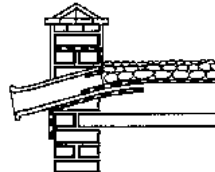
Fig. 146: Detail of water-proofing between roof/ parapet and roof/wall. Note the flexible system of laying of beams into the wall with insulation (thermal bridge) and waterproofing of the receiving base.
