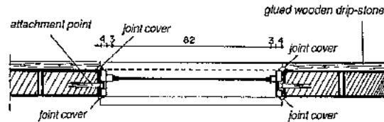
Fig. 279: Detail of system of attachment using metal elements in the mortar.
