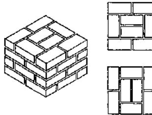
Fig 61 b: Simplified bonding pattern for a 60 × 60 cm pillar.
