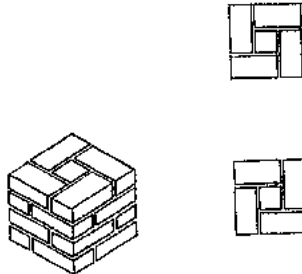
Fig 61 b: Simplified bonding pattern for a 45 × 45 cm pillar.
