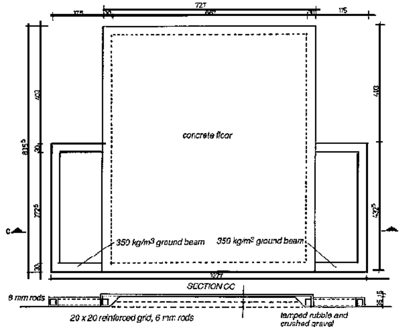
Fig. 303: Plan of foundations using compacted infill and reinforced concrete peripheral ground beams.
