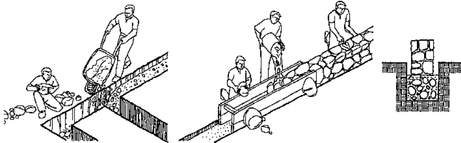
Fig. 94: The use of cyclopean concrete for foundations and footings is an attractive solution from the technical and economic point of view.
