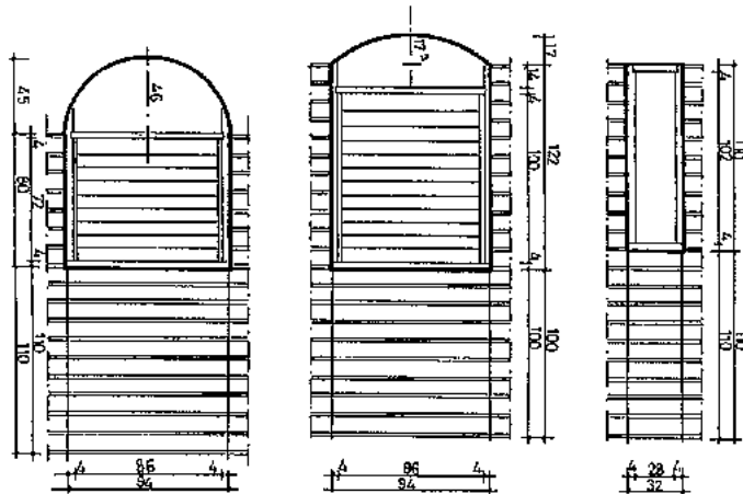
TYPES OF DOORS AND THEIR ARCHES
