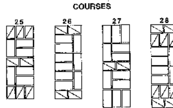
Fig. 323 b: Bonding pattern of corbel.
