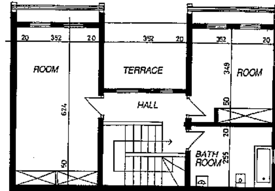
Fig. 234: Plan of house built in vibration-compacted blocks measuring 40 × 20 × 20 cm.
