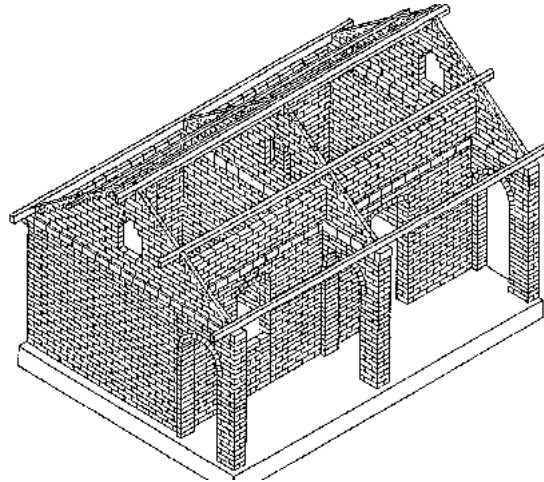
Fig. 204: Laying the purlins from gable wall to gable wall.
