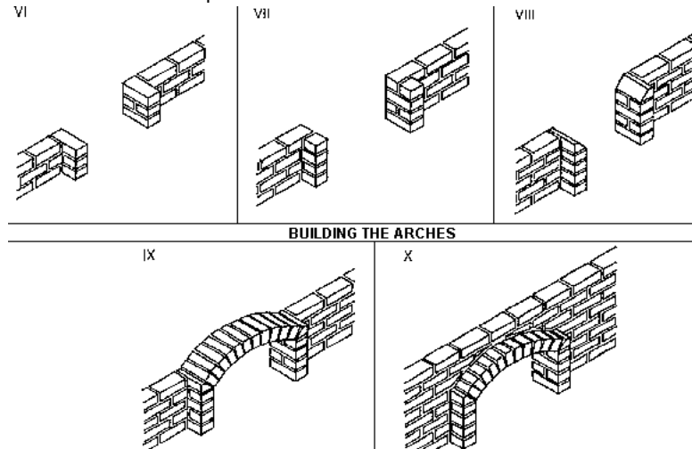
Fig. 218: Building the buttressed reveals of the openings. Note the thickness of the arch on the outside.
