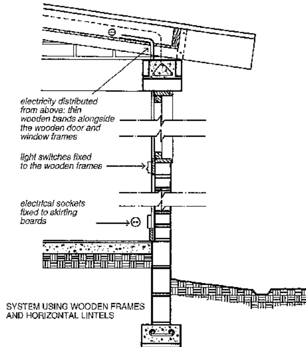
Fig. 170: Vertical sections showing the integration of the electrical network alongside the woodwork and skirting boards.
