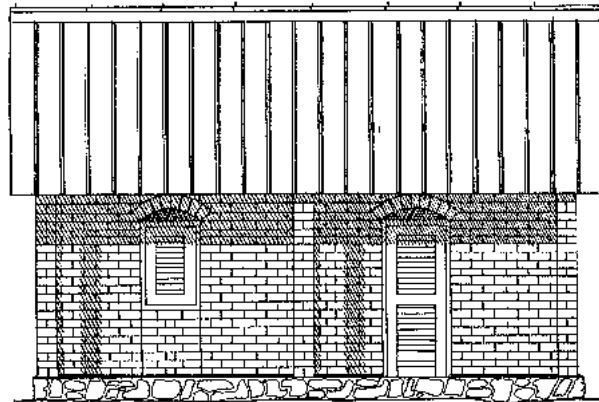
Fig. 194: Main elevation with verandah.
