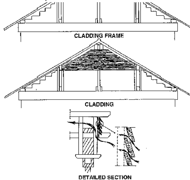
Fig. 225: Elevation and sections of the bracket anchoring system of the roof covering and of the cladding ventilation system.
