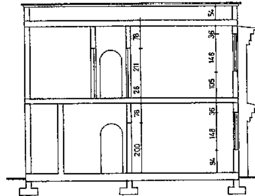
Fig. 243: Elevation and section of house built from compressed earth blocks measuring 29.5 × 14 × 9 cm.
