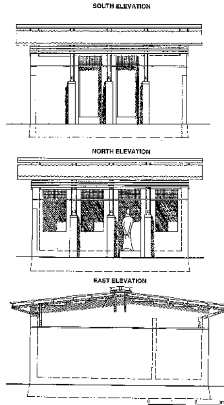
Fig. 288: Elevation of elevations of guest house.
