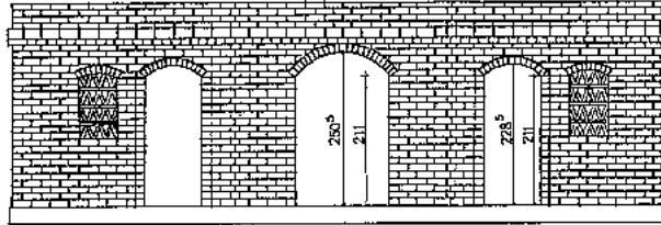
OUTWARD SIDE ELEVATION
