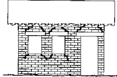
Fig. 100: Avoid too many openings in any one wall.
