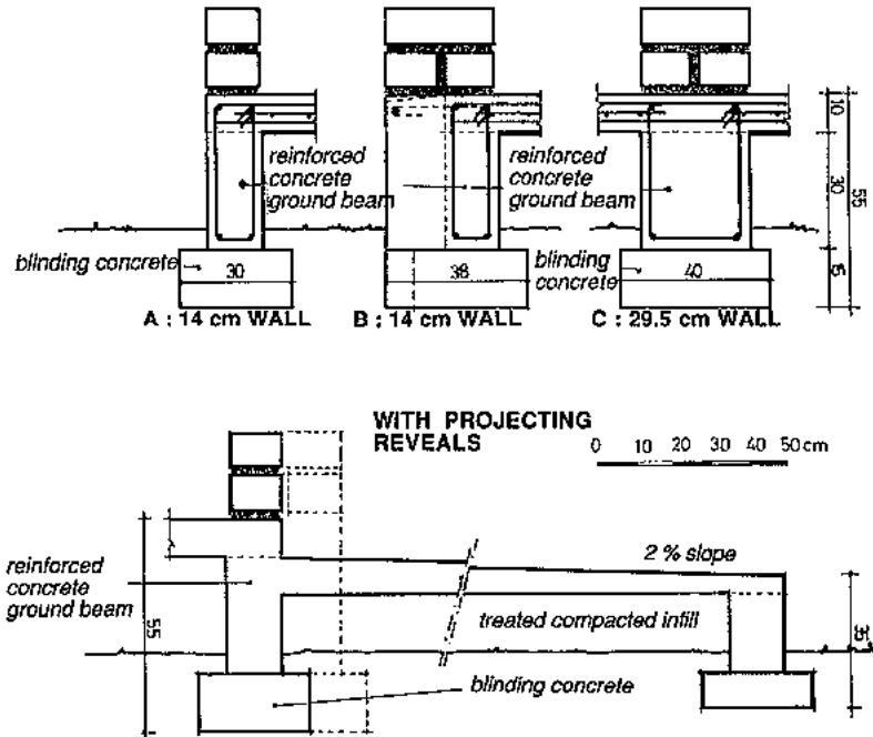
Fig. 264: Types of foundations and their variations depending on the thickness of the walls and the principle of a pavement over compacted.
