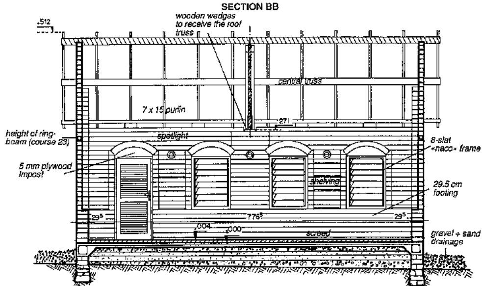
Fig. 311: Longitudinal section of classroom. Note the principle of a median roof truss end purlins resting on the gables.
