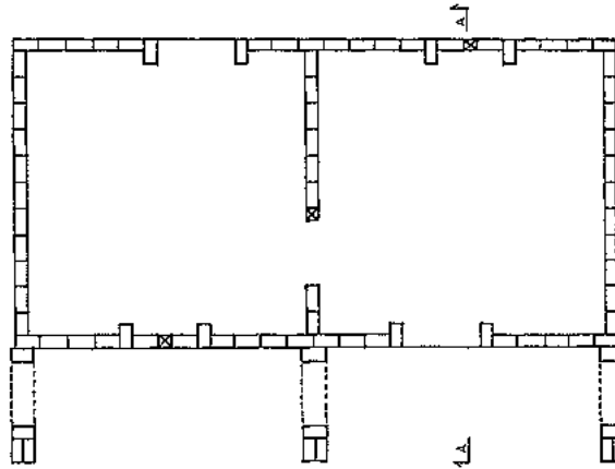
Fig. 192: Bonding pattern for the first course of compressed earth blocks.
