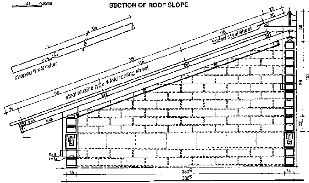
Fig. 141: Ruralhouse, Afatobo, Ivory Coast. Design by CRATerre, S. Maini. A double sloping roof of steels heets rests on a roof-structure of rafters. These are attached to the masonry of the gutter walls, at the lower side, under a ring-beam made of special sand-cement blocks used as lost formwork, by a stainless steel tie-beam linked to the roof rafter and on one section of rafter passing through the masonry, under the ring-beam. At the top, a ridge ventilator is itself fixed to the partition wan using the same principle.
