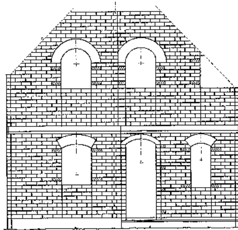
Fig. 273: Coursing of elevations for accurate openings.
