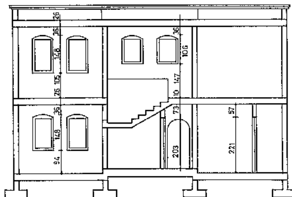
Fig. 237: Elevation and section M of house made from vibration-compacted blocks measuring 40 × 20 × 20 cm.
