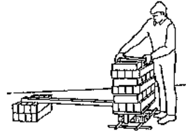
Fig. 171: Block-breaking equipment to test bending strength.
