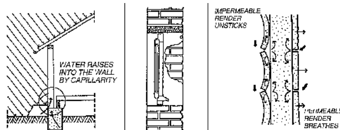
EXAMPLES OF HUMIDITY PROBLEMS (FIG.74;75;76)
