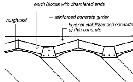
Fig. 128: Chamfered earth block, easier to lay.
