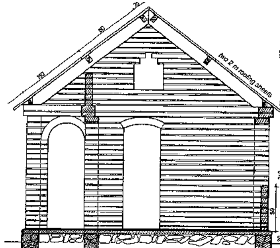
Fig. 196: Section AA figs. 192 and 193. Note the arches: semi-circular (verandah), Dutch (doors and windows), and corbel (upper ventilation of the gable-end).
