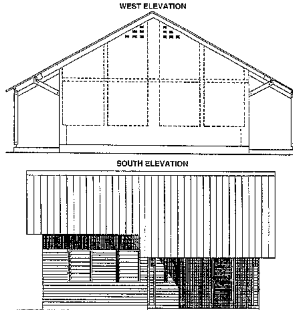
Fig. 309: Elevation of gable-end elevation and main elevation of classroom.
