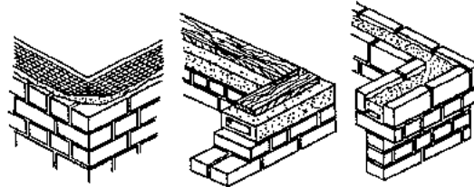
Fig. 120: Ring-beams and reinforced comers using wood or steel embedded in the wall.
