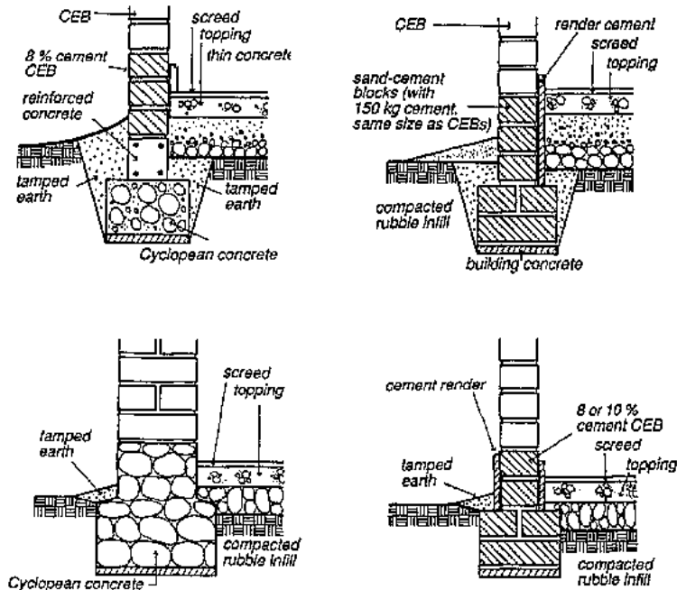
Fig. 90: Several examples of how to treat a humidity risk resulting from infiltration without accumulation.
