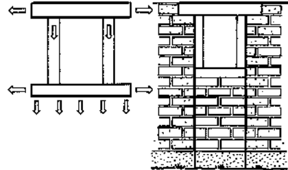
Fig. 104: Well dimensioned sill or independent breast.
