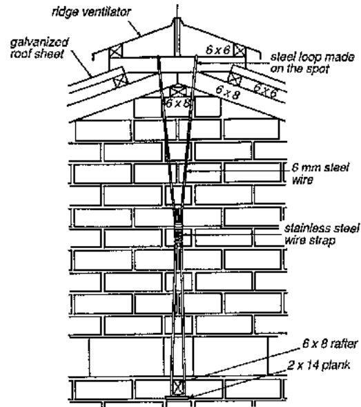
Fig. 143: Detail of fixing the ridge ventilator to the gable-end wall. The metal tie-beam is clipped to a section of the rafter crossing through the masonry, under the sand-cement ring-beam.
