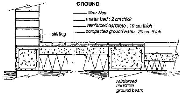
Fig. 327: Detail of working drawing for foundations.
