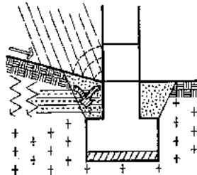
Fig. 88: Prolonged accumulation.
