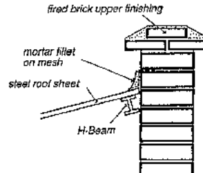
Fig. 138: Detail of joint between roof and acrotere.
