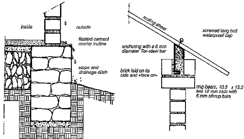
Fig. 197: Principle used for water runoff at the base of the wall and for anchoring the lower edge of the roof covering.
