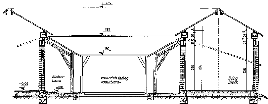
Fig. 215: Sections of type T3 and T4 houses, with verandahs facing "outwards" and
