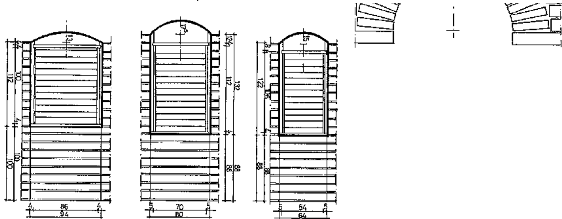
Fig. 277: Drawings of the complete range of door and window openings with Dutch or semi-circular arches.
