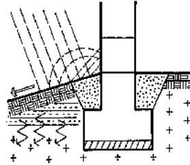
Fig. 87: Temporary accumulation.
