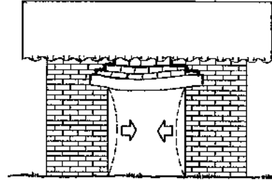
Fig. 98: Make sure the lintel is the correct size for wide openings.
