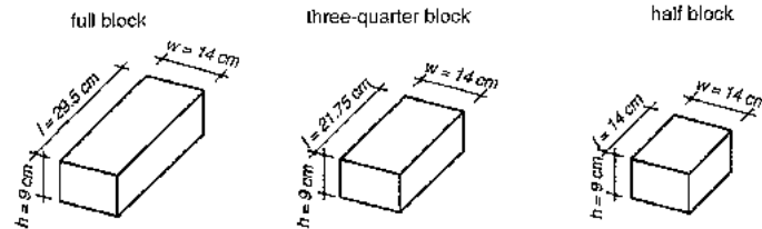
DIMENSIONS OF COMMON BLOCK AND DERIVATES (FIG.49)
