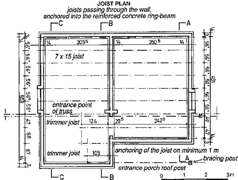
Fig. 270: Laying plan of floor joists.
