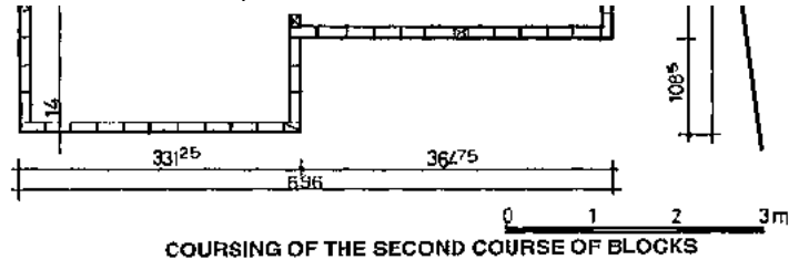
Fig. 268: Coursing the bonding patterns of the first floor walls. First course (top plan), second course (bottom plan).
