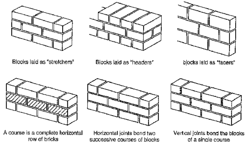
TERMINOLOGY FOR TYPES OF BONDING PATTERN (FIG.44)
