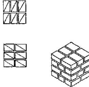
Fig. 61 a: Classic bonding pattern for a 45 × 45 cm pillar.
