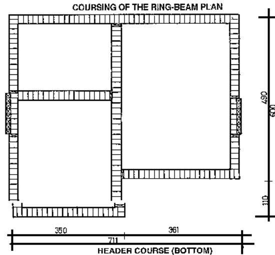
Fig. 266: Course of header blocks forming the bottom of the formwork for the ring-beam.
