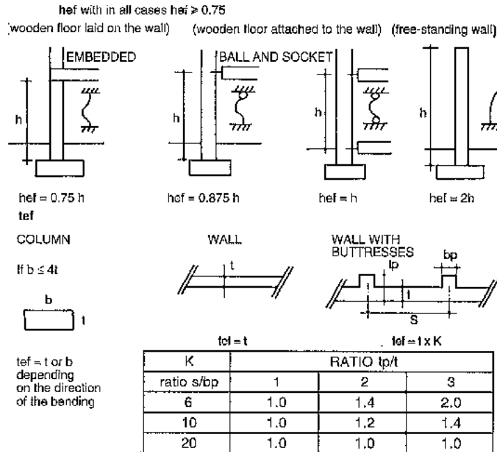
Fig. 173: Comparison of values of effective height and thickness for walls varying in design but sharing a common height and thickness.
