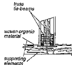
Fig. 293: bracing rafter of gable wall with false brackets for attaching to the wall.
