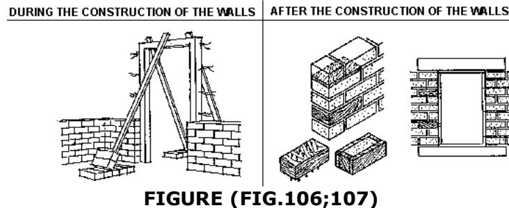
Fig. 106: Holding the door-frame in place as the walls are built up.
