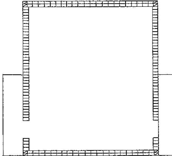
Fig. 304: Coursing of bonding pattern of the first four odd number courses 29.5 cm thick (footing).
