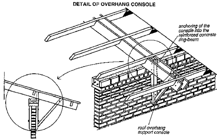
Fig. 144: Housing project, Cameroon. Design CRATerre, arch. P. Rollet and V. Rigassi. The anchoring of the lower side of the roof uses the principle of an overhang console with a bracket against the wall. On the outside, the bracket is itself attached to the ring-beam with a fixing Iron.
