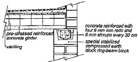
Fig. 325: Detail of ring-beam design.
