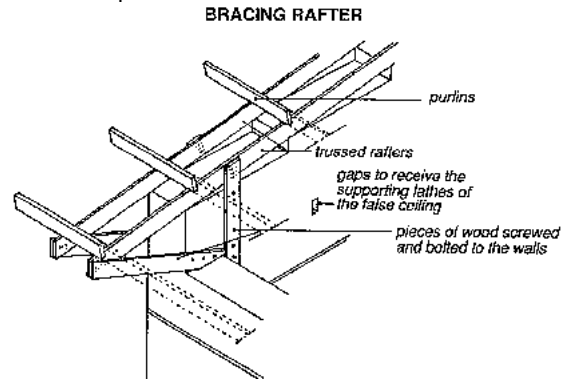
Fig. 292: Detail of support of false ceiling. The underface of the tie-beams of the different rafters of the roof structure enable small section supports for the false ceiling to be attached.
