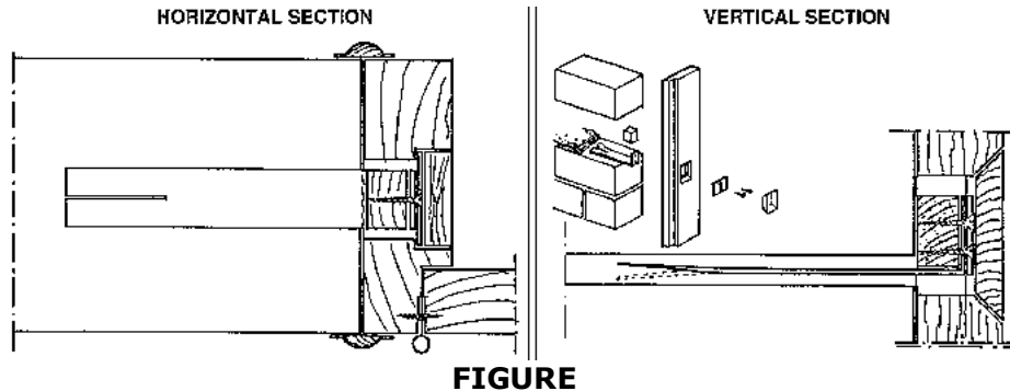
Fig. 279: Detail of system of attachment using metal elements in the mortar.
