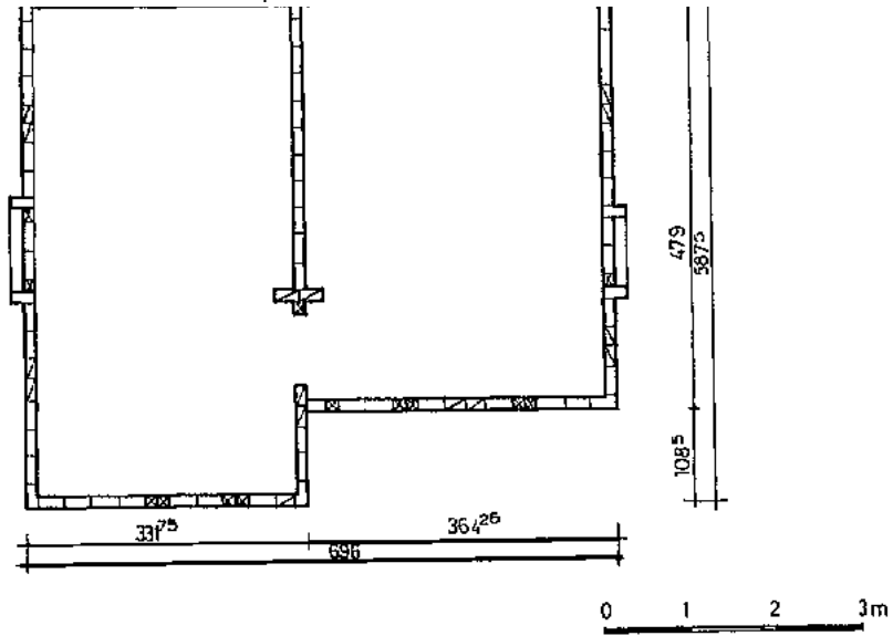
COURSING OF THE FIRST COURSE OF BLOCKS
