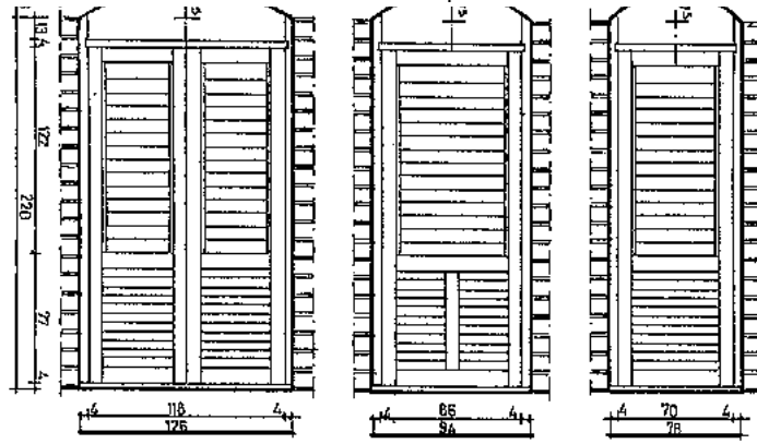
TYPES OF DOORS AND THEIR ARCHES
