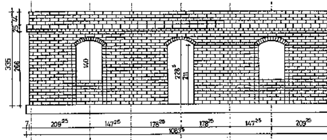
LEFT-HAND GABLE WALL
