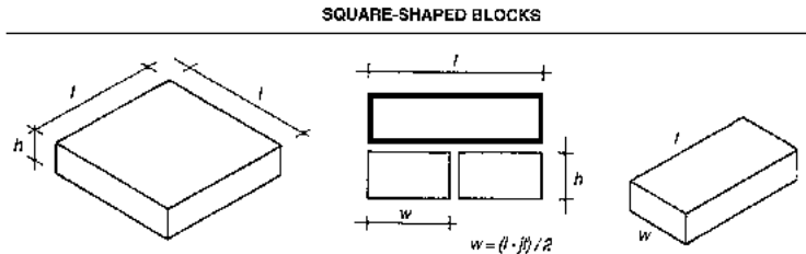
Fig. 62: Square block and half block obtained by cutting it down the middle.
