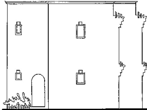
Fig. 243: Elevation and section of house built from compressed earth blocks measuring 29.5 × 14 × 9 cm.
