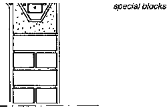
Fig. 332: Vertical section of the external wall from the ring-beam to the merlon.
