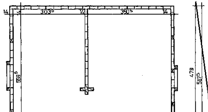
COURSING OF THE FIRST COURSE OF BLOCKS
