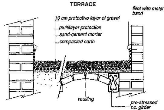
Fig. 326: Detail of water-proofing of flat roofs.
