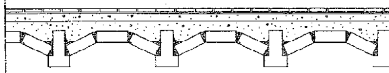
Fig. 249: Longitudinal section of the building principle of vaulting using reinforced concrete girders and compressed earth blocks.
