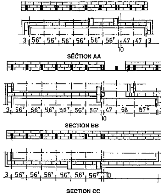
Fig. 271: Plans and detailed sections of layout of floor joists.
