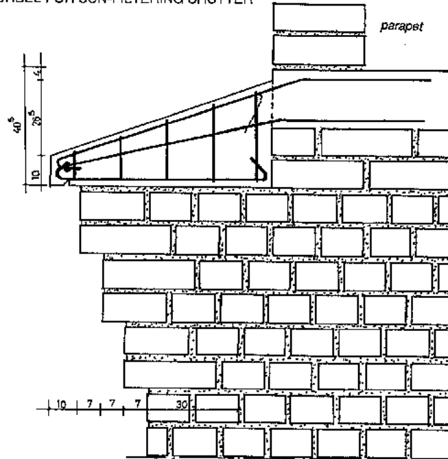
Fig. 248: Corbelling of the elevation with RC corbel for attachment of sun-filtering shutter.
