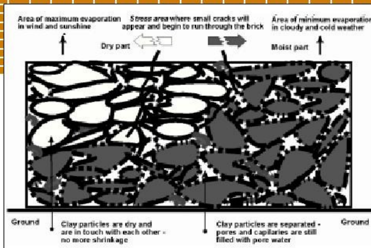
Fig. 3: Schematic drawing of "unbalanced" drying
