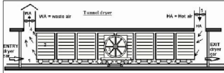
Fig. 11: Schematic drawing of artificial dryer: tunnel dryer with drying charge pushed on dryer cars through horizontal air flow
