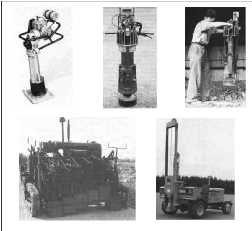
Figure 2.16 – Civil engineering compaction equipment using impact
