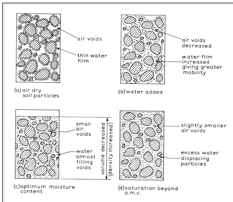
Figure 2.10 – Diagram of particle intimacy around the O.M.C.
