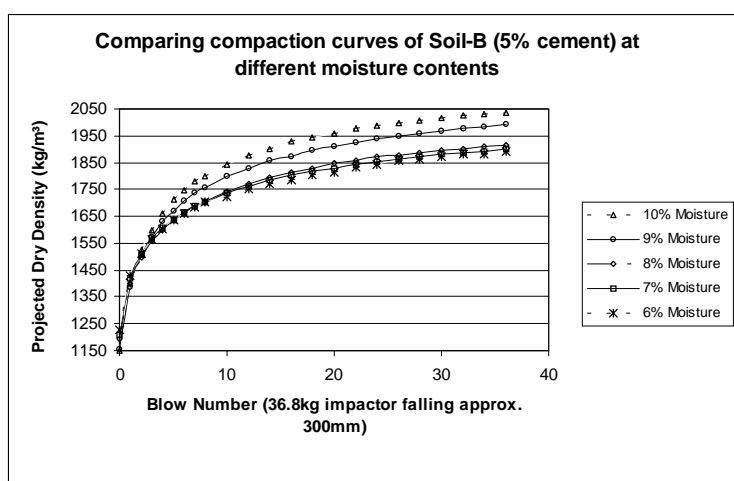
Figure 4.9 – Compaction curves of blocks at different moisture contents
