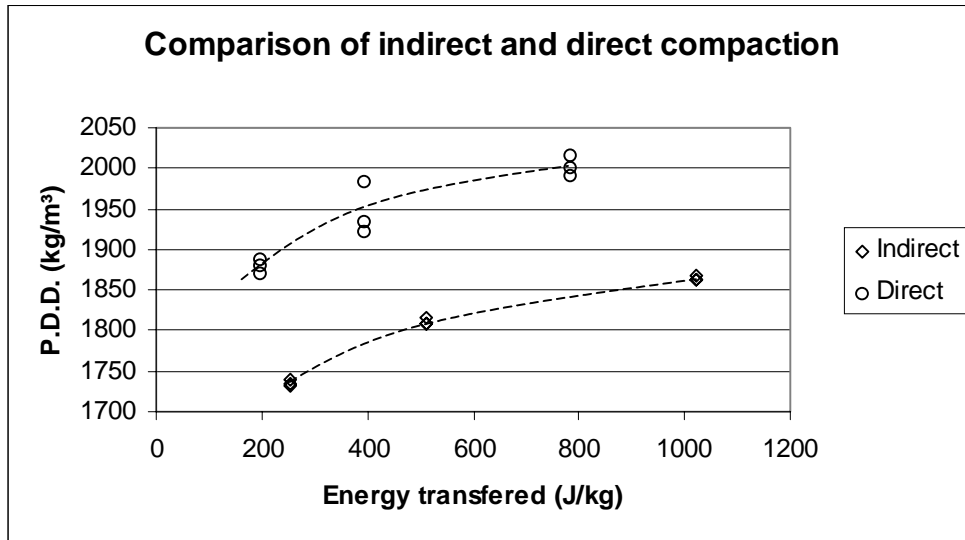
Figure 4.2 – Analysis of direct and indirect compaction
