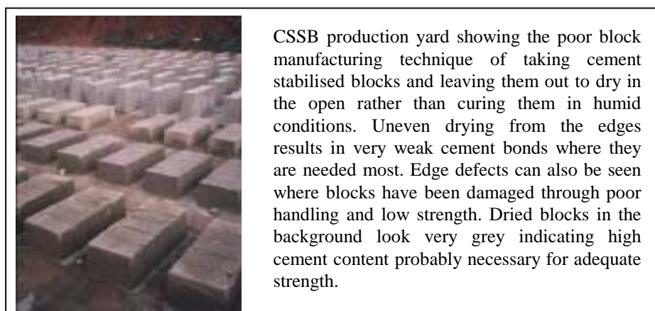
Figure 2.14 – CSSB production yard showing poor curing practice
