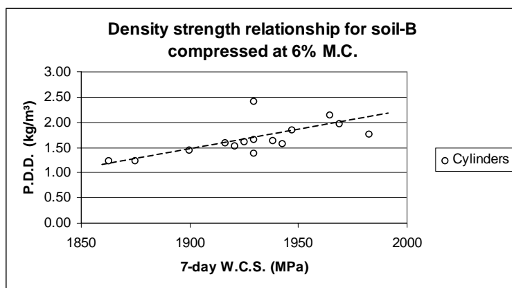
Figure 3.7 – Strength density relationship for soil-B at 6% M.C.
