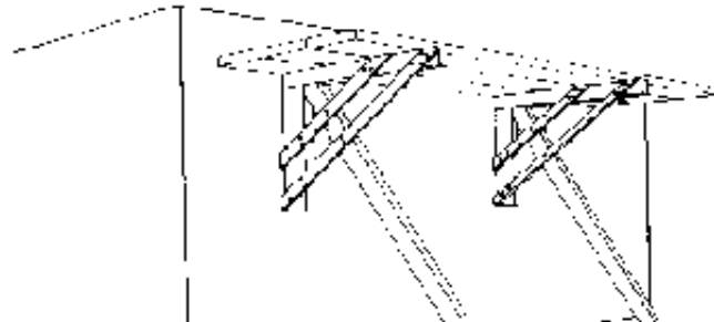
Scaffold built during wall construction
