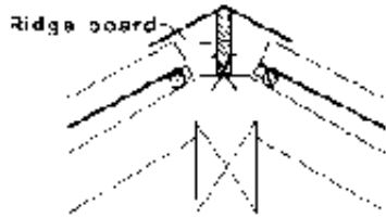
Fixing on ridgeboard by hooks
