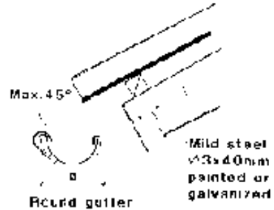
Round gutter
