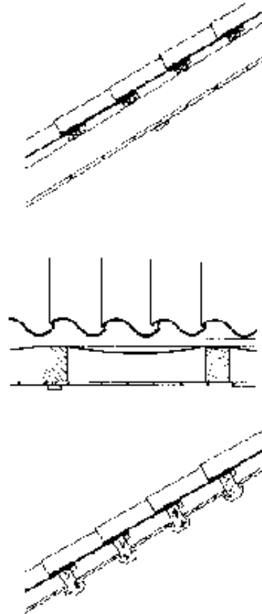
Types of double leaf roofing
