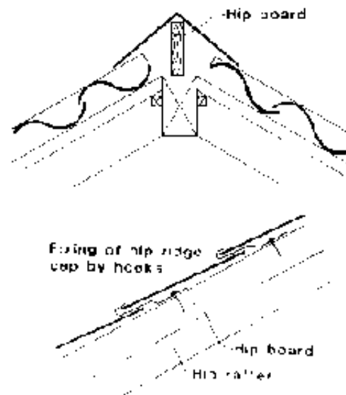
Fixing of the hipped ridge cap
