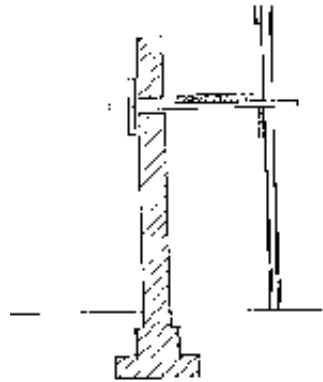
Scaffold built during wall construction
