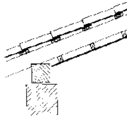
Double leaf roofing
