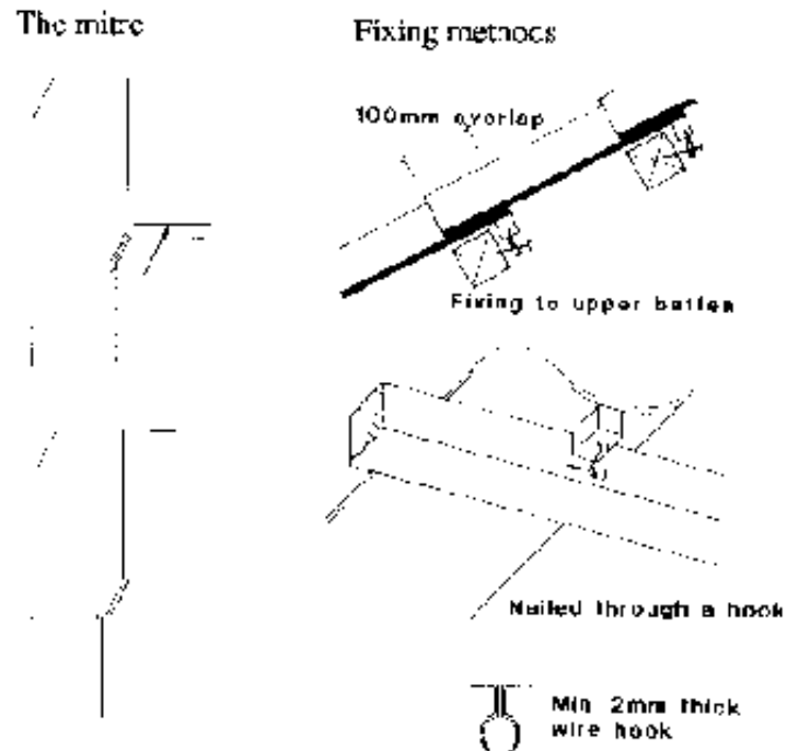
The mitre; Fixing methods
