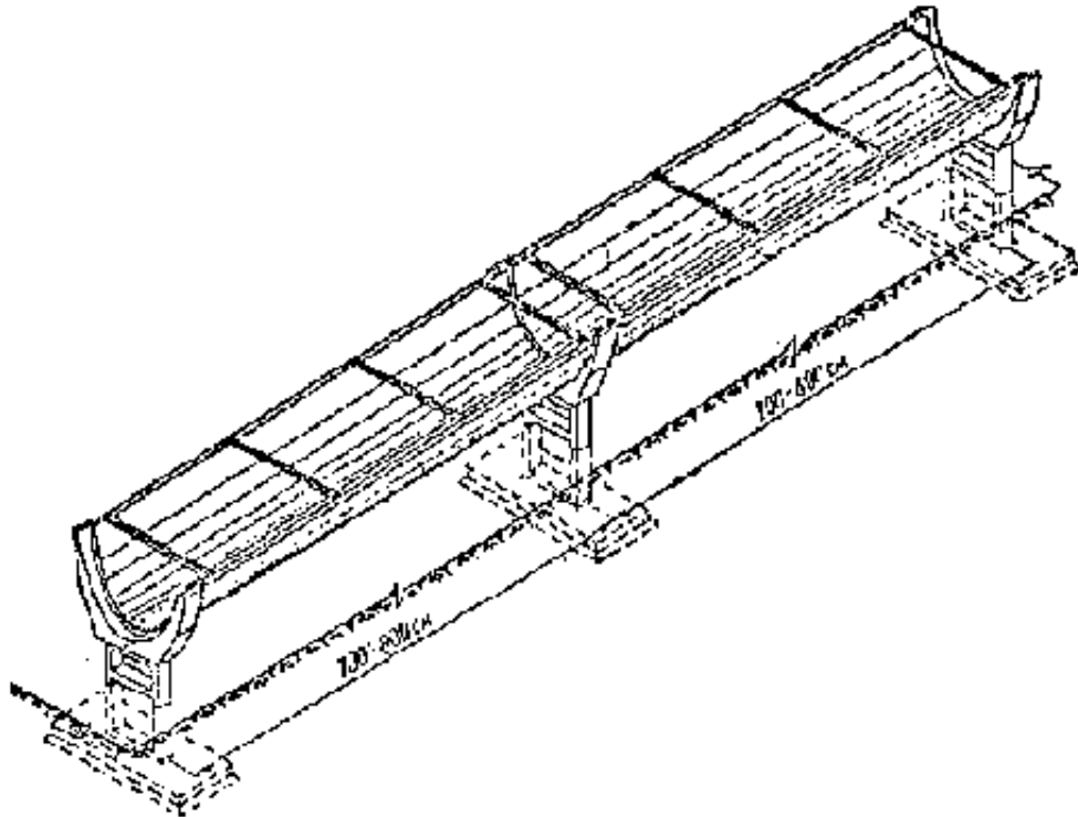
FIGURE 1: Water-conveying troughs, 20 mm thick, are mass-produced in precast ferrocement units in the USSR (Drawn from diagram in Kowalski, T.G. "Ferrocement in Hong Kong." Far East Builder. July 1971, p.29.)
