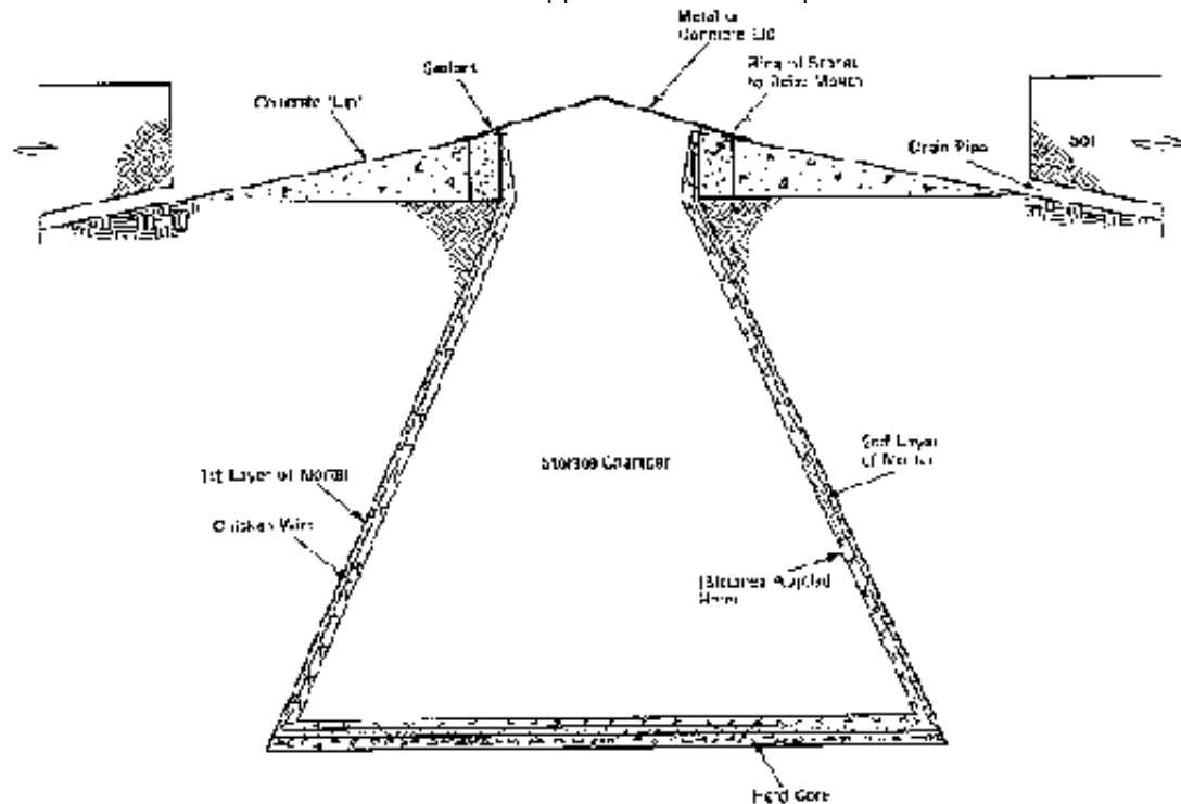
Figure C-3. Cross-section of ferrocement underground storage pit
