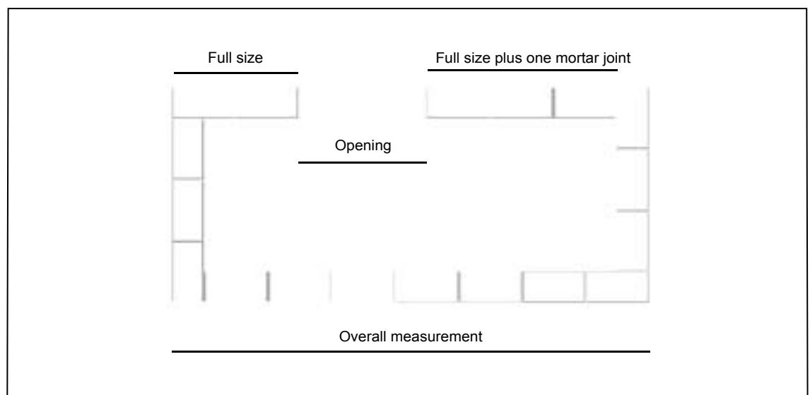
Scheme of different types of measurement for a ground floor plan shown as an example
