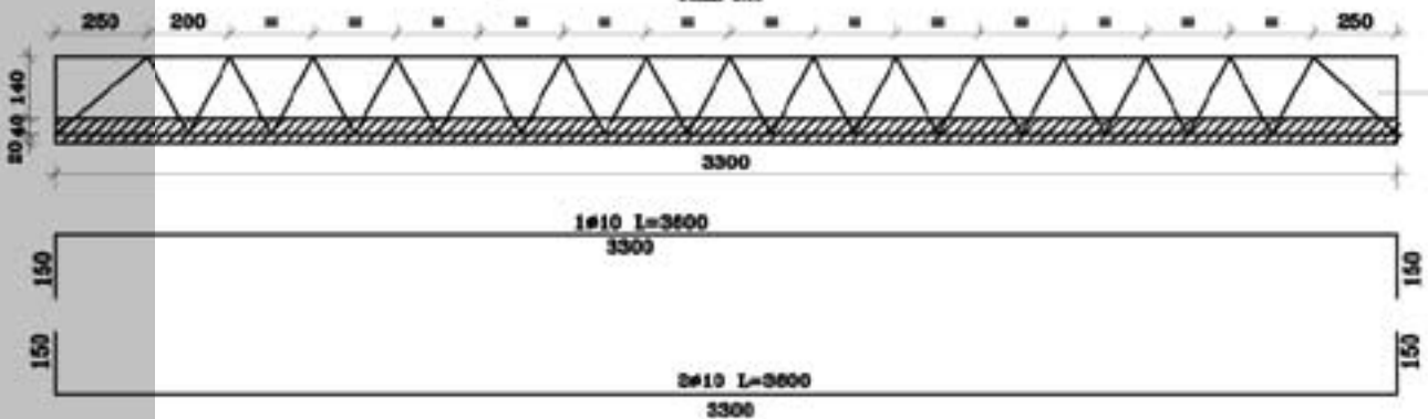
PRECAST BEAM -1 SCALE 1:10
