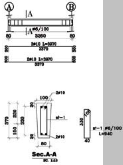
FFB-1 First floor beam A-B on axis 1,3,4 & 5
