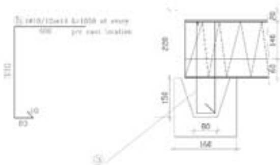
DETAIL A: Additional re-bar at edge
