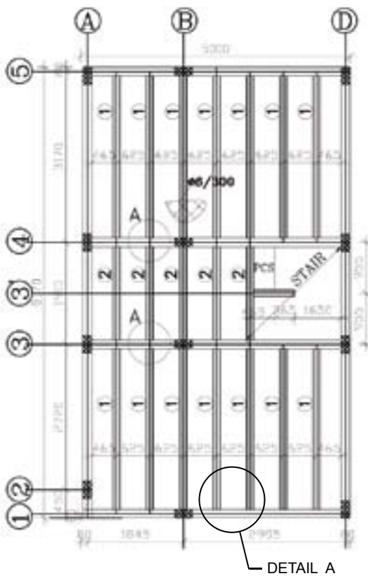
FIG-7s typical pre-cast beam layout
