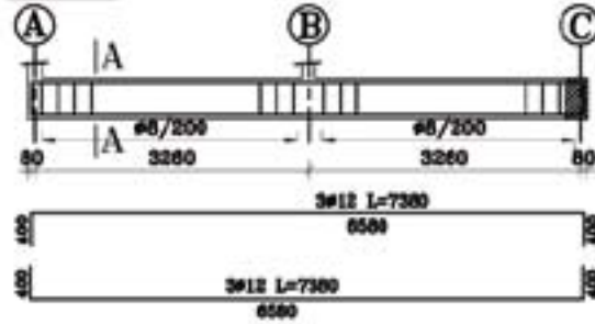
MB-1 Mat beam A-B-C on axis 1
