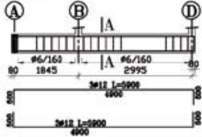
MB-1 Mat beam A-B-D on axis 1
