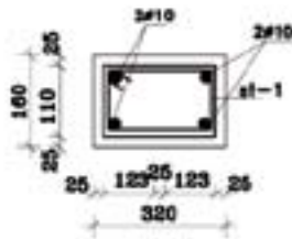
SEC.A-A Scale 1:10
