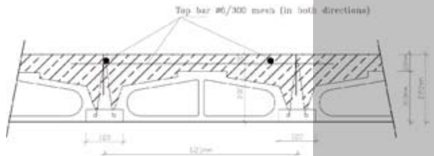
FIG-1s section of slab at final condition
