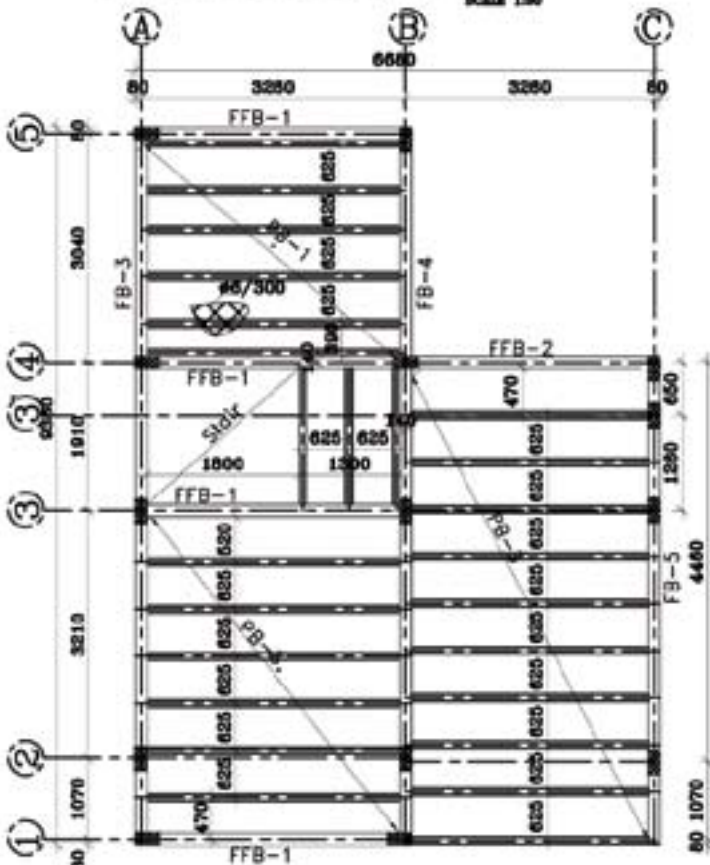
FFB-1 First floor beam A-B on axis 1,3,4 & 5
