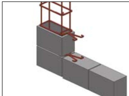
Connection inbetween column and wall
