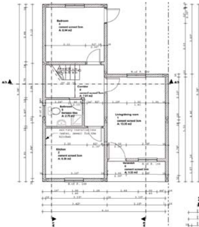
GROUND FLOOR, SCALE 1 : 100
