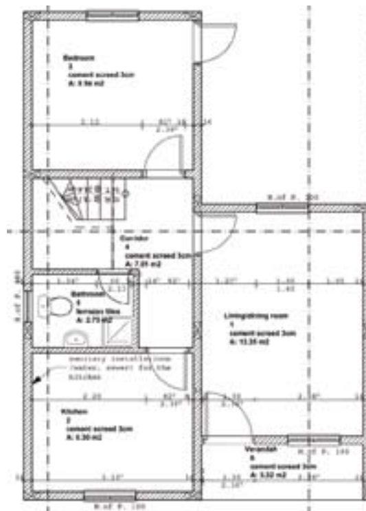
Building plan for the model
