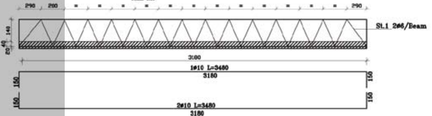
PRECAST BEAM -1 (1894pcs)
