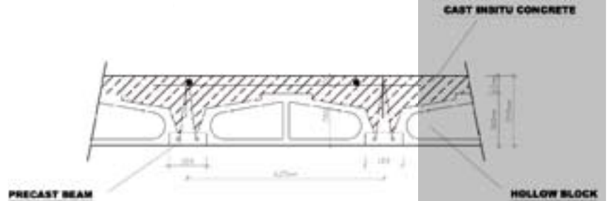
Typical Slab Section
