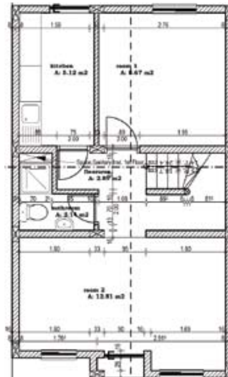
Building plan for the model
