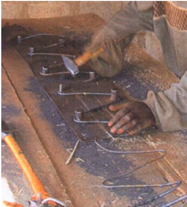
Forming the stirrup
