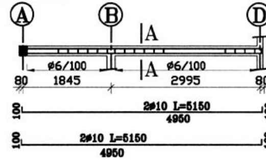
RB-1 Roof beam A-B-D on axis 1
