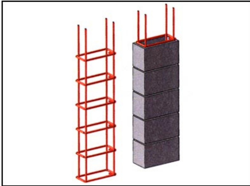
Column HCB with reinforcement
