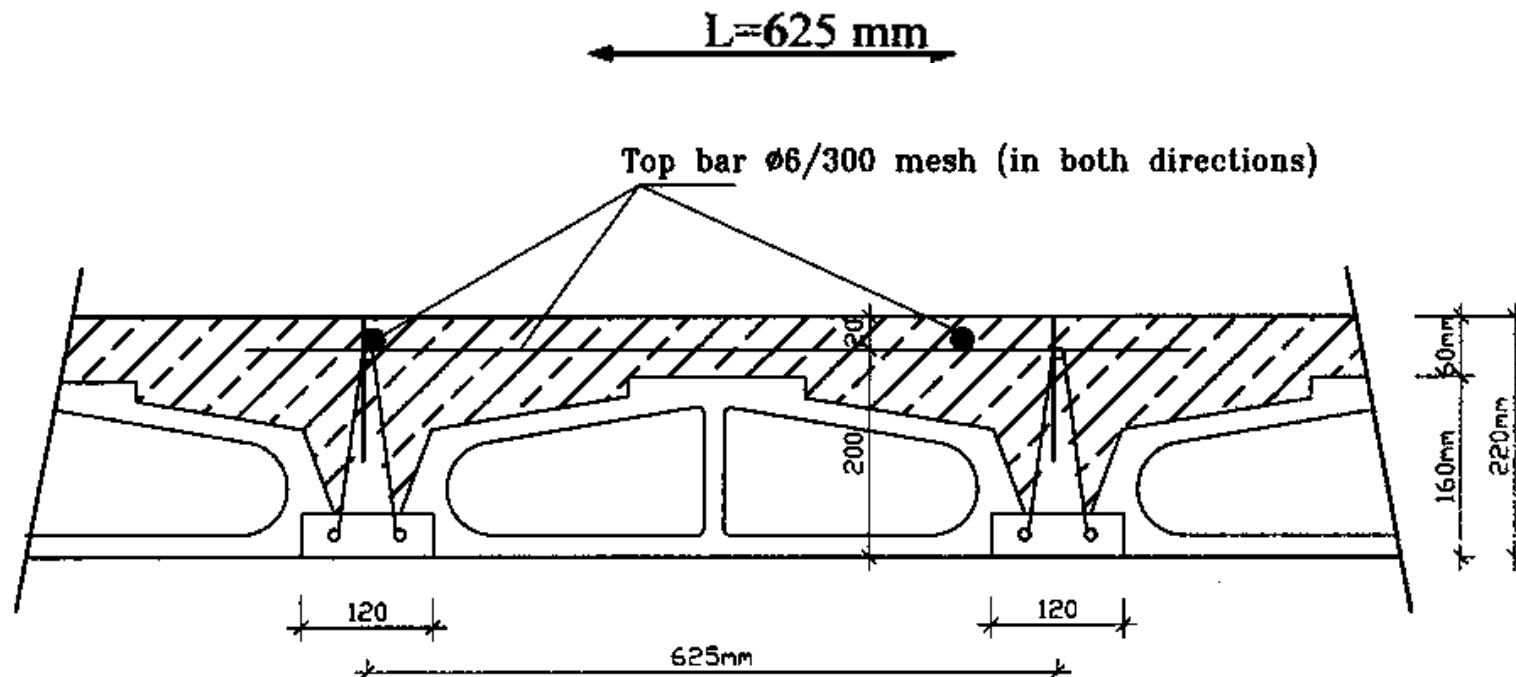
FIG-1s section of slab at final condition
