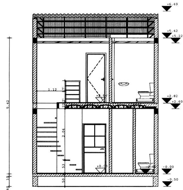
SECTION A/2, SCALE 1: 100 0
