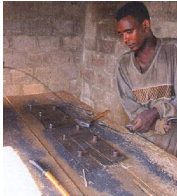
Removing a finished segment
