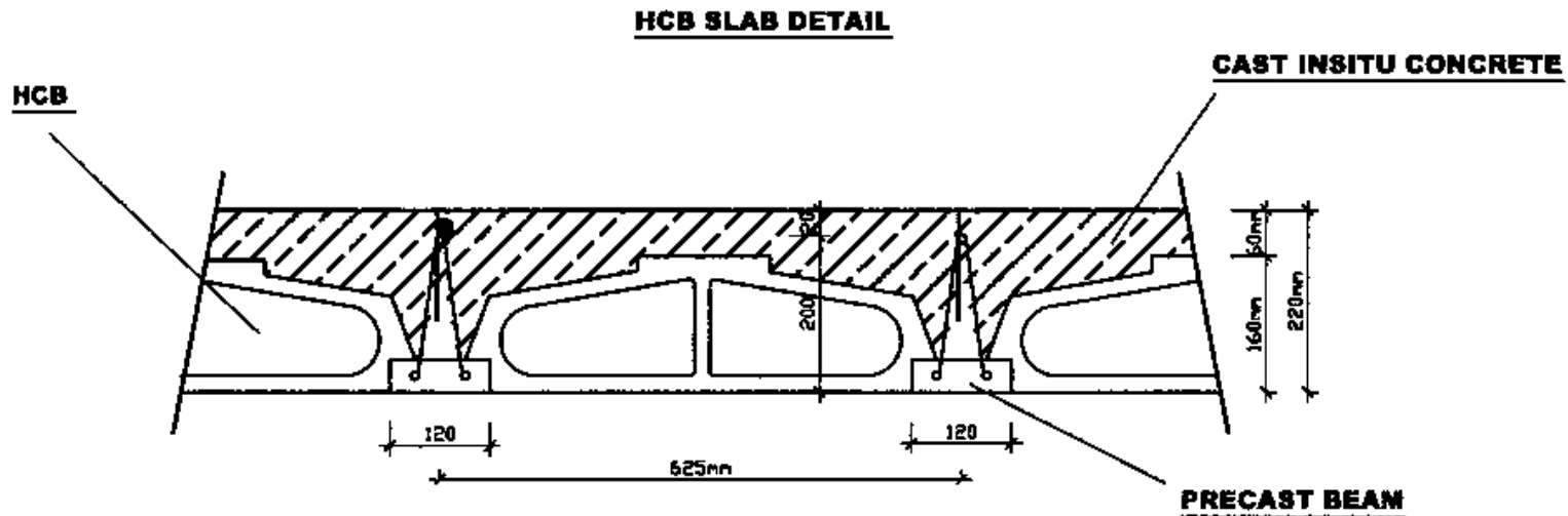
Fig-4s section of slab at final condition
