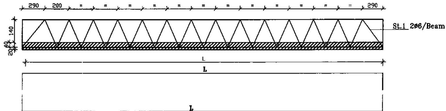
FIG 5s typical longitudinal section of precast beam
