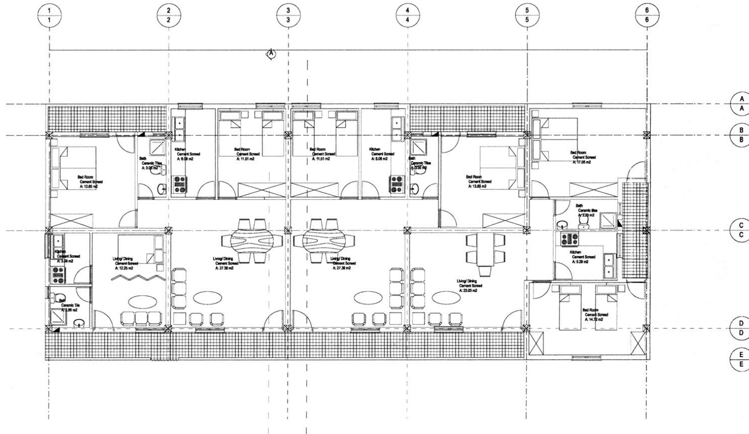
Building plan for the model
