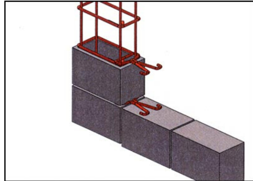
Connection inbetween column and wall
