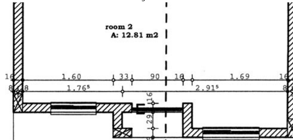
Building plan for the model
