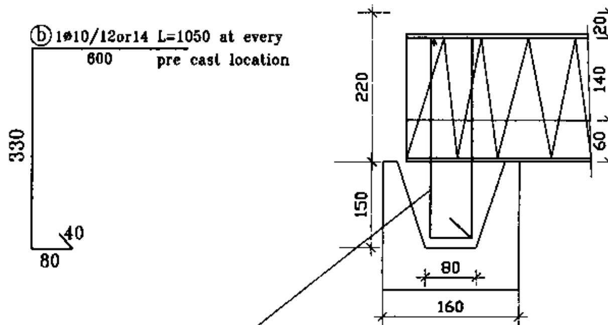
DETAIL A: Additional re-bar at edge
