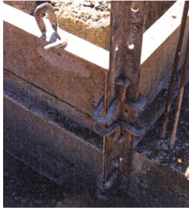
The edge of a formwork-assembly for foundation
