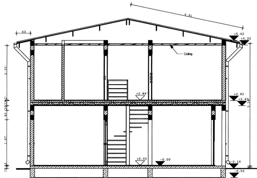
SECTION A/3, SCALE 1: 100
