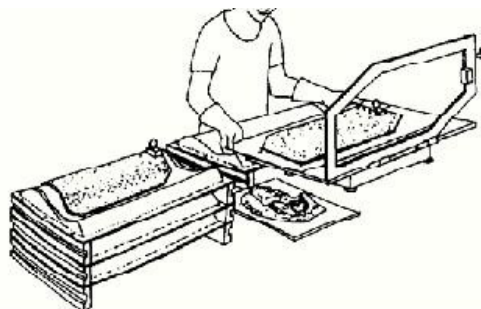
Figure 5: Pull polythene sheet with wet pantile over setting mould
