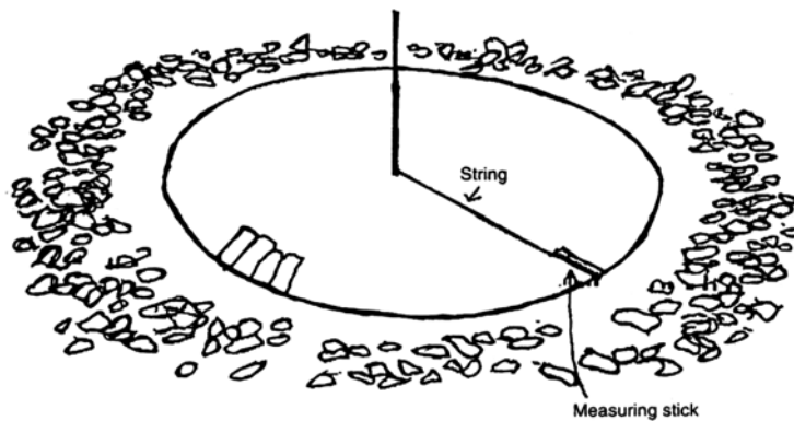
Figure 5: Only one circle is needed for a single skin wall
