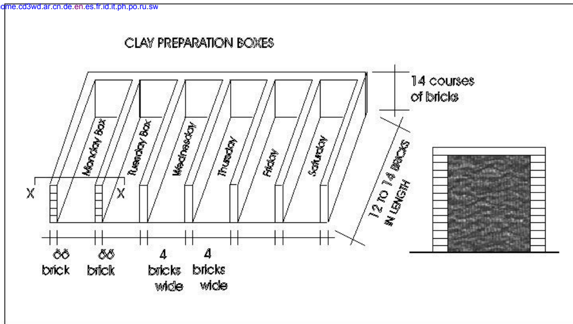
Fig. 5: One preparation box for each day - clay content for approximately 1000 bricks
