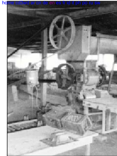
Fig. 9: Preparation plant suitable for clay without stones and roots
