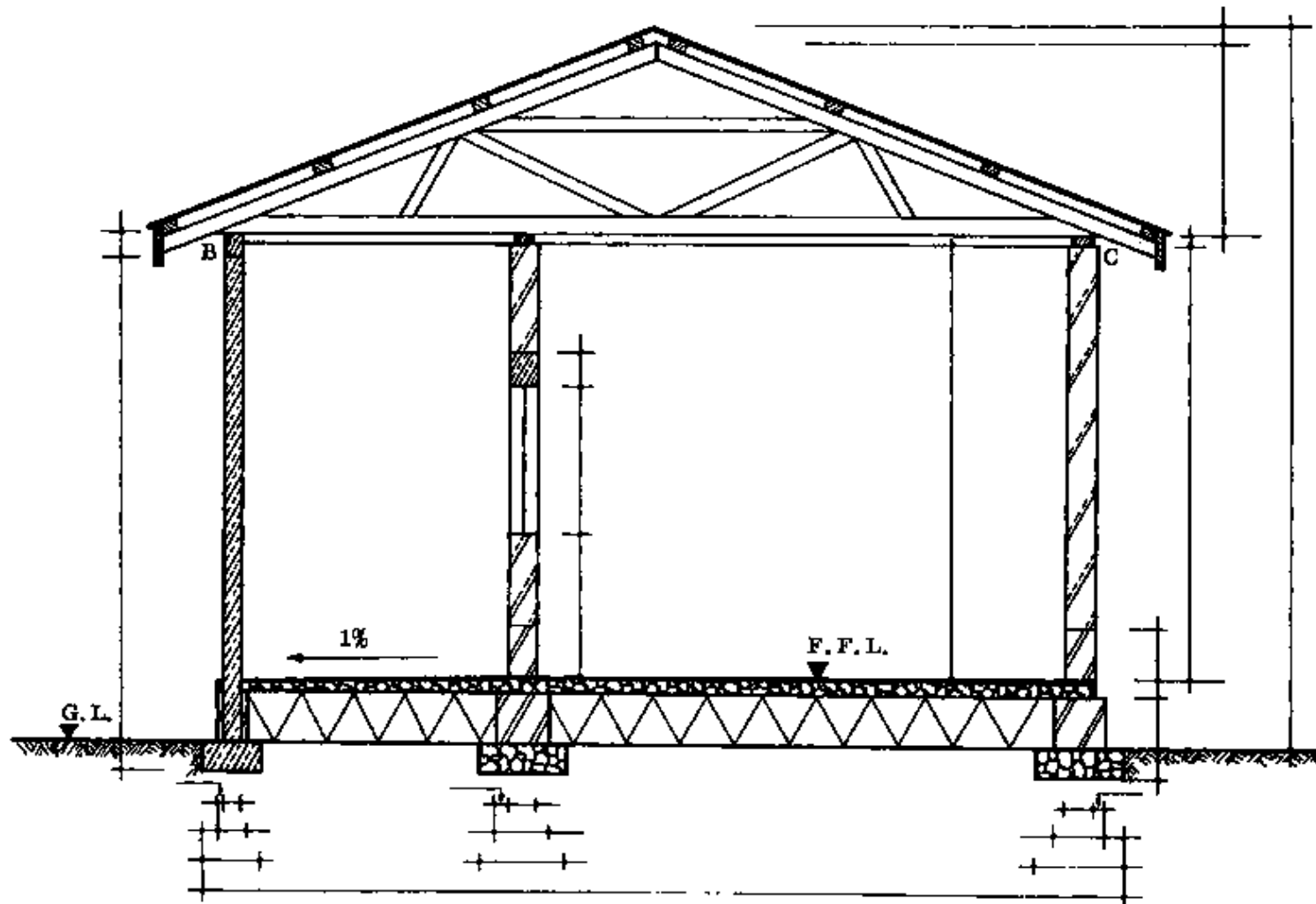
BUILDING WITH VERANDAH
