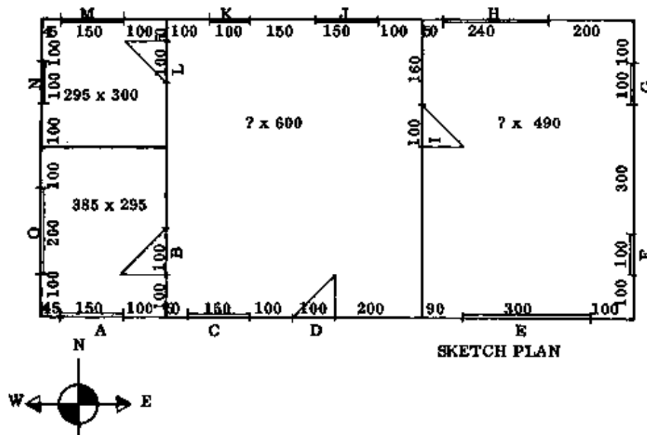
SKETCH PLAN
