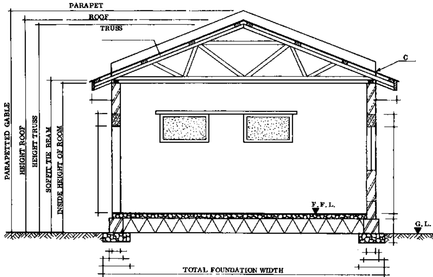
PARAPETTED GABLE ROOF
