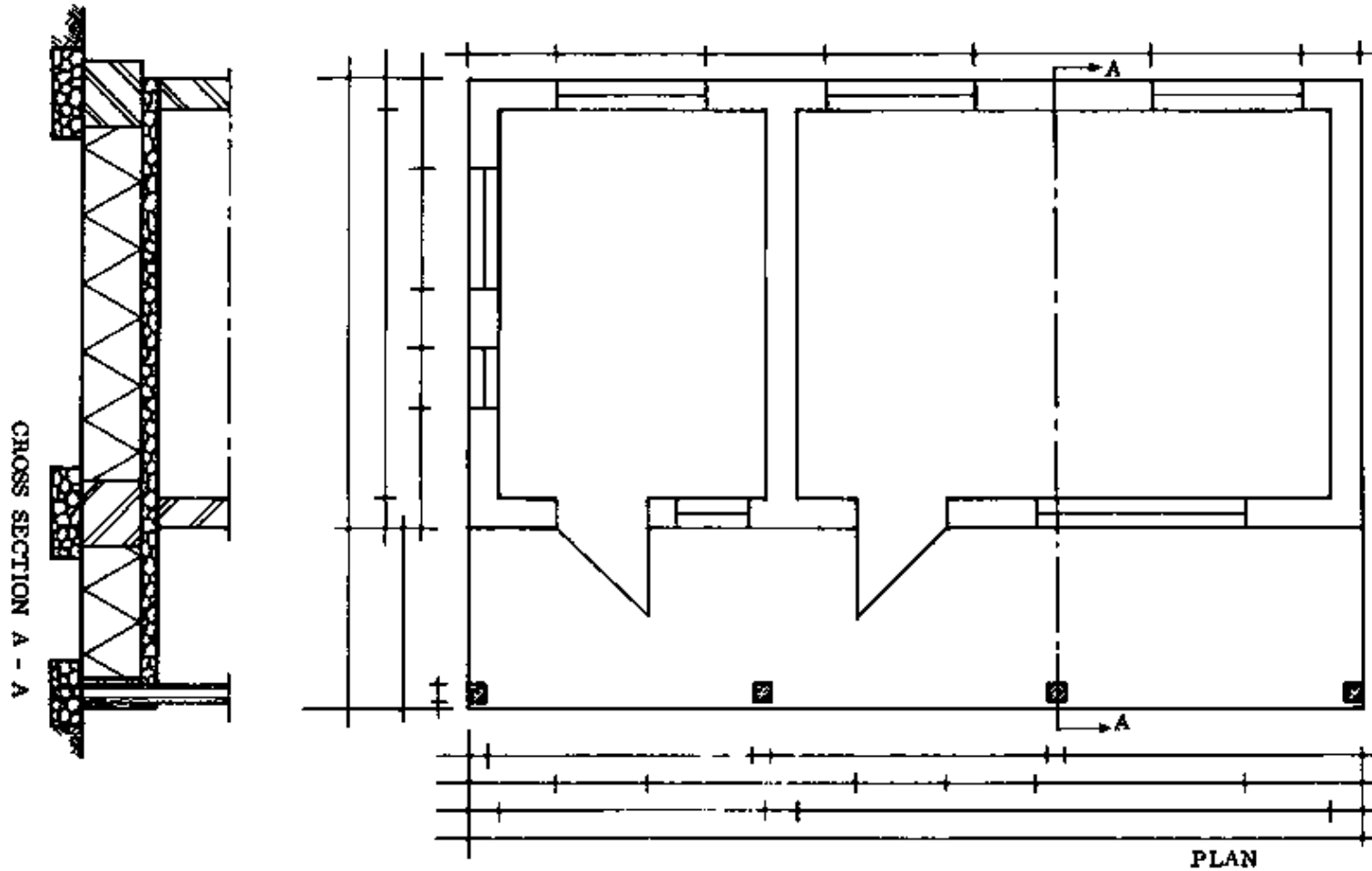
BUILDING WITH VERANDAH
