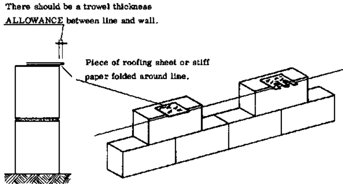
TINGLE PLATE
