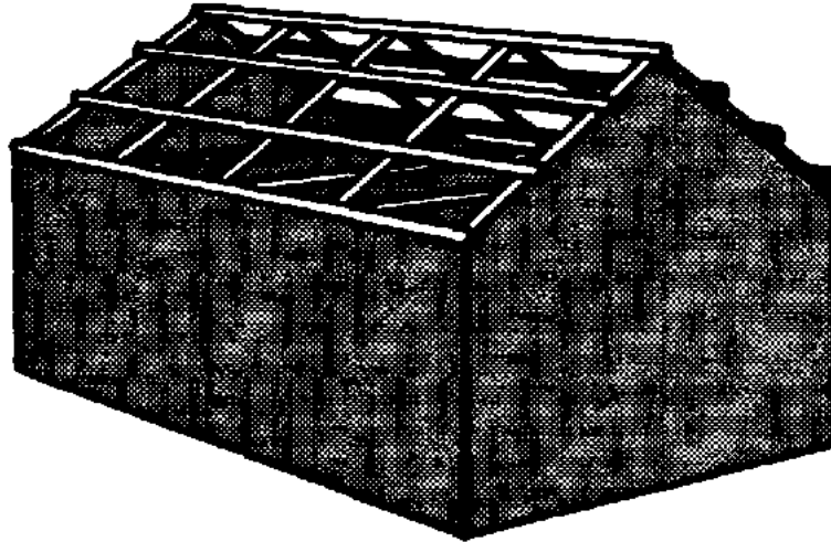
Gable roof: with purlins attached to trusses, and using end walls as truss supports
