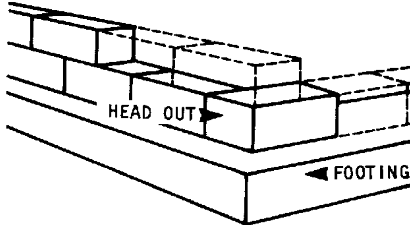
Staggered bond
