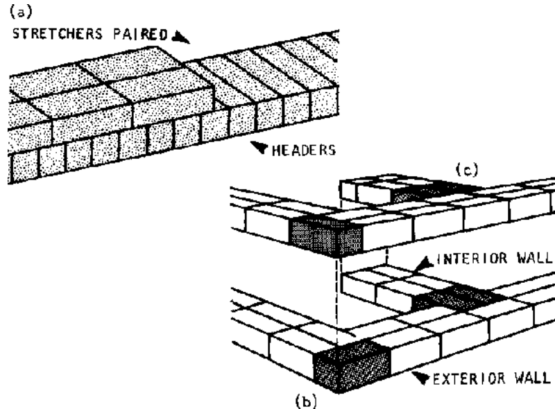
Double brick walls
