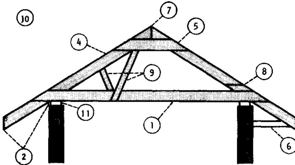
Roofs and trusses
