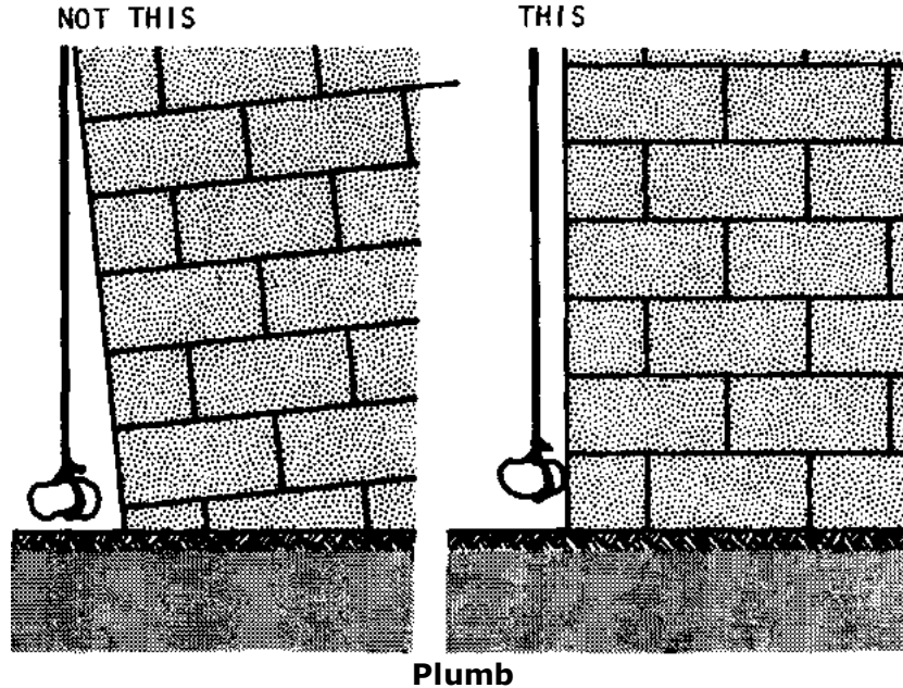
Plumb
