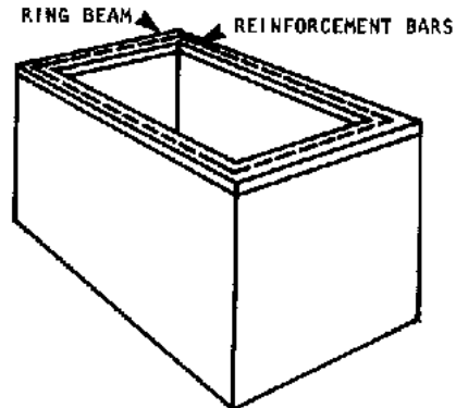
Ring beams
