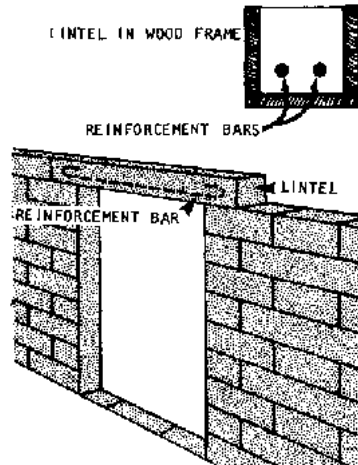
Lintels
