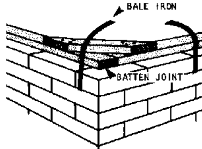
Wall plates
