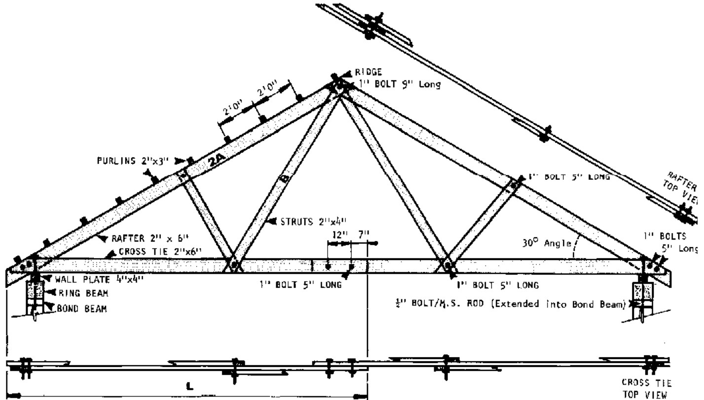
Construction details for truss on building 6 - 9.6 meters wide
