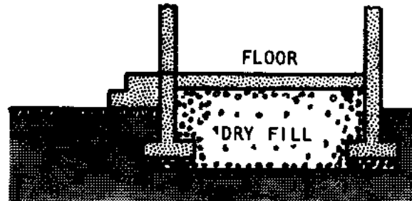
CORRECT: Raised to Prevent Flooding Keeping the floor dry
