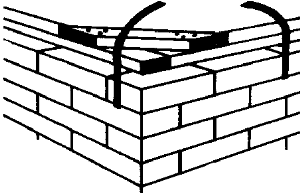
Batten joint with bale iron straps
