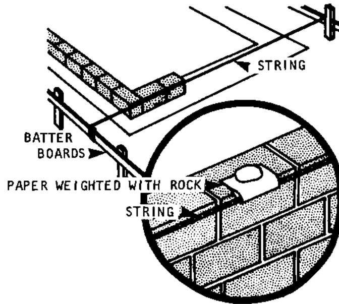
Paper weighted with rock
