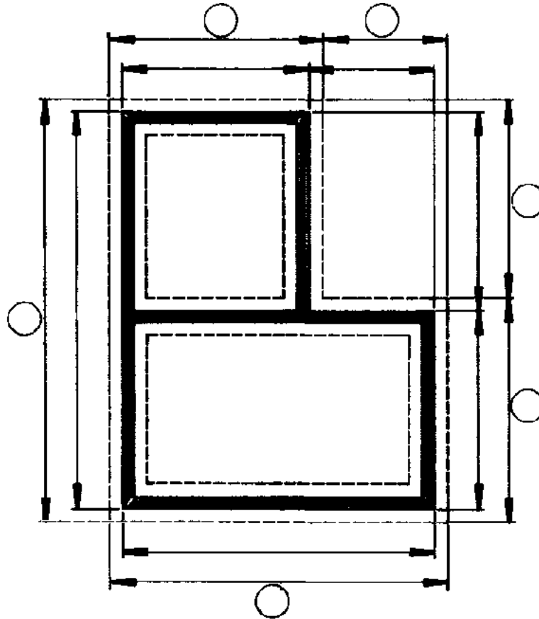
Complet foundation plans
