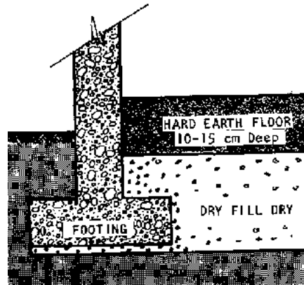
Concrete floor
