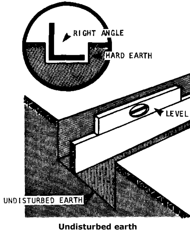
Undisturbed earth
