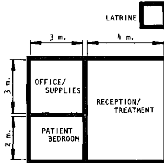
Plan for a small health station
