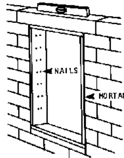
The sill
