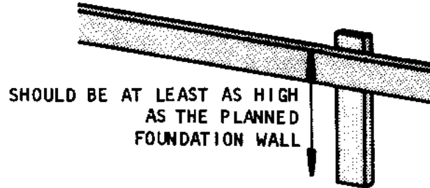
Placing batter boards
