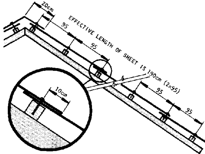
Effective length of sheet
