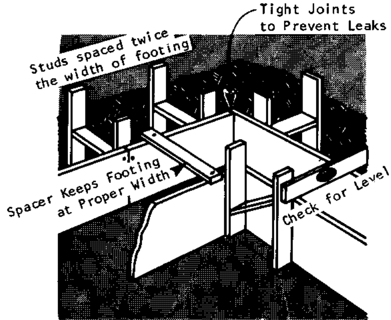
Formwork for footings
