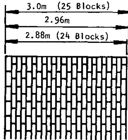
Wall height and length
