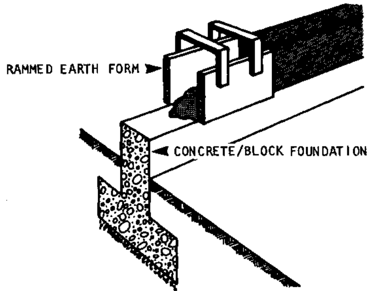
Rammed earth form
