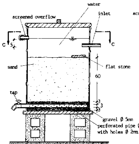
CROSS-SECTION A-A
