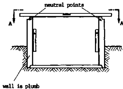
CROSS-SECTION C-C
