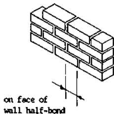
Half-Brick Wall
