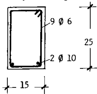
CROSS-SECTION B-B (1:10)
