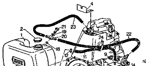
1. Exploded Diagram - Side-View (Part of Diaphragm Pump)
