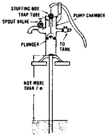
Force Pump Suction Type
