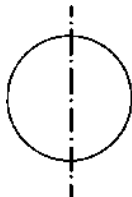
Symmetry of Circle
