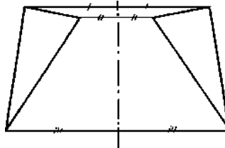
Symmetry of 2 Triangles
