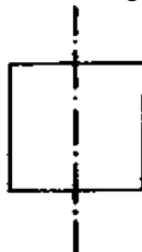
Symmetry of Square
