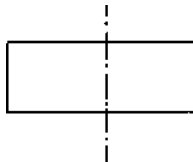
Symmetry of Rectangle
