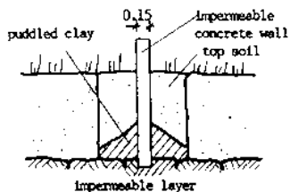
CROSS-SECTION B-B: ANTI-SEEPAGE WALL
