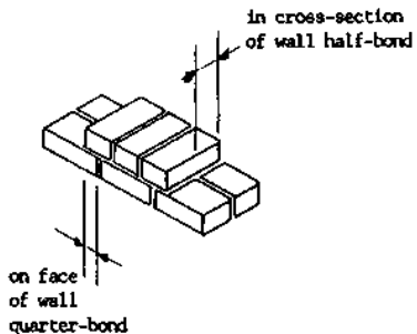
One-Brick Wall
