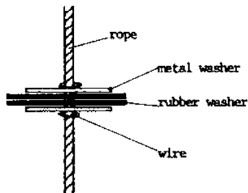
DETAIL: ROPE AND WASHER
