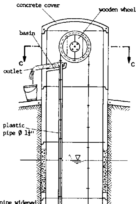
CROSS-SECTION A-A
