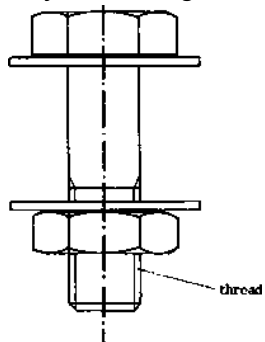
SIDE-VIEW A-A in different way
