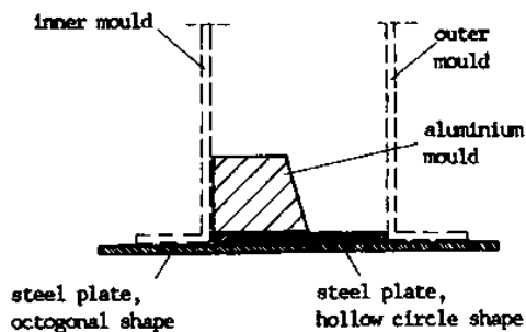
Cross-section A-A through base plate
