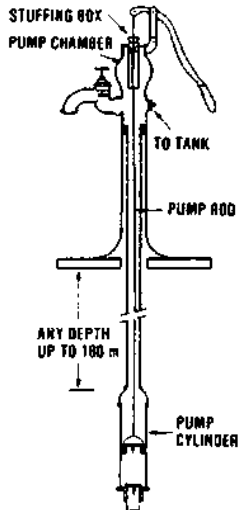
Force Pump with Cylinder
