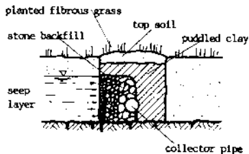
CROSS-SECTION A-A: INFILTRATION TRENCH
