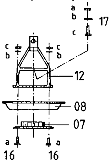
1. Exploded Diagram - Side-View (Part of Diaphragm Pump)
