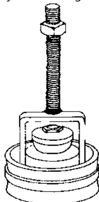
ISOMETRIC VIEW
