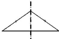
Symmetry of Equilateral Triangle
