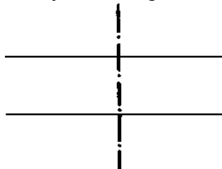
Symmetry of 2 Parallel Lines
