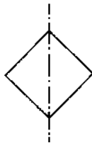
Symmetry of Square
