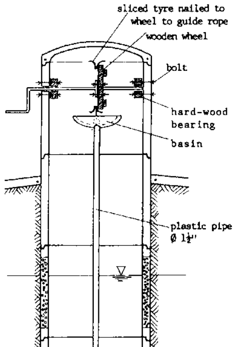
CROSS-SECTION B-B
