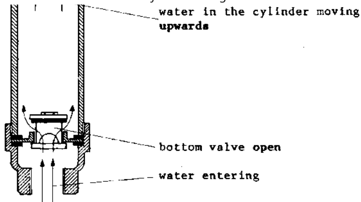
Schematic Illustration; some details left for sake of clarity; valves in side-view.
