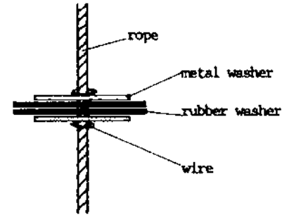
DETAIL: ROPE AND WASHER
