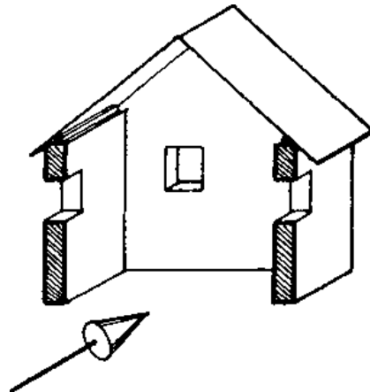
ISOMETRIC VIEW of the remaining part; this is not called "cross-section"!!!
