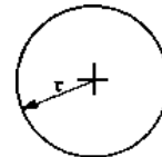
Radius and centre
