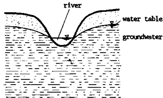
Effluent Stream: gains water from the aquifer (the sane stream may have influent and effluent sections)
