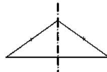
Symmetry of Equilateral Triangle
