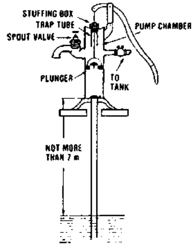
Force Pump Suction Type
