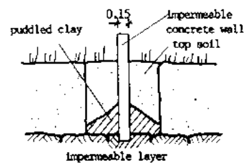
CROSS-SECTION B-B: ANTI-SEEPAGE WALL
