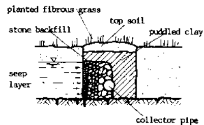
CROSS-SECTION A-A: INFILTRATION TRENCH
