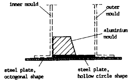
Cross-section A-A through base plate
