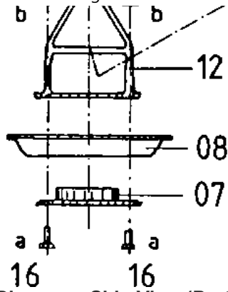
1. Exploded Diagram - Side-View (Part of Diaphragm Pump)
