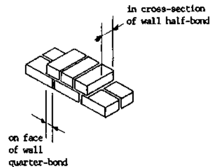
One-Brick Wall
