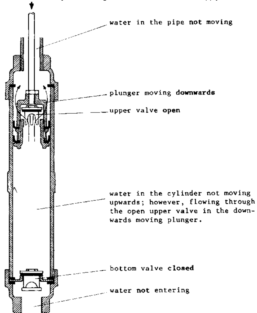
Schematic Illustration: sane details left for sake of clarity; valves in side-view.
