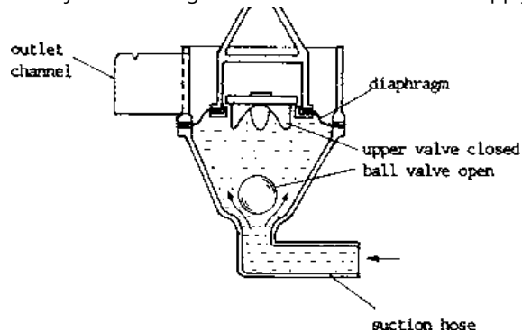
Schematic Illustration Diaphragm assembly turned by 90° for clarity; see also 8.24/22.
