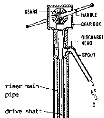
CROSS-SECTION
