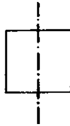
Symmetry of Square
