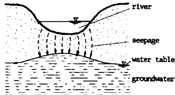
Stream only Flowing Periodically: dry during drought
