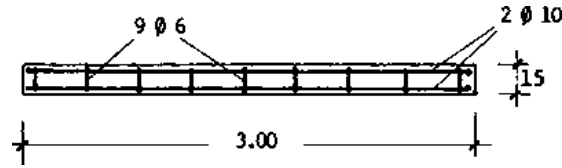
LAYOUT PLAN C-C (1:40)
