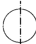
Symmetry of Circle
