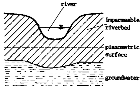
Stream Isolated Hydraulically: from an artesian aquifer below it
