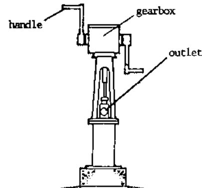
CUT-AWAY SIDE-VIEW
