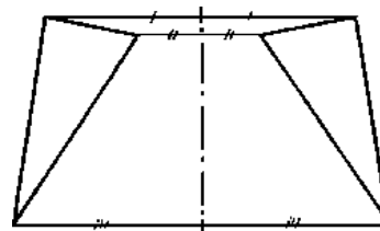
Symmetry of 2 Triangles
