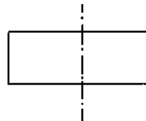
Symmetry of Rectangle
