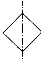
Symmetry of Square
