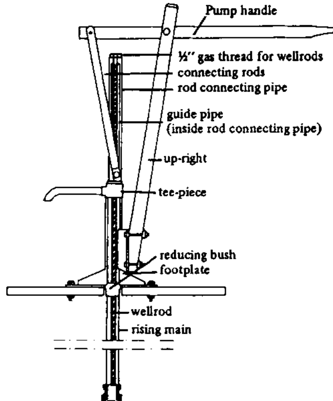
12. Piston Hand Pump with Uganda Type Handle with cylinder, riser main pipe, rod, outlet, and wooden handle; for deep wells.
