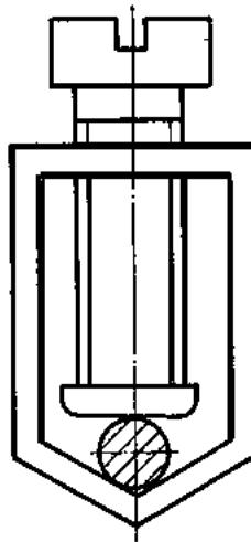
Figure 14 - Connection by means of connector block
