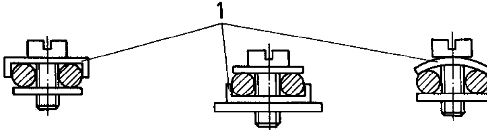
Figure 12 - Clamping saddle connections - 1 clamping saddle
