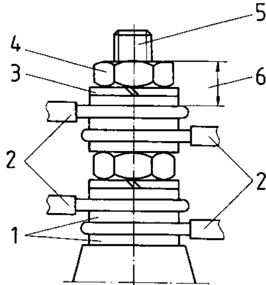
Figure 11 - Construction of a bolt joint with four aluminium conductors - 1 washer, 2 conductor, 3 lock washer, 4 nut, 5 bolt, 6 pressure piece
