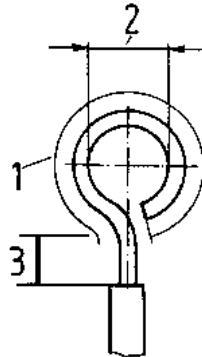
Figure 8 - Representation of a wire lug - 1 length to be stripped, 2 lug diameter, 3 distance from beginning of lug to conductor insulation
