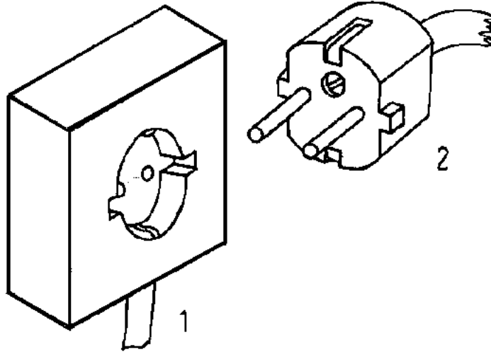
Figure 19 - Heavy-current plug-and-socket connector - 1 plug , 2 socket
