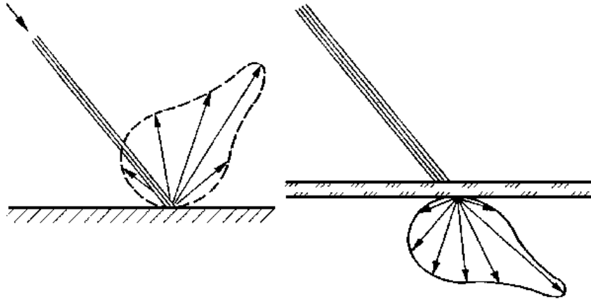
Figure 12. Mixed reflection, transmission
