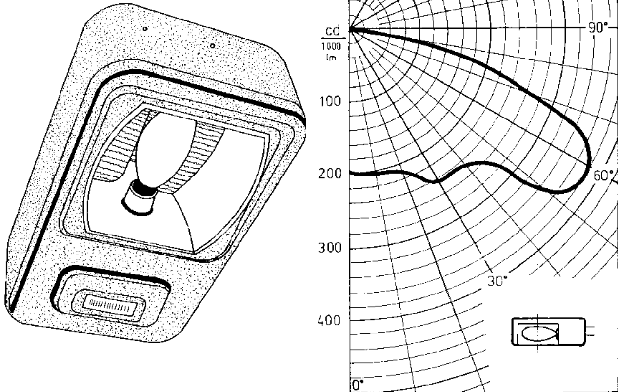
Figure 50. Brace-fixed lamp pole fitting with light distribution curve with a light output ratio of 0.73 (NA 400-01 sodium vapour lamp)
