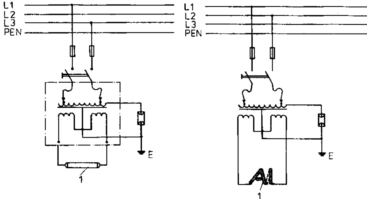
Figure 55. High-voltage fluorescent lamp circuits
