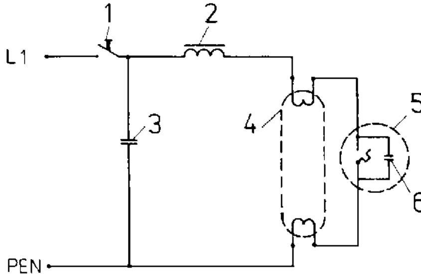
Figure 27. Separate switching of fluorescent lamps
