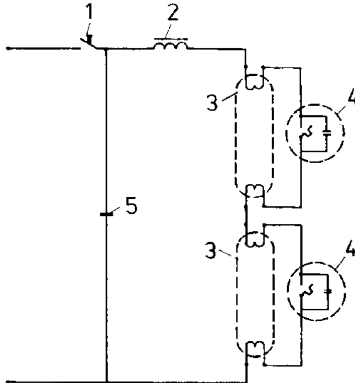
Figure 28. Tandem switching of fluorescent lamps
