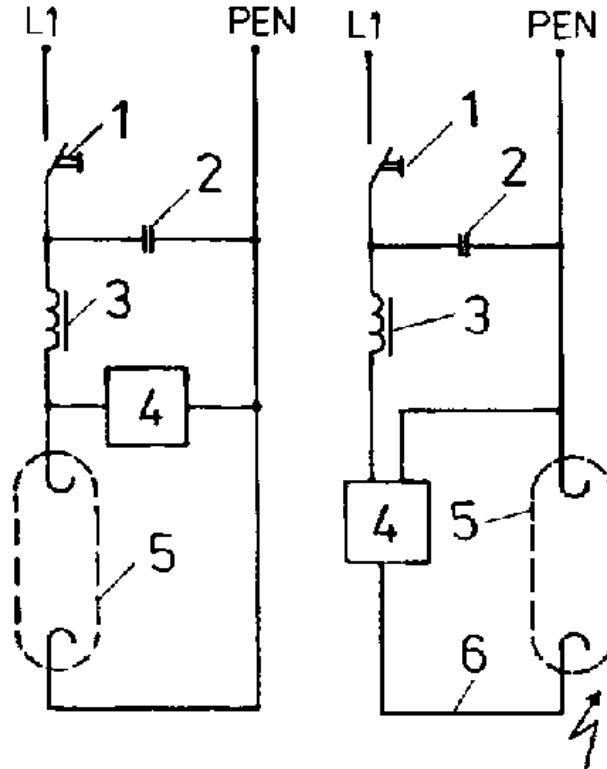
Figure 36. Circuit of high-pressure sodium vapour lamps
