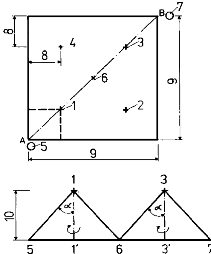
Figure 16. Dimensional sketch
