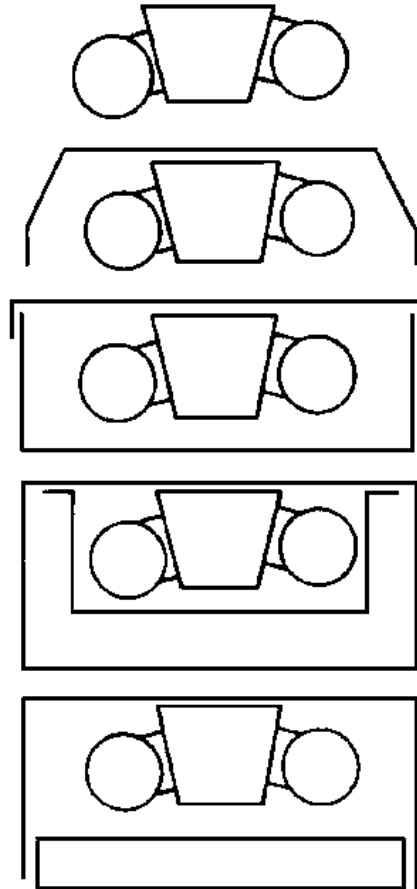
Figure 45. Combination fitting with various glare protection shields
