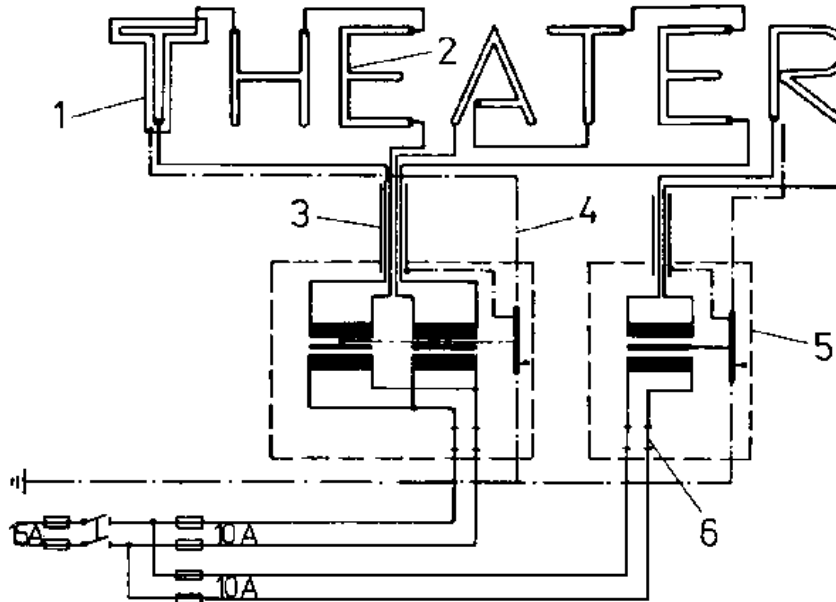
Figure 54. System structure of a fluorescent lamp installation
