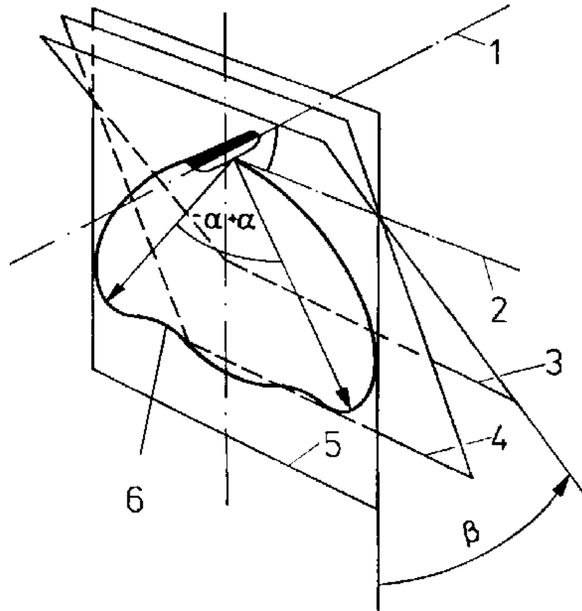
Figure 4. Light distribution curve (A plane)
