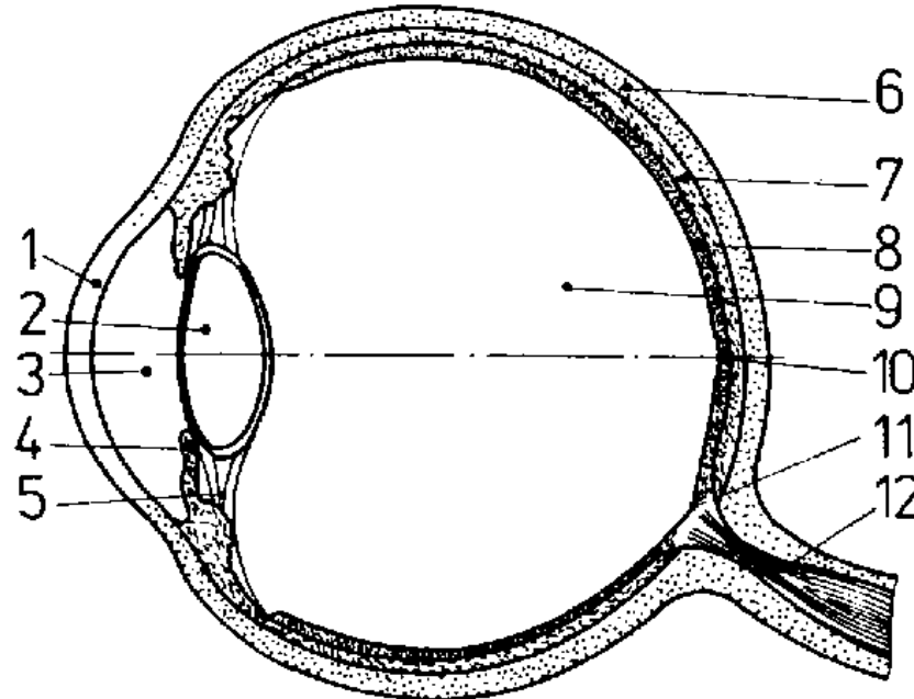
Figure 13. Horizontal section through the human eye
