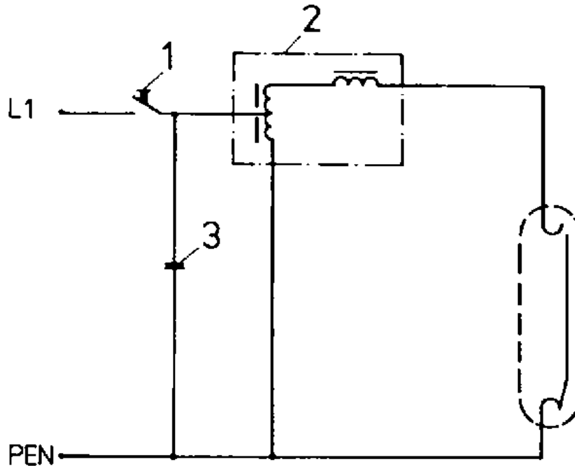
Figure 29. Rapid switching of fluorescent lamps
