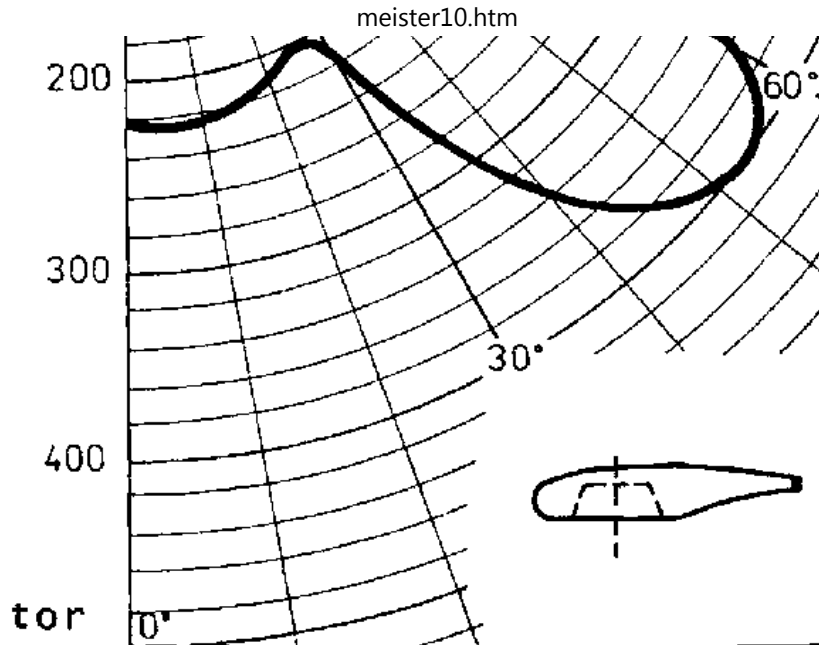
Figure 49. Brace-fixed lamp hole fitting with light distribution curve with a light output ratio of 0.76 (high-pressure mercury vapour lamp NF 400-01)
