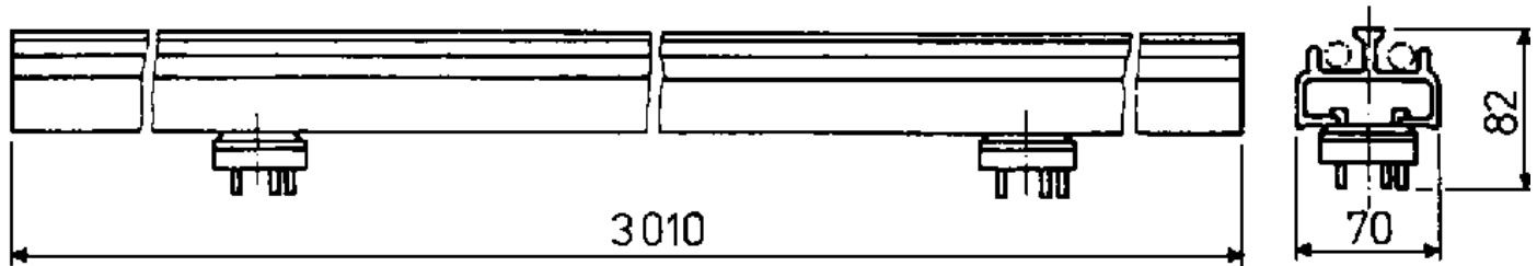
Figure 57. Carrier rails for fittings in row installation
