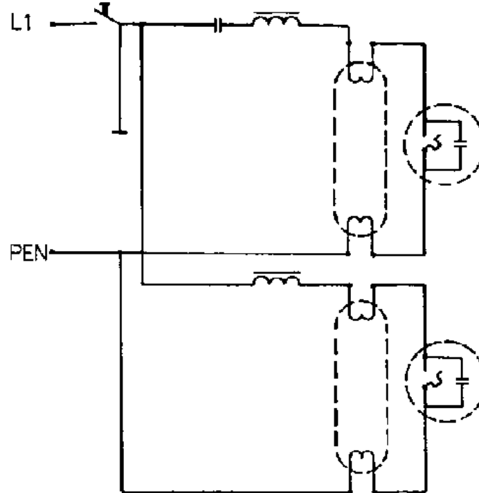
Figure 30. Dual lamp circuit of fluorescent lamps
