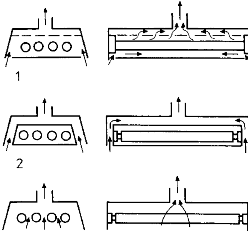
Figure 47. Air-handling fittings
