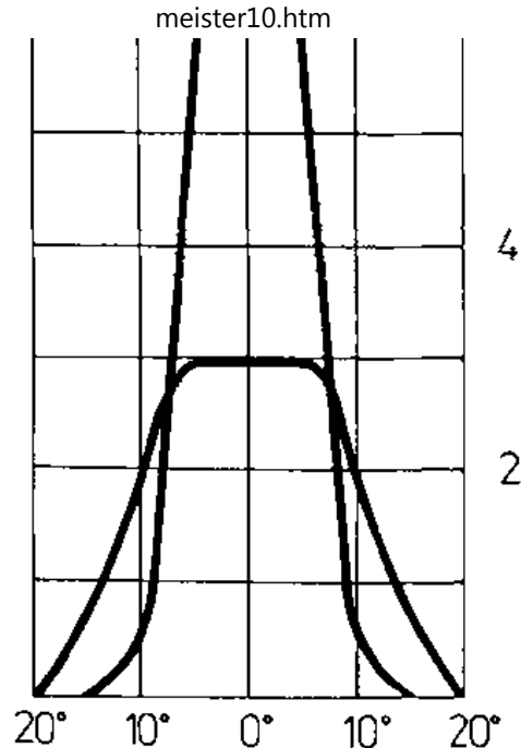
Figure 48. Narrow-angle lighting fitting for illuminating halls with light distribution curve with a light output ratio of 0.66 (halogen metal vapour lamp NC 2000-60)
