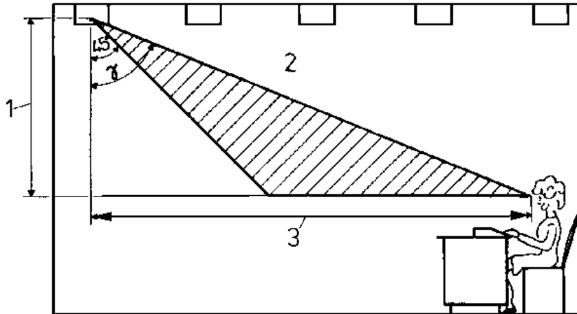
Figure 14. Radiation angle for glare evaluation
