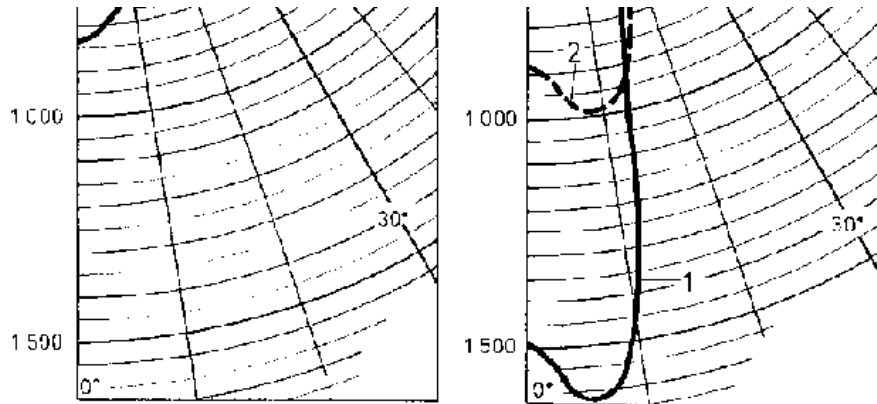
Figure 53. Mirror downlighter with light distribution curves (general service lamp 300/500 W curve around 0 degree)
