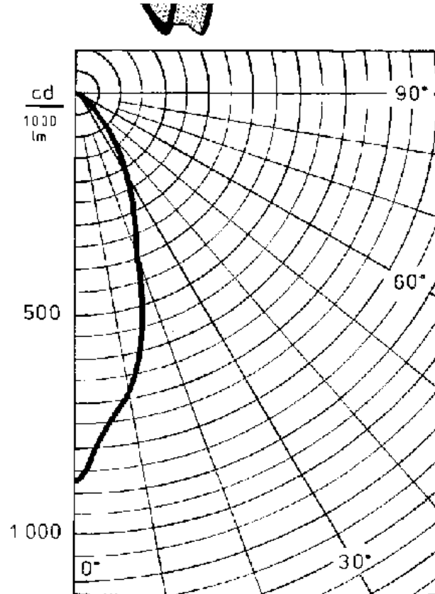
Figure 52. Industrial spot-light with light distribution curve (high-pressure mercury vapour lamp NF 400-01)
