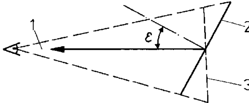
Figure 8. Representation of luminance
