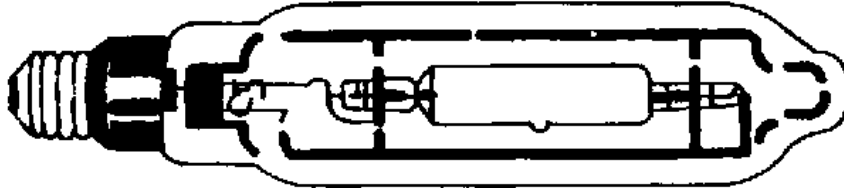
Figure 33. Halogen metal vapour lamp
